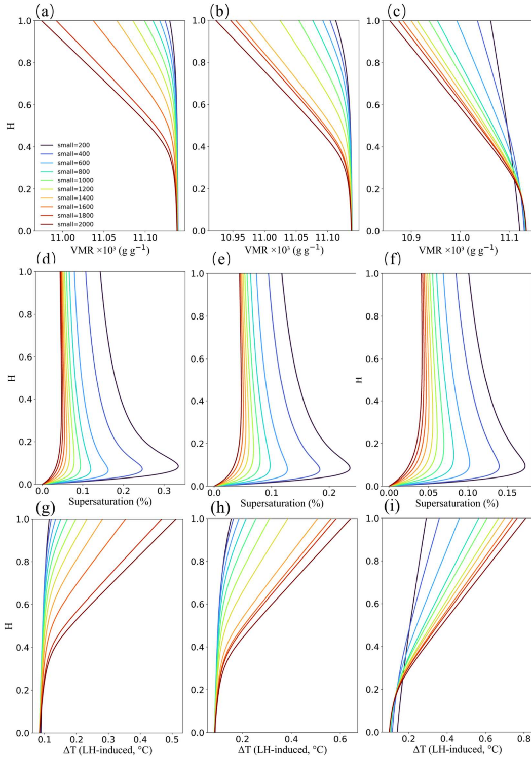
345 Figure.8 Vertical profiles of cloud water vapor mixing ratio (VMR) vapor content (a-c), supersaturation relative humidity (e-f), and condensation-induced environmental warming (g-i) under different aerosol concentrations. Colored curves represent different aerosol concentrations, and the vertical coordinate H denotes the normalized cloud height.
