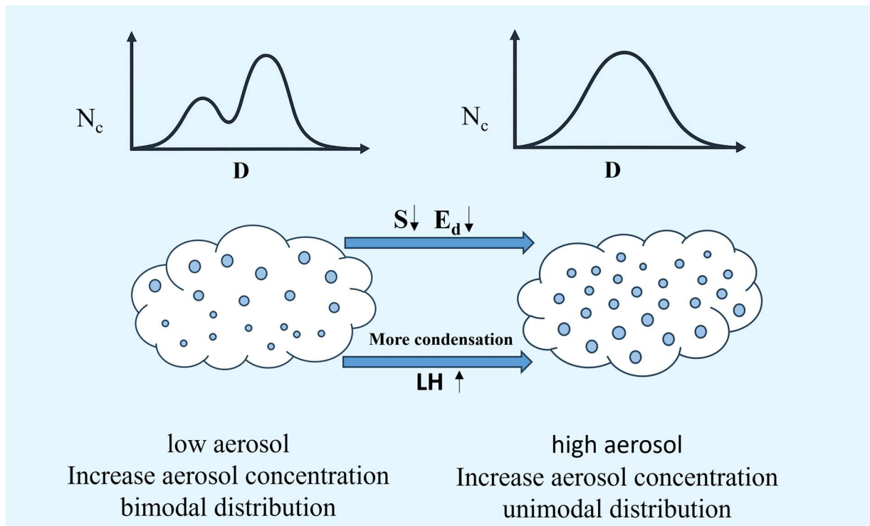
Figure. 28: Conceptual illustration of the effects of low and high subcloud aerosol concentrations on cloud droplet properties.
