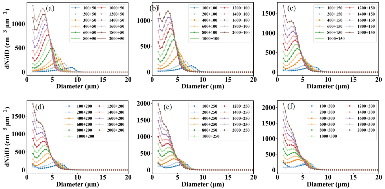
315 Figure.6 Cloud droplet size distributions under varying concentrations of small particles with fixed concentrations of large particles. The concentrations of large particles are (a) 50, (b) 100, (c) 150, (d) 200, (e) 250, and (f) 300 \text{cm}^{-3} . In the legend, the notation “x + y” denotes the concentrations of small particles (x) and large particles (y), respectively.
