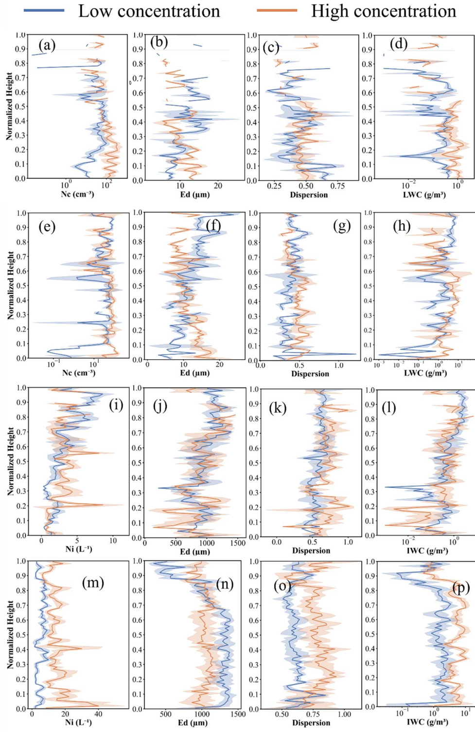
Figure 4 Vertical distributions of different cloud particle characteristics. (a–d) water cloud droplets, (e–h) mixed-phase clouds droplets, (i–l) ice crystals in mixed clouds, (m–p) ice crystals in ice clouds. For each cloud type, the panels from left to right represent number concentration, effective diameter, dispersion, and water content, respectively.
