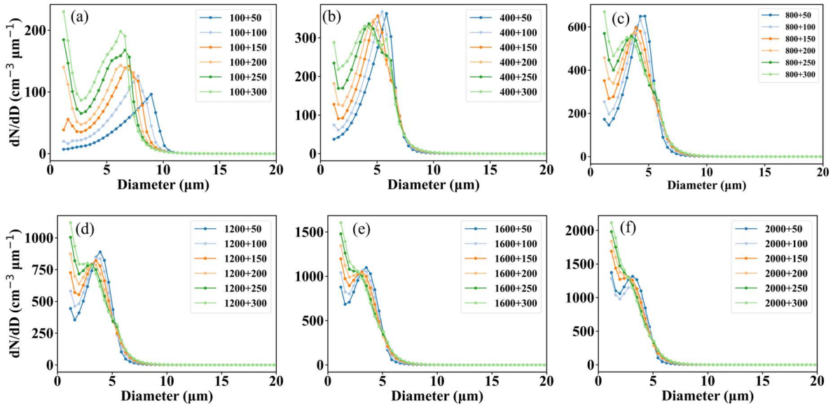
Figure.5 Cloud droplet size distributions under varying concentrations of large particles with fixed concentrations of small particles. The concentrations of small particles are (a) 100, (b) 400, (c) 800, (d) 1200, (e) 1600, and (f) 2000 \text{cm}^{-3} . In the legend, the notation “x + y” denotes the concentrations of small particles (x) and large particles (y), respectively.
