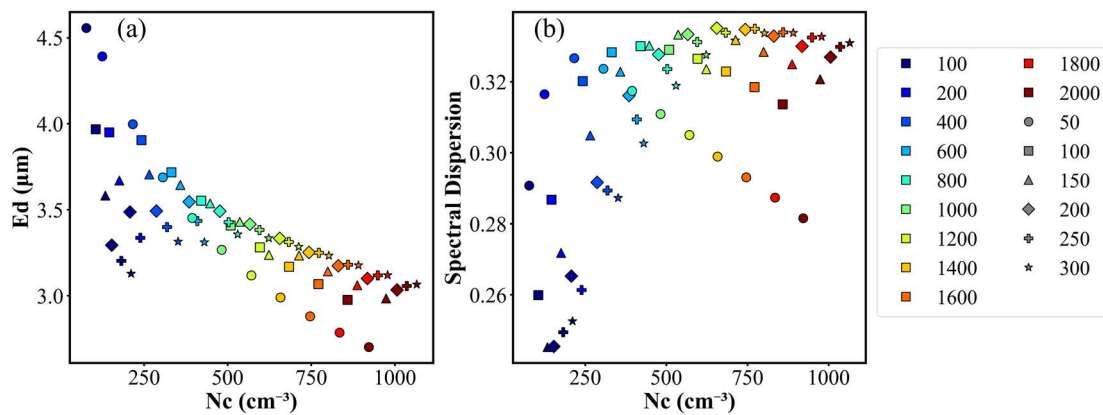
330 Figure 7. Scatter plot of the cloud droplet effective diameter ( E_d ), droplet spectral dispersion, and droplet number concentration ( N_c ) at cloud base. The marker color represents the concentration of small particles, and the marker shape represents the concentration of large particles.
