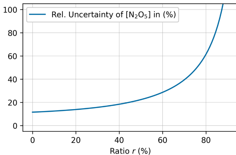
45 Figure S3: The dependence of the relative uncertainty of our true, ambient [N 2 O 5 ] measurements on r which describes the ratio of NO 3 over the sum of NO 3 and N 2 O 5 in the heated cavity and can be approximated by the equilibrium constant with an additional ambient NO 2 measurement (see main text). The values are calculated using the relative uncertainties in Table 2 and the equations presented in Section 3.6.
