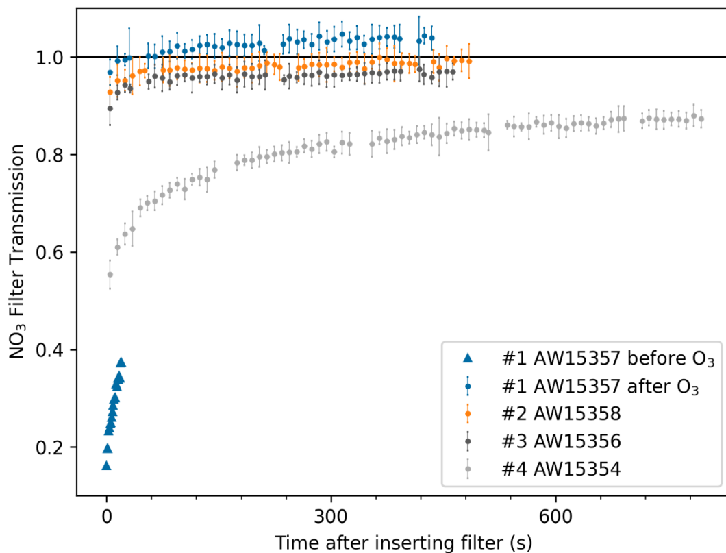
35 Figure S2: NO 3 -Transmission measurements for filters that had been used during a field campaign in Hyytiälä, Finland. AW15357 (blue) was measured before (triangles) and after (circles with error bars) the exposure to high amounts of ozone, while AW15358 (orange) was measured only afterwards. AW15356 (dark grey) was inserted into a sealed filter holder and flushed by about 3000 sccm (zero air with 15 ppmv of O 3 ) for 100 minutes while AW15354 (light grey) was not exposed to ozone prior to measuring its transmission.
