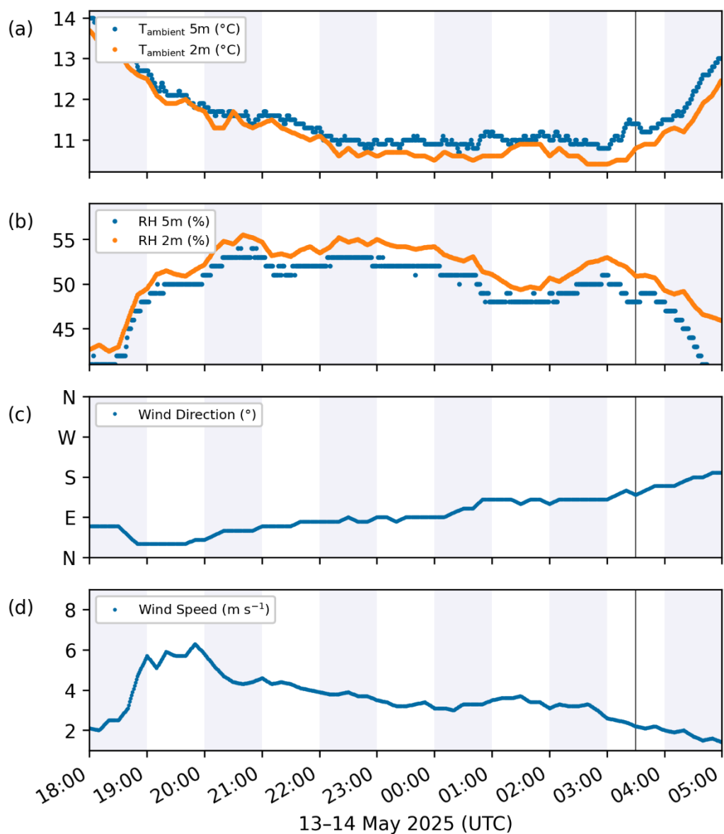
50 Figure S4: Meteorological data from a field campaign in May 2025 at the Kleiner Feldberg, Germany. Measurements of (a) ambient temperature and (b) relative humidity close to our sampling inlet (5m) and from a DWD station (2m) about 15 m to the east. (c) Wind direction and (d) wind speed provided by DWD.
