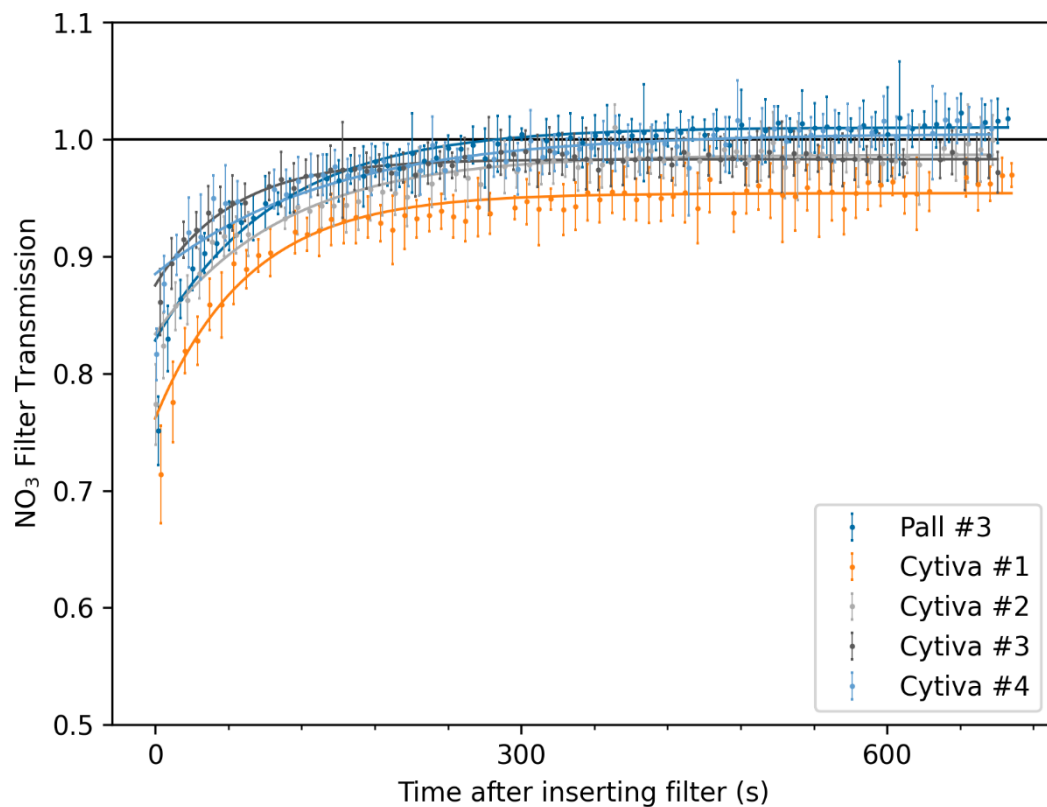
30 Figure S1: PTFE filter transmission of NO 3 using new filters from Pall and Cytiva. The error bars only represent the statistical uncertainty ( 2\sigma ) based on averaging 10-second data. Equation (3) was used to derive the maximum transmission. The measurement “Pall #4” was excluded due to major source instabilities. The overview of all T_{max} can be seen in Table 1, and a comparison between filters from Pall and Merck is shown in Figure 5.
