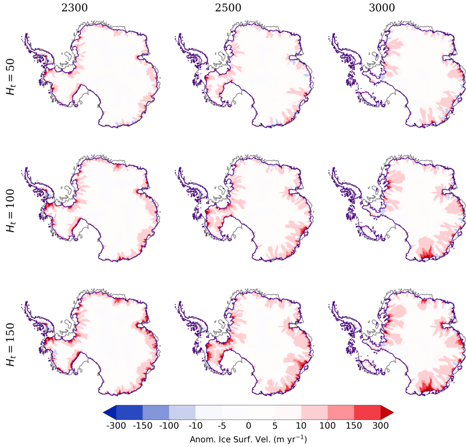
Figure 6. Ice surface velocity anomalies ( \text{m yr}^{-1} ) for the different values of at different timesteps with respect to the case where H_t = 0 m for the experiments with CESM2-WACCM (SSP5-8.5). The gray and purple lines represent the initial and evolving GL, respectively (defined as H_{af} = 0 ).
