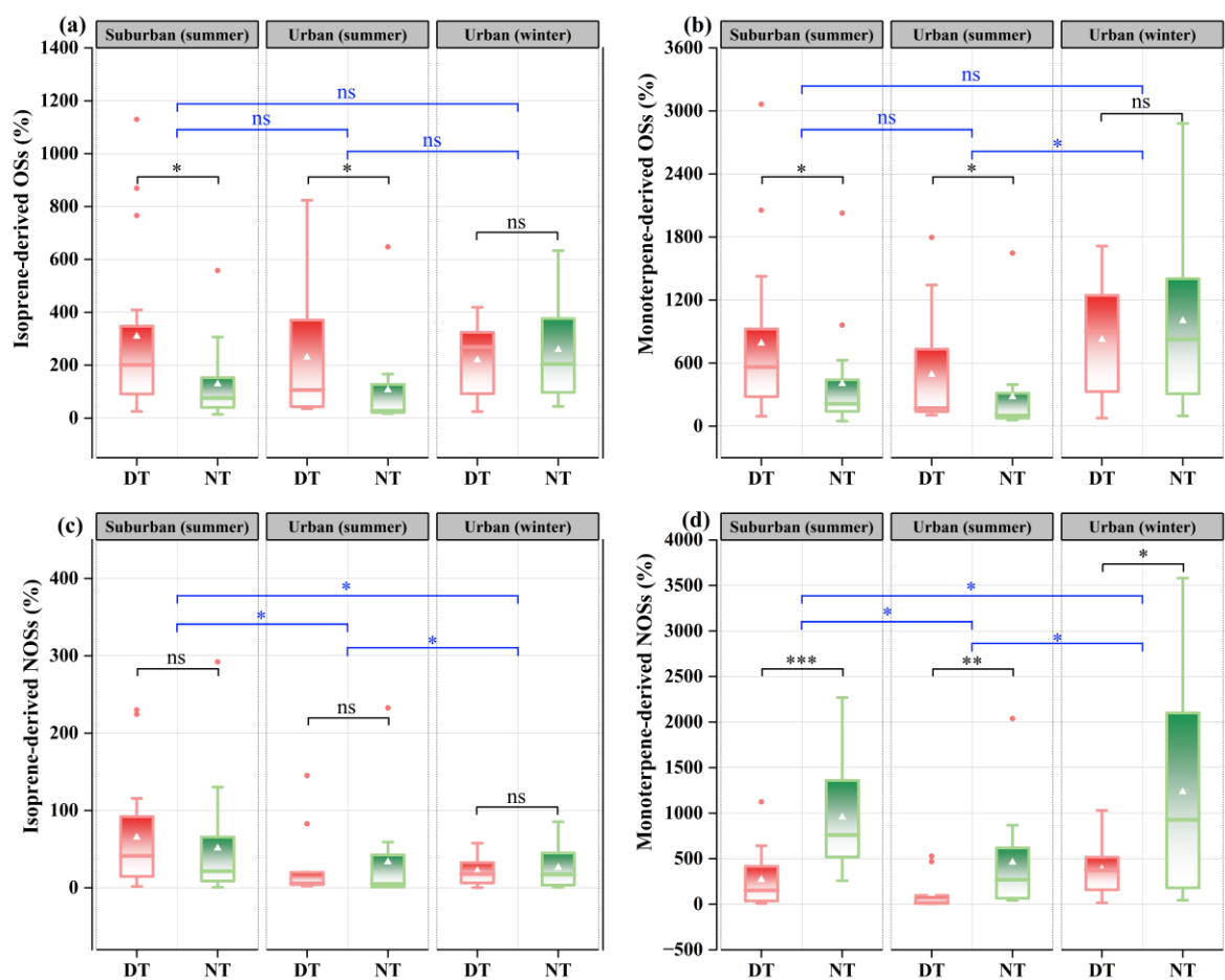
Figure 5. Spatial, seasonal, and day-night diurnal variability of isoprene- and monoterpene-derived OSs (a, b) and NOSs (c, d). The y-axis represents the relative abundances of monoterpene/isoprene-derived OSs and NOSs, defined as peak areas normalized to the internal standard. The whisker plot boundaries are between the 10th and 90th percentiles, the box displays the 25th, 50th (median), and 75th percentiles, and the triangles display the mean values. Asterisks denote statistical significance (* p < 0.05 , ** p < 0.01 , *** p < 0.001 ), while “ns” indicates no significance.
