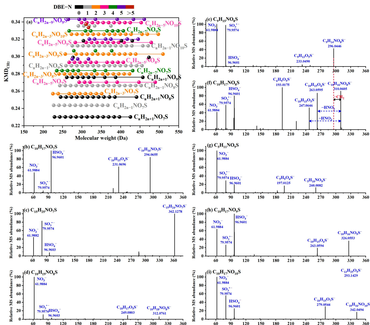
Figure S6. (a) CH 2 -based Kendrick mass defect (KMD) diagram of potential NOSs. (b–i) MS/MS fragmentation spectra of eight representative sulfur- and nitrogen-containing ions. The parent ions chosen for fragmentation were (b) C 10 H 17 NO 7 S, (c) C 15 H 25 NO 7 S, (d) C 10 H 19 NO 8 S, (e, f) C n H 2n-3 NO 8 S (n = 9 and 10), (g) C 5 H 11 NO 9 S, (h) C 10 H 17 NO 9 S, and (i) C 10 H 17 NO 10 S.
