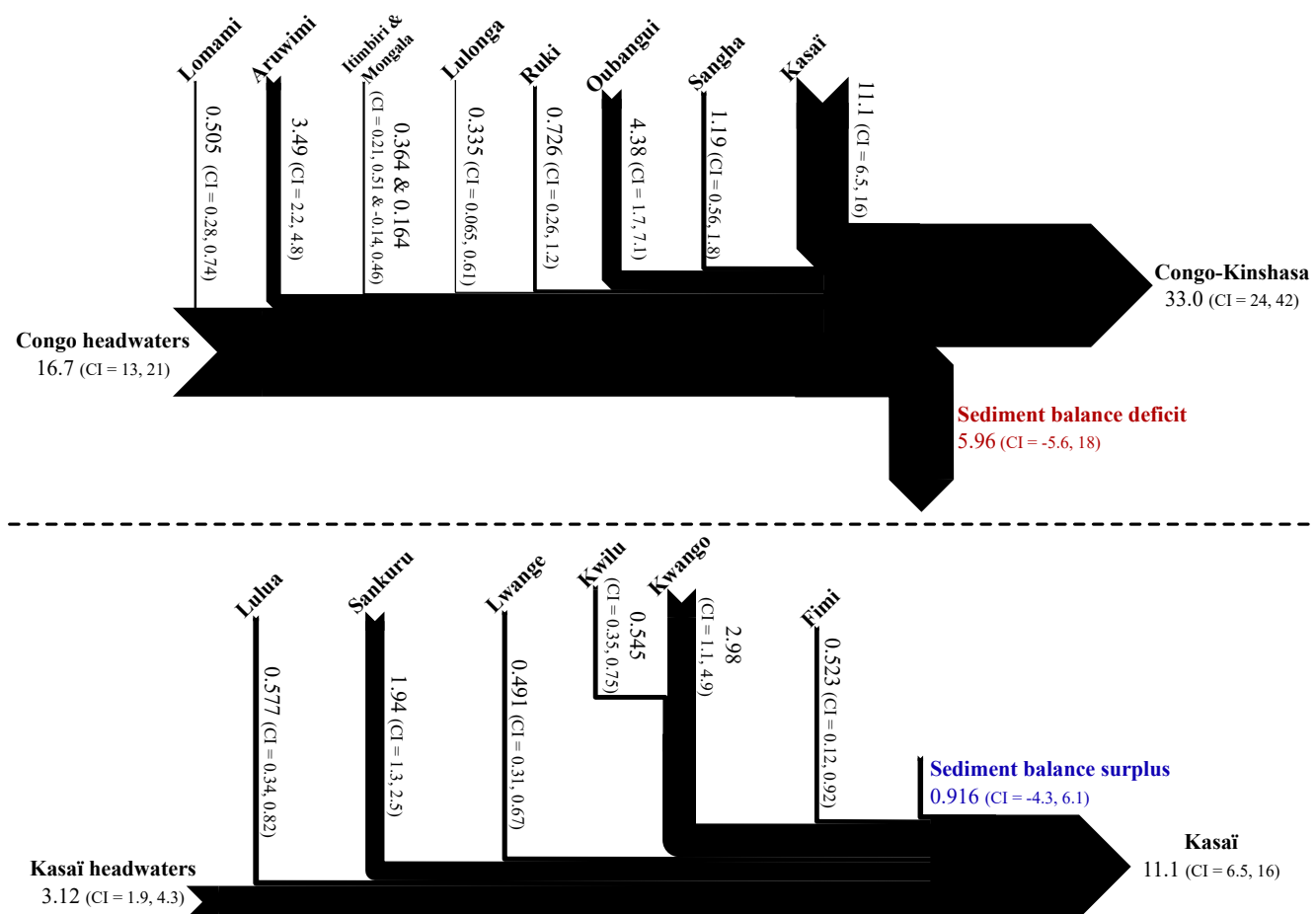
Figure 5. Median sediment yield budgets (Tg yr -1 ) for the Congo River Basin (a) and the Kasai River Basin (b) from 2015-2019. Sediment balance deficit (red) signified that the inputs (headwaters and tributaries) were higher than the output while a sediment balance surplus (blue) signified that the output was higher than the sum of all inputs. The size of lines for each component are proportional to sediment yield.
