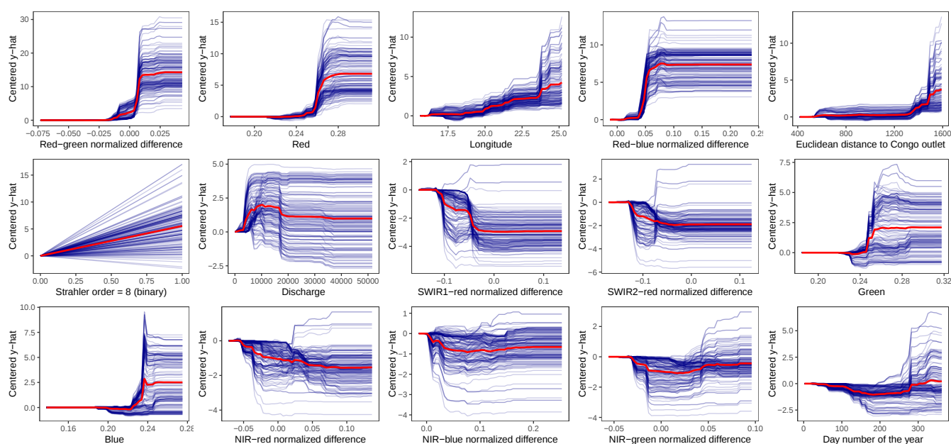
Figure A4. Partial dependence plots of variables included in our random forest model, where the horizontal axis corresponds to each variable's range of values and the vertical axis (centered y-hat) is the response of the RF model to the evolution of each variable. The blue lines are response curves for each individual observation of the training dataset, and the red line is the mean of all responses curves.
