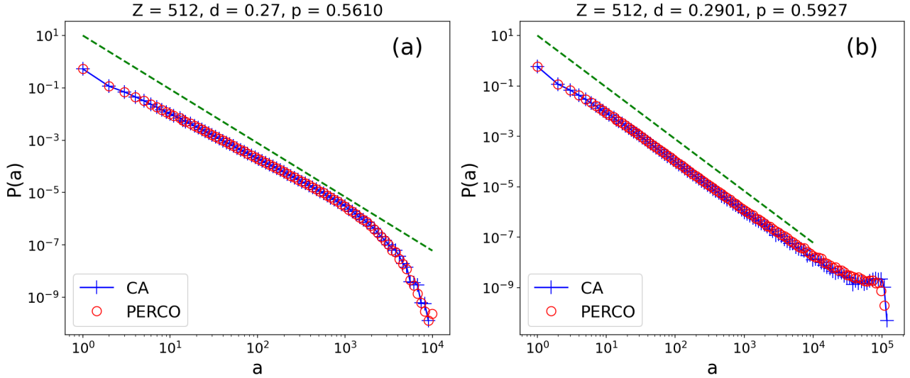
Figure 4: Probability distributions of the cluster size (cross) for CA_{0,0.27} (a) and CA_{0,0.2901} (b) for Z = 512 , together with the cluster size distributions from a 2-dimensional site percolation on a square lattice (open circle) of the same size with occupancy probability p set to the mean averaged fractional rain cluster coverage, \Omega , for the CA. Approximately 10^7 clusters are used to sample the probability distributions. The reference line (green) has slope 187/91 .
