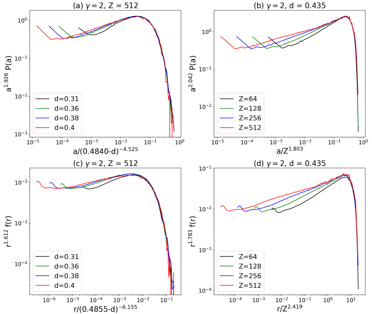
Figure 7: As in Figures 3c, d and 4c, d but for \gamma=2 with d = 0.31, 0.36, 0.38 and 0.40 for (a) and (c), and d = 0.435 for (b) and (d). The estimated exponents in (a) and (c) are \zeta_A (1.926/1.612), \eta_A (-4.525/-6.155) and d_c (0.484/0.4855) respectively, and in (b) and (d) are \zeta_A (2.042/1.783) and D_A (1.803/2.419) respectively.
