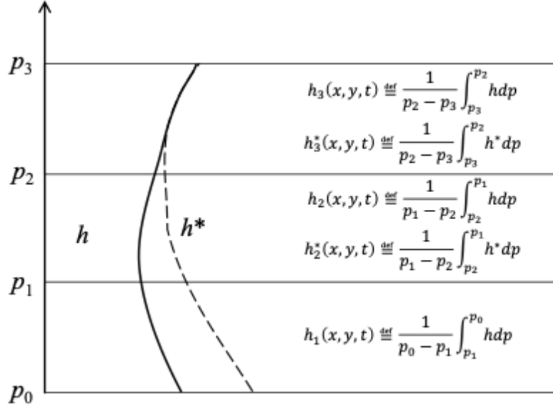
145 Figure 1: Illustration of the moist static energy profiles in the CA. Vertical axis is the atmospheric pressure. P_0 , P_1 , P_2 and P_3 are 1000 hPa, 850 hPa, 450 hPa and 100 hPa, respectively. See Appendix B for more details on how the CA variable X is defined from these unsaturated and saturated profiles.
