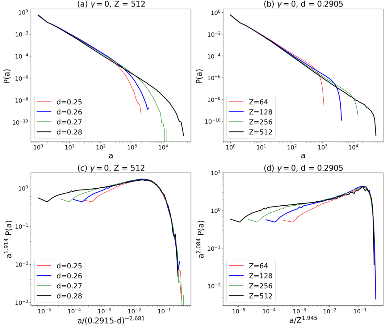
295 Figure 5: (a) Cluster size distributions for CA_{0,d} with Z = 512 and d from 0.25 to 0.28 with increment of 0.01 (b) As (a) but with Z = 64, 128, 256 and 512 for CA_{0,0.2905} . Note that the percolating clusters (largest cluster from each avalanche) are excluded in this case. (c) The data collapse for the distributions shown in (a) using estimated values for \zeta_A (1.914), \eta_A (-2.681) and d_c (0.2915) (see main 300 text), (d) Same as (c) but shows the data collapse for the distributions shown in (b), with estimated values \zeta_A (2.084) and D_A (1.945). Approximately 4 \times 10^7 clusters are used to sample each distribution shown in the plots.
