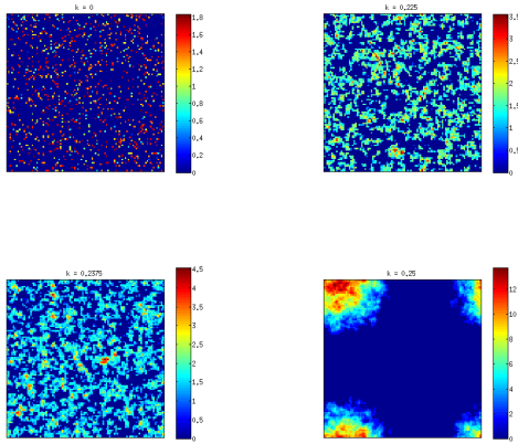
Figure C1: Snapshot of model run based on the distribution of variable X.
