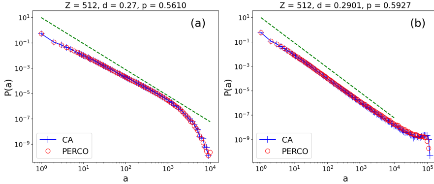
255 Figure 4: Probability distributions of the cluster size (cross) for CA_{0,0.27} (a) and CA_{0,0.2901} (b) for Z = 512 , together with the cluster size distributions from a 2-dimensional site percolation on a square lattice (open circle) of the same size with occupancy probability p set to the mean averaged fractional rain cluster coverage, \Omega , for the CA. Approximately 10^7 clusters are used to sample the probability distributions. The reference line (green) has slope 187/91.
