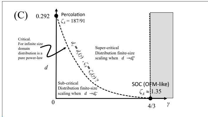
Figure 11: Characteristics of the sCA (CA excluding the representation of the GW1 dynamics in its toppling mechanisms). (a) The distribution of cluster area for different domain size ( Z = 16, 32, 64 ) and (b) its data collapse for the sCA with \gamma = 4/3 and with d \rightarrow 0^+ . (c) Schematic illustrating the hypothetical phase space of the sCA_{\gamma,d} . The curve d = d_c(\gamma) represents the unknown critical line of the sCA. sCA is unphysical beyond \gamma = 4/3 (stippled area).
