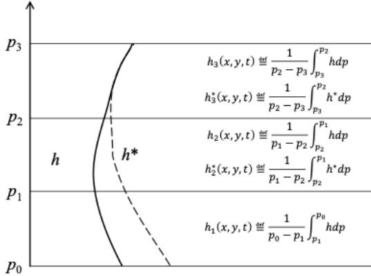
145 Figure 1: Illustration of the moist static energy profiles in the CA. Vertical axis is the atmospheric pressure. p_0, p_1, p_2 and p_3 are 1000 hPa, 850 hPa, 450 hPa and 100 hPa, respectively. See Appendix B for more details on how the CA variable X is defined from these unsaturated and saturated profiles.
