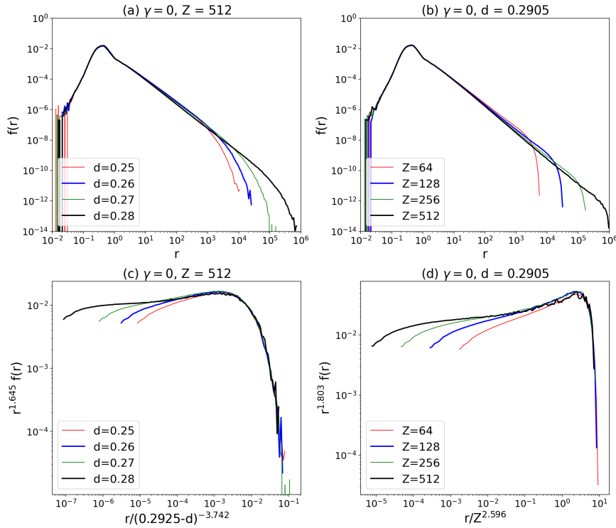
Figure 6: As in Figure 3 but for the distributions of the cluster total rain rate, with estimated values in (c) \zeta_1 (1.645), \eta_1 (-3.742) and d_c (0.2925) and in (d) \zeta_1 (1.803) and D_1 (2.596). Note the very small f(r) values for small r in panels (a) and (b), which are due to the single-cell clusters in the model that toppled during simulation and contributed to the pdf.
