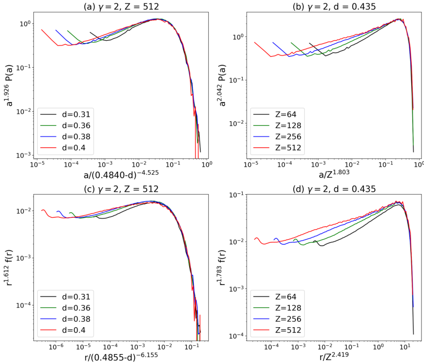
Figure 2: As in Figures 3c, d and 4c, d but for \gamma=2 with d=0.31, 0.36, 0.38 and 0.40 for (a) and (c), and d=0.435 for (b) and (d). The estimated exponents in (a) and (c) are \zeta_A(1.926/1.612) , \eta_A(-4.525/-6.155) and d_c(0.484/0.4855) respectively, and in (b) and (d) are \zeta_d(2.042/1.783) and D_d(1.803/2.419) respectively.
