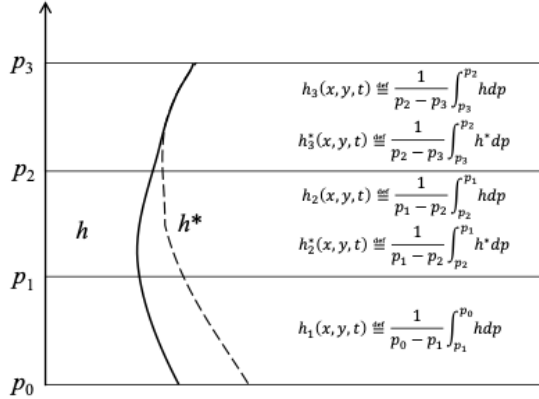
Figure 1: Illustration of the moist static energy profiles in the CA. Vertical axis is the atmospheric pressure. P_0, P_1, P_2 and P_3 are 1000 hPa, 850 hPa, 450 hPa and 100 hPa, respectively. See Appendix B for more details on how the CA variable X is defined from these unsaturated and saturated profiles.
