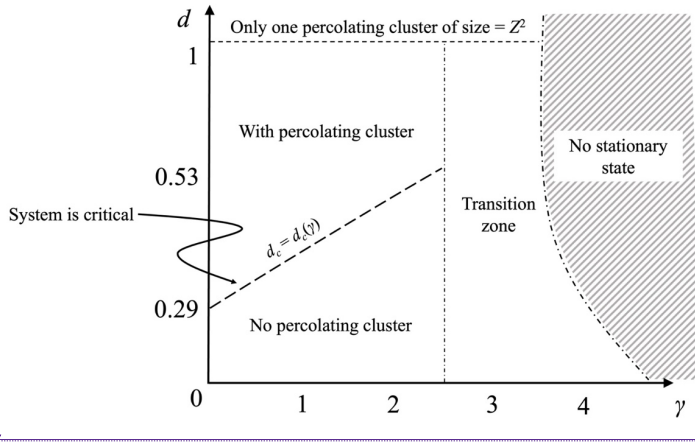
Figure 3: Schematic representation of the phase space of CA as a function of the drive magnitude d and the coupling constant \gamma . The dash line indicates the critical drive magnitude d_c that is \gamma -dependent, a state when percolating cluster emerges and the characteristics scale diverges. For infinite-size domain, distribution is pure power law. When d \rightarrow d_c^+ distribution is finite scaling whose characteristic scale depends on the domain size. The percolating cluster is more filling with increasing d and increasing separation of scales. When d \rightarrow d_c^- (no percolation cluster), distribution is finite scaling whose characteristic scale depends on d - d_c . When \gamma becomes large, there is a transition zone when the system takes too long computational resource to reach stationarity or stationary period is too short to collect sufficient data for reliable characterization.
