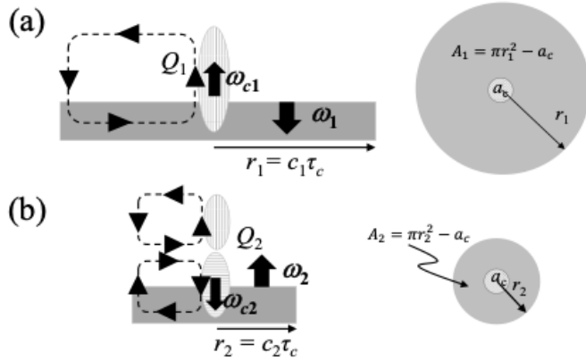
Figure 2: Schematic showing the effects on the atmosphere due to the (a) GW1 ( l = 1 ) and (b) GW2 ( l = 2 ) gravity bores. The diagrams on the left represent a vertical cross-section of the troposphere that includes the convective site. The vertical (horizontal) stippled ellipse at the middle of the figure represents a positive (negative) heating anomaly. The greyed region is a cross section of the volume of clear sky atmosphere within the sub cloud layer behind the wave fronts at a time \tau_c . \omega_1 and \omega_2 are the area-time averaged velocities in the clear sky region behind the wave fronts (greyed region) due to the heating mode Q_1 and Q_2 . The averaging is done over the area on the top of the boundary layer (top of the greyed area) and across time from the time convection is triggered to a duration \tau_c . \omega_1 and \omega_2 are the area-time averaged vertical velocity confined within the convective site. The area averaging is done across the convective site only in this case. The cross-section of the instantaneous (radially symmetric) circulation at time \tau_c after the convection is triggered is represented by the dotted loops with arrow indicating the direction of the circulation. The diagrams on the right represents the top view of the corresponding cross section views.
