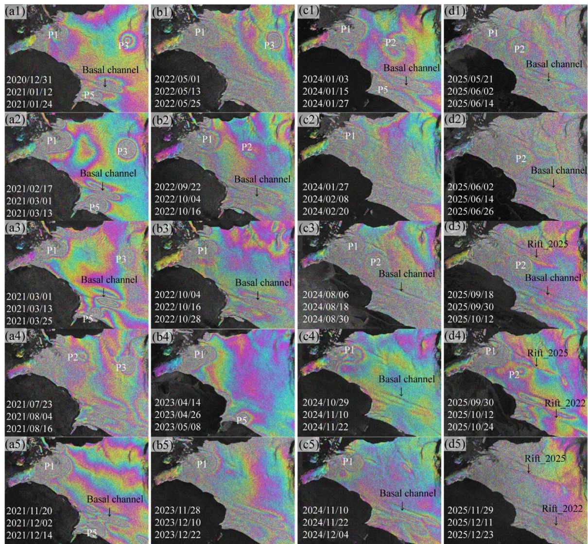
Figure 9. Changes in pinning points P1, P2, P3, and P5 derived from double-difference interferograms over the N-PIIS from 2021 to 2025. Panels (a–d) show results for 2021, 2022, 2023, 2024, and 2025, respectively.
