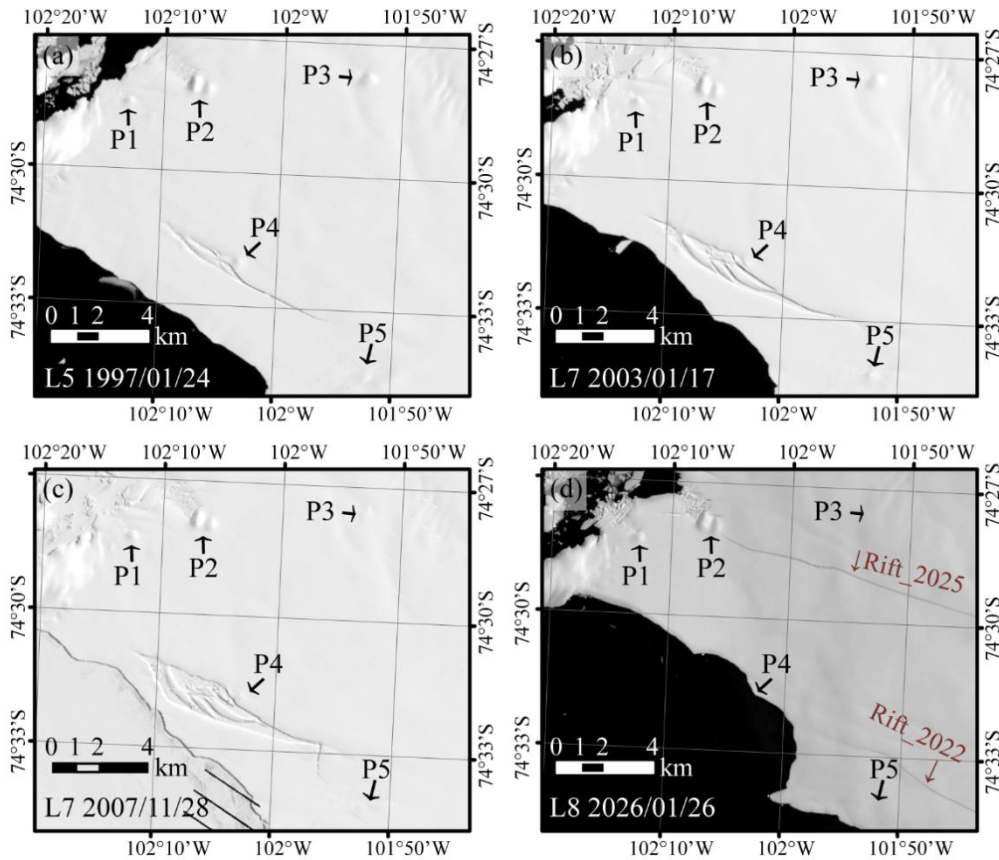
Figure 7. Changes in pinning points in Landsat imagery. Panels (a–d) show pinning-point conditions on 24 January 1997 (Landsat-5), 17 January 2003 (Landsat-7), 28 November 2007 (Landsat-7), and 26 January 2026 (Landsat-8), respectively. Panel (d) also reveals the positions of rifts that appeared in 2022 (Rift_2022) and 2025 (Rift_2025).
