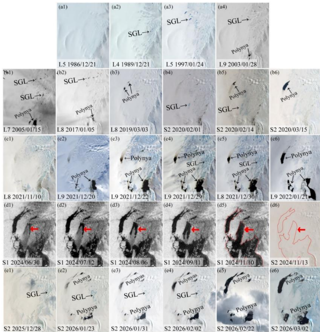
Figure 5. Distribution and development of supraglacial lakes (SGL) and polynyas within the N-PIIS. (a) Overview map in 1986, 1989, 1997, and 2003. (b) Overview map in 2005, 2017, 2019, and 2020. (c) Overview of polynya development during the 2021/2022 austral summer. (d) Decrease in backscatter coefficient observed in Sentinel-1 imagery from June to November 2024 (red arrows). (e) Overview of polynya development during the 2025/2026 austral summer.
