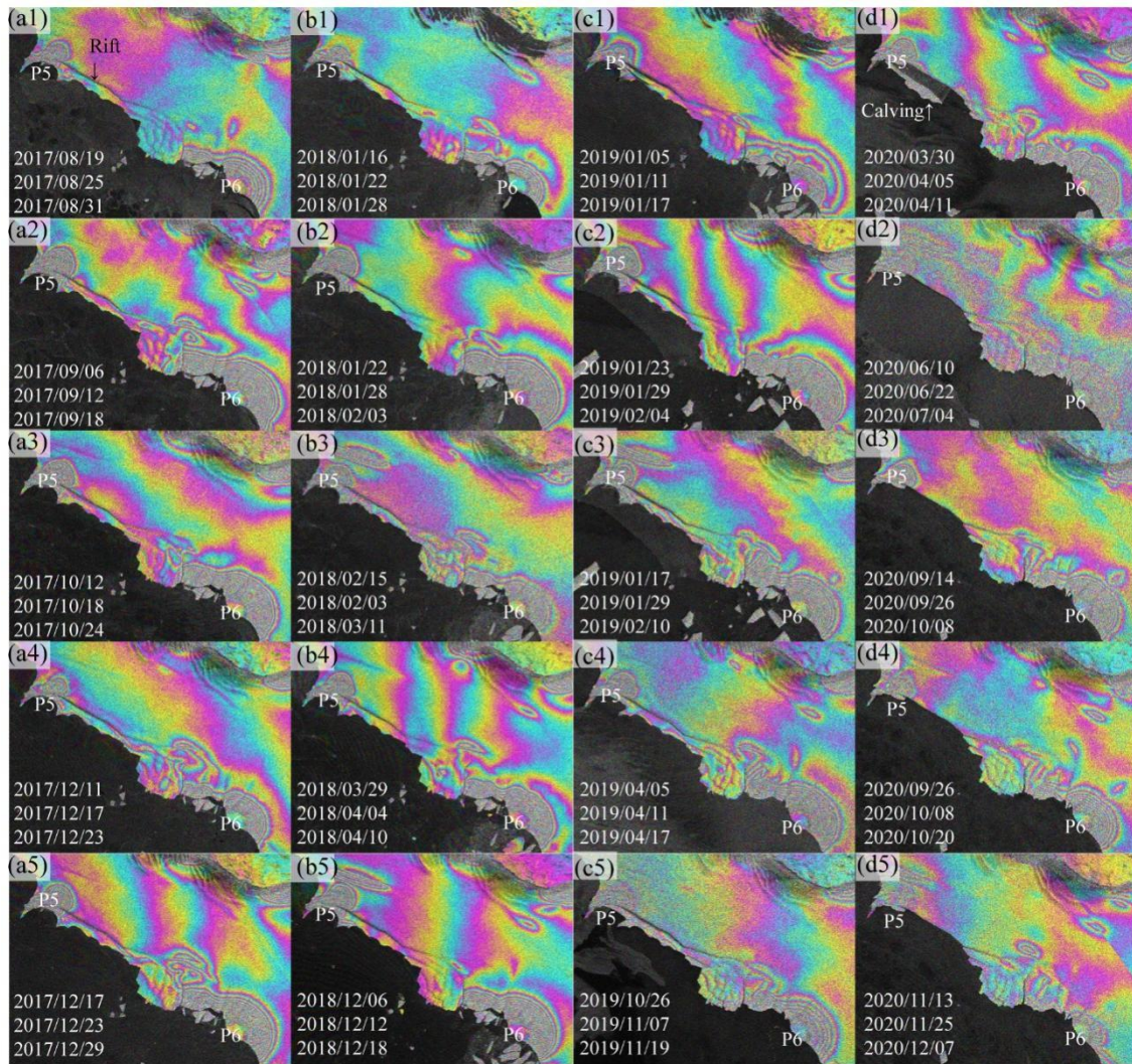
240 Figure 12. Double-difference interferograms of the N-PIIS from 2017 to 2020. Panels (a–d) show results for 2017, 2018, 2019, and 2020, respectively.
