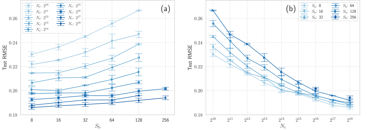
Figure B3. Test RMSEs of DAN as a function of the batch size S_b for a selection of N_r values (panel a) and as a function of the number of dataset trajectories N_r for a selection of S_b values (panel b). For each pair (S_b, N_r) , an ensemble of 3 \mathbf{a}_\theta operators is learned, from which error bars (plus or minus the standard deviation) are estimated and added to the curve plots.
