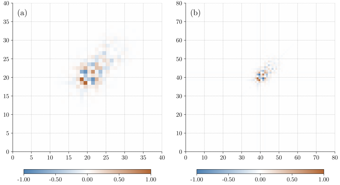
Figure 1. Plot of the normalised mean marginal gain \frac{[\bar{\Omega}_r]_{ij}}{\max |[\bar{\Omega}_r]_{ij}|} \frac{|\bar{\Omega}_{ij}^{(r)}|}{\max |\bar{\Omega}_{ij}^{(r)}|} in the fully observed DA configuration of the L96 model, obtained with a model size of N_x = 40 (panel a) and N_x = 80 (panel b).
