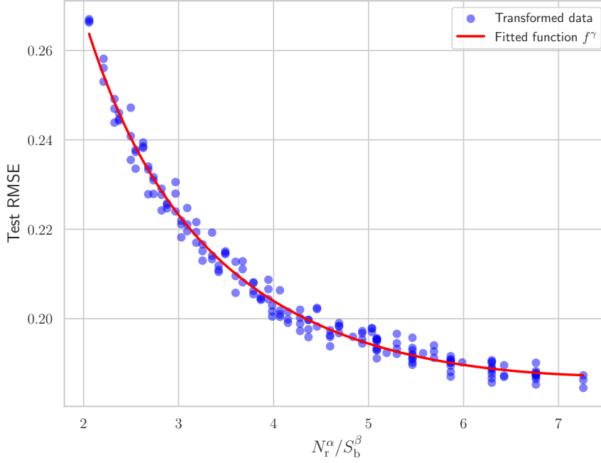
Figure B4. Checking the relevance of the functional regression by plotting the fit function f^\gamma with respect for to N_r^\alpha / S_b^\beta (curve), and of the test RMSE results (dots).
