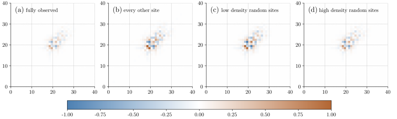
Figure 2. Plot of the mean marginal gain \frac{[\bar{\Omega}_r]_{ij} \bar{\Omega}_{ij}^{(r)}}{\max |[\bar{\Omega}_r]_{ij} \bar{\Omega}_{ij}^{(r)}|} normalised by the maximum of its absolute value over all entries and over the four panels, in several sparse observation DA configuration of the L96 model.
