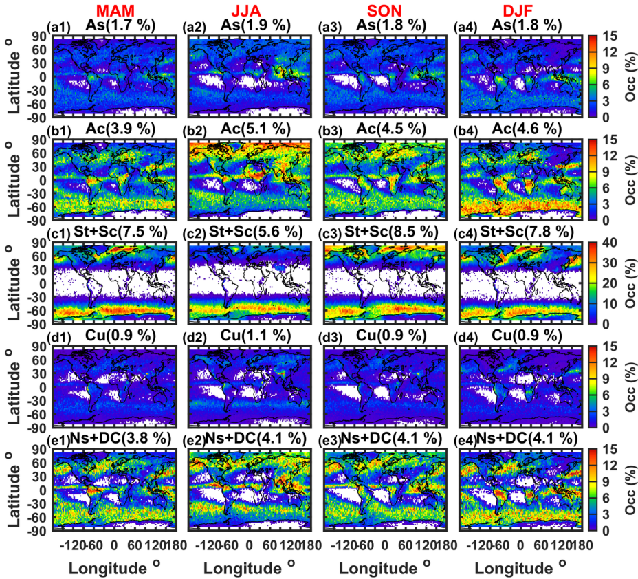
555 Figure 5: Seasonal spatial distributions of mixed-phase cloud occurrence for the five cloud types. Rows a–e correspond to As, Ac, St+Sc, Cu, and Ns+DC, respectively. Columns 1–4 represent March–April–May (MAM), June–July–August (JJA), September–
