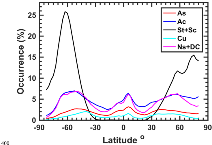
400 Figure 2: Zonal mean mixed-phase cloud occurrence for different cloud types: As, Ac, St+Sc, Cu, and Ns+DC. Each curve represents the zonal mean occurrence for the corresponding cloud type. The y-axis shows mixed-phase cloud occurrence (%), and the x-axis represents latitude (°) with a 2.5° resolution.
