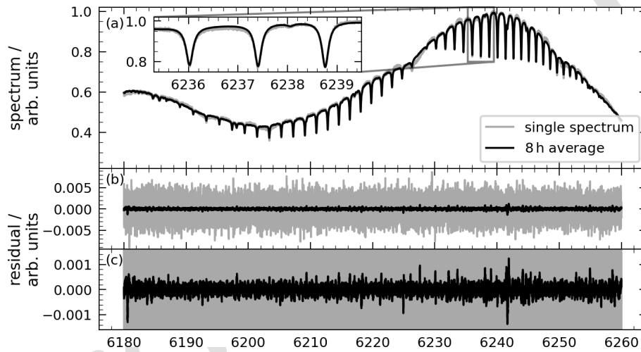
Figure 3. Panel (a): Single spectrum (1 min acquisition time) in comparison to 8 h average, along the open path of 3106 m total length. Inset shows a zoom into three CO 2 absorption lines. Panels (b) and (c): fit residuals, with different levels of zoom. Spectral sampling of 3.34 \times 10^{-3} \text{ cm}^{-1} . The single spectrum was measured on 30 October 2025, 14:27 UTC. The average was acquired on 30 October 2025, from 08:30 to 16:30 UTC.
