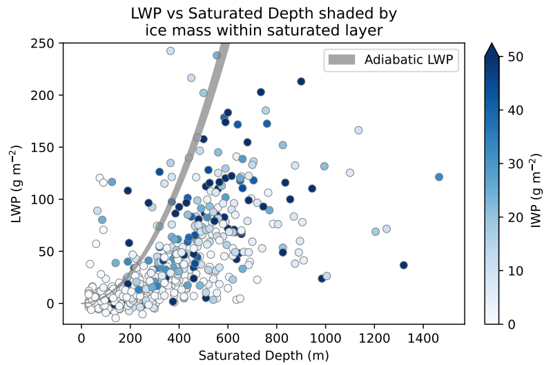
Figure A4. Liquid water path as a function of saturated depth for cases with a single saturated layer and a cloud base temperature between -20 and -10 degrees C, colored by the amount of ice within the saturated layer. The grey shaded region shows the adiabatic liquid water path predicted as a function of saturated depth for cloud base temperatures between -20 and -10 degrees C. Displays the same cases as in Figure 2b of the main manuscript.
