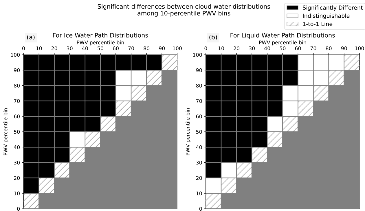
Figure A5. Significant difference flags between all pairs of ice (a) and liquid (b) water path distributions by PWV percentile from Figure 3. Significant difference is determined at the 95% level by a two-sample Kolmogorov-Smirnov test.
