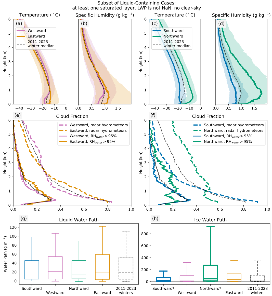
Figure A8. Same as Figure 4 in the main manuscript, except all panels display the same subset of cases: at least one saturated layer is present, the liquid water path is defined, and the radar does not detect clear sky.
