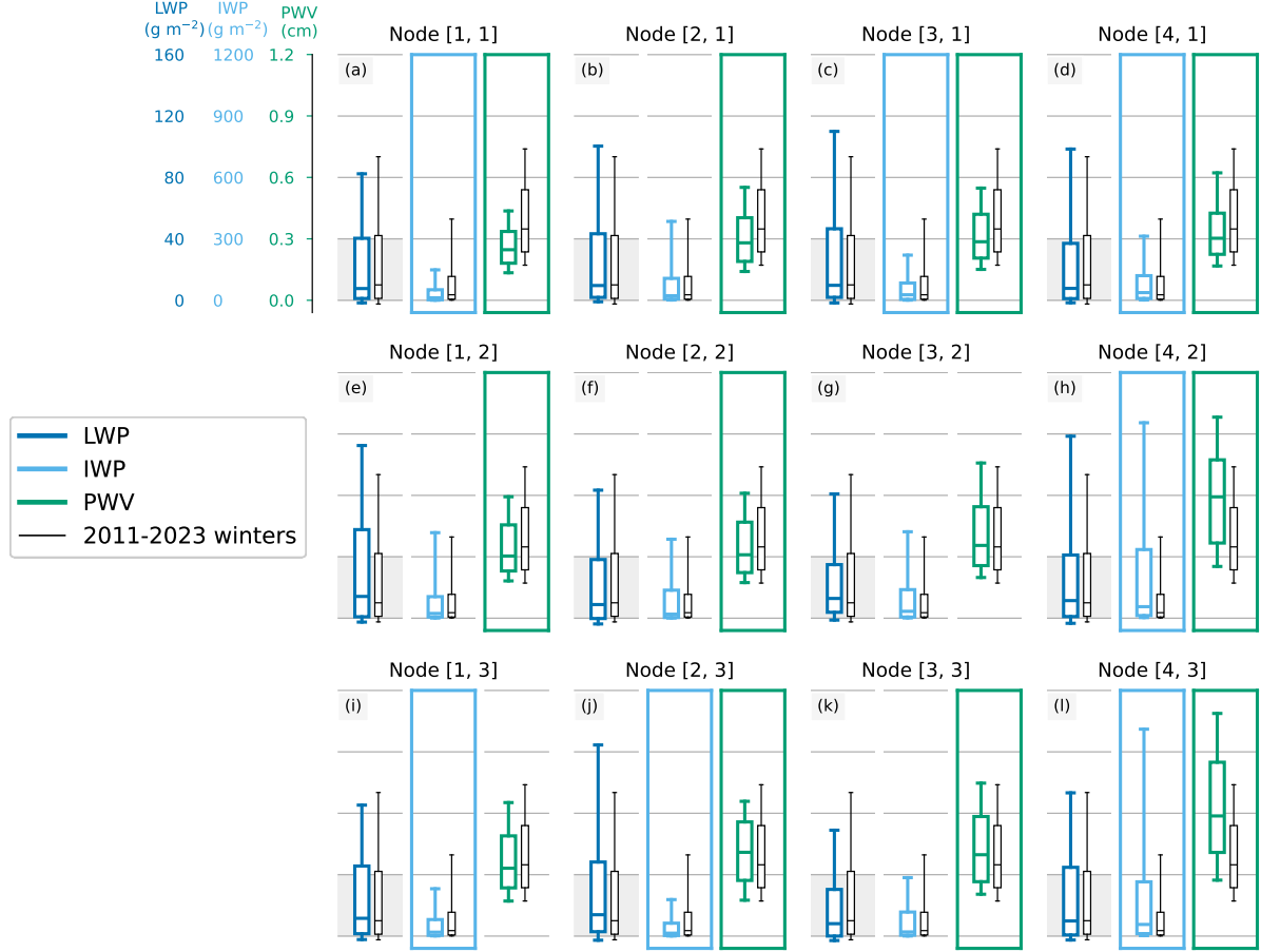
Figure 7. Box-and-whisker plots of liquid water path (dark blue) on the left, ice water path (light blue) in the middle, and precipitable water vapor (green) on the right during each SOM node. Clear-sky cases are excluded from all distributions. Whiskers extend to the 10 th and 90 th percentiles. The black plots are the distribution over all 2011-2023 winters and therefore the same for all nodes. If the distribution for a given node is significantly different from that of all 2011-2023 winters, that plot is outlined in the corresponding color.
