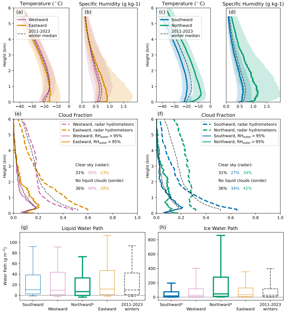
Figure 4. Panels compare conditions during westward (45° to 135°; in pink) and eastward (225° to 315°; in orange) winds (panels a, b, e, g) and between southward (315° to 45°; in blue) and northward (135° to 225°; in green) winds (panels c, d, f, h) at 500 m at North Slope of Alaska as detected by radiosondes: temperature (a, c) and specific humidity (b, d) profiles; vertical profiles of cloud fraction from the radar (e, f; dotted lines) and liquid cloud fraction from soundings (solid lines); box-and-whisker plots of liquid (g) and ice (h) water path, excluding radar-detected clear sky cases. Shaded regions correspond to the 25 th to 75 th percentile range (a-d). Saturated regions (e, f) are defined as RH>95% in soundings. Box-and-whisker plots (g, h) are bolded and labeled with an asterisk if the distribution is significantly different from the 2011-2023 winter distribution, and whiskers extend to the 10 th and 90 th percentiles. Black dashed lines in all panels are the median over all 2011-2023 winters, while the black solid line in (e, f) is the 2011-2023 winter median for the RH>95% condition.
