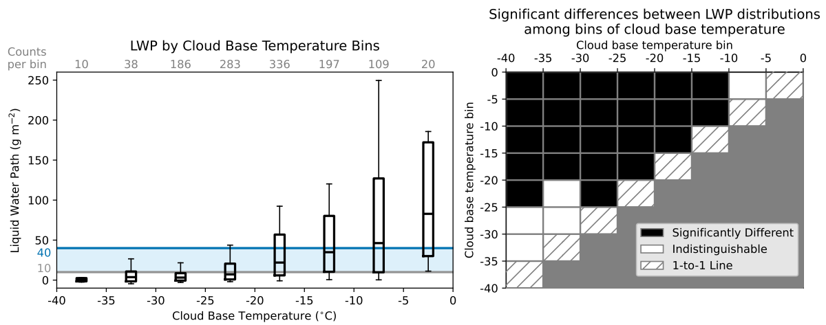
Figure A3. Liquid water path distributions as a function of cloud base temperature in 5-degree bins for single-layer cloud cases (a) and a significant difference matrix comparing all pairs of LWP distributions at the 95% confidence level using a Kolmogorov-Smirnov test.
