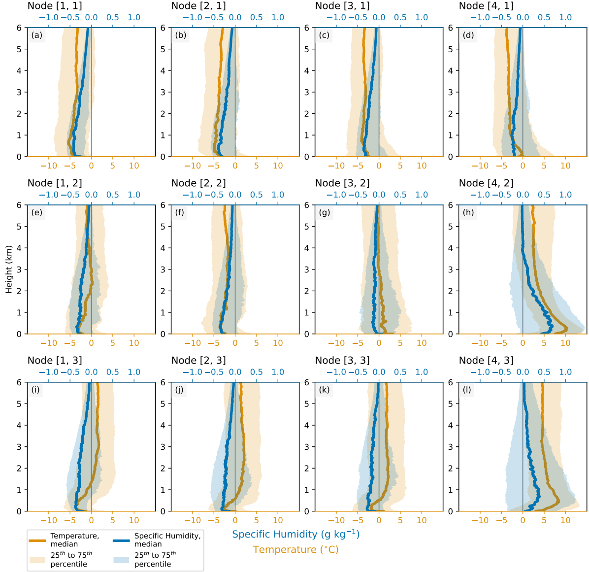
Figure 6. Vertical profiles of the difference between conditions during each node and the 2011-2023 extended winter mean for temperature (gold) and specific humidity (blue) from radiosondes. For each node, the median (solid line) and 25 th to 75 th percentile (shaded region) of anomalies from the winter mean are represented. The lower x-axis gives temperature in degrees Celsius while the upper x-axis shows specific humidity in g kg -1 ; both axes scales are the same for all panels. The node label is given above each plot, and the positions within the grid are the same as in Fig. 5.
