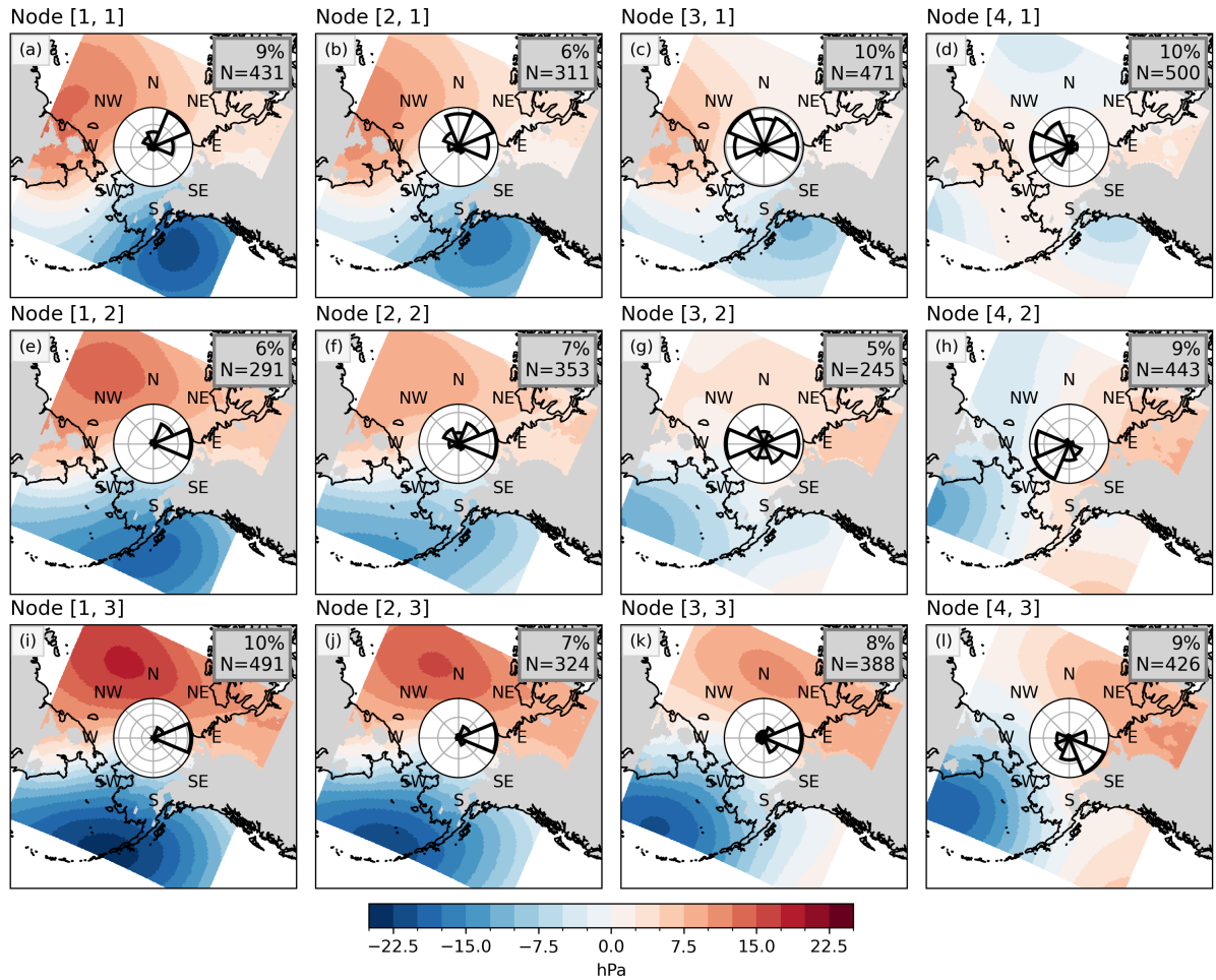
Figure 5. Self-organizing maps (SOM) show the correspondence between sea level pressure anomalies and 500-m wind direction at North Slope of Alaska. Shaded contours show the sea level pressure anomalies based on ERA5 output of each self-organizing map (SOM) node are shown in shaded contours while a wind rose gives the distribution of 500 m wind direction according to sondes radiosondes at North Slope of Alaska-NSA during each node. The frequency of each node from 2011-2023 is given in the upper right-hand corner.
