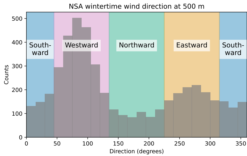
Figure A7. The distribution of 500 m wind direction at NSA, with the ranges defining northerlies-southward (blue), easterlies-westward (pink), southerlies-northward (green), and westerlies-eastward (orange) winds shaded.
