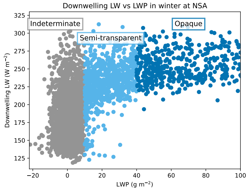
Figure A2. Downwelling longwave radiation at the surface as a function of liquid water path. Points are colored according to the three liquid water path categories defined in the paper: Thin Indeterminate ( <10 \text{ g m}^{-2} ), Semi-transparent ( 10\text{-}40 \text{ g m}^{-2} ), and Opaque ( >40 \text{ g m}^{-2} ). Downwelling longwave radiation is the downwelling longwave hemispheric irradiance reported in the qcrad1long.c2 datastream.
