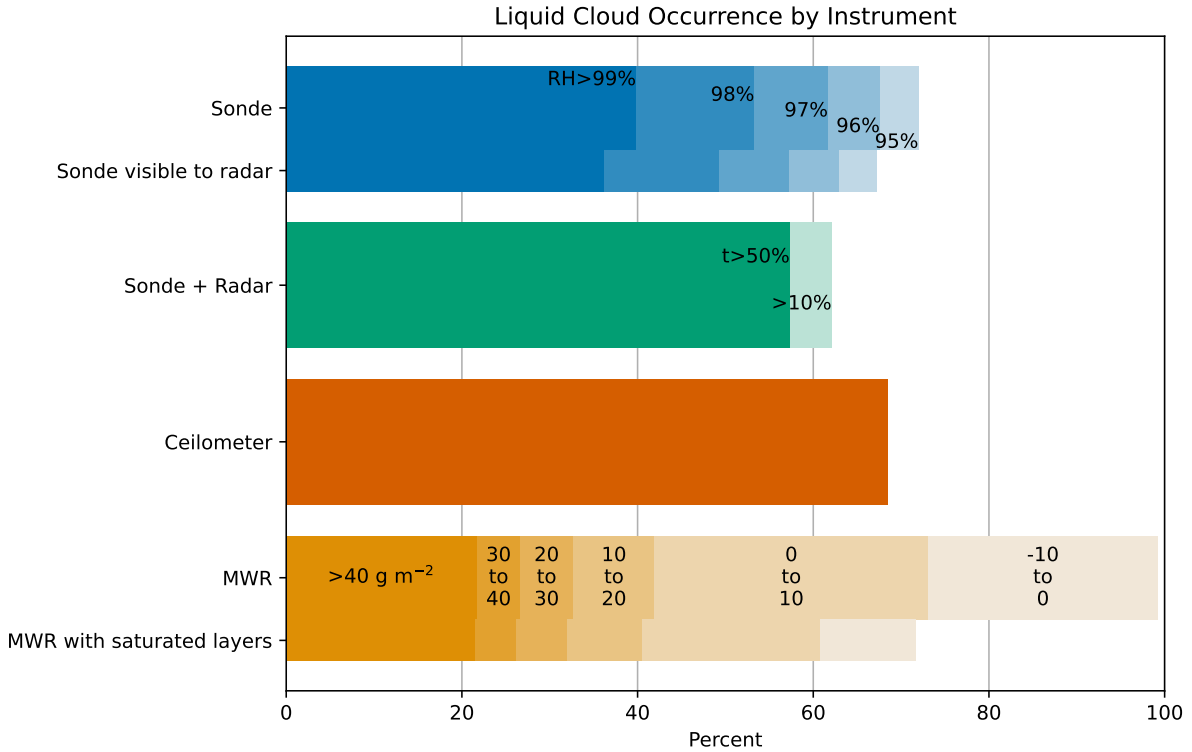
Figure 1. Liquid-containing clouds are ubiquitous at the North Slope of Alaska in winter, but the precise liquid cloud fraction varies by instrument and detection threshold. Each bar shows the The percent of the time that liquid-containing clouds were detected at NSA by the corresponding each instrument for November through March of 2011-2023. All percents are relative to times when no instruments (sonde, radar, ceilometer, and MWR) were missing data, for a total of 3,400 data points. Shading for the ‘Sonde’ bars corresponds to different relative humidity thresholds from 95% (pale blue) to 99% (dark blue), while ‘Sonde in radar range’ shows the same but only based on sonde readings above 165 m, which is the lowest range gate detected by the cloud radar. ‘Sonde + Radar’ is based on times when the relative humidity was above 95% and the cloud radar detected hydrometeors in at least one of the liquid-saturated regions. Over 50% of values at a given height had to be above the signal-to-noise threshold to be retained in the hourly average for t > 50\% , and only 10% for t > 10\% . ‘Ceilometer’ is based on times when the ceilometer detected at least one cloud base height. ‘MWR’ is shaded according to the liquid water path in \text{g m}^{-2} , displayed in bins from highest (dark gold) to lowest (pale gold) values, while “MWR with saturated layers” shows the same liquid water path bins but only for times when at least one saturated layer was detected in the corresponding sonde.
