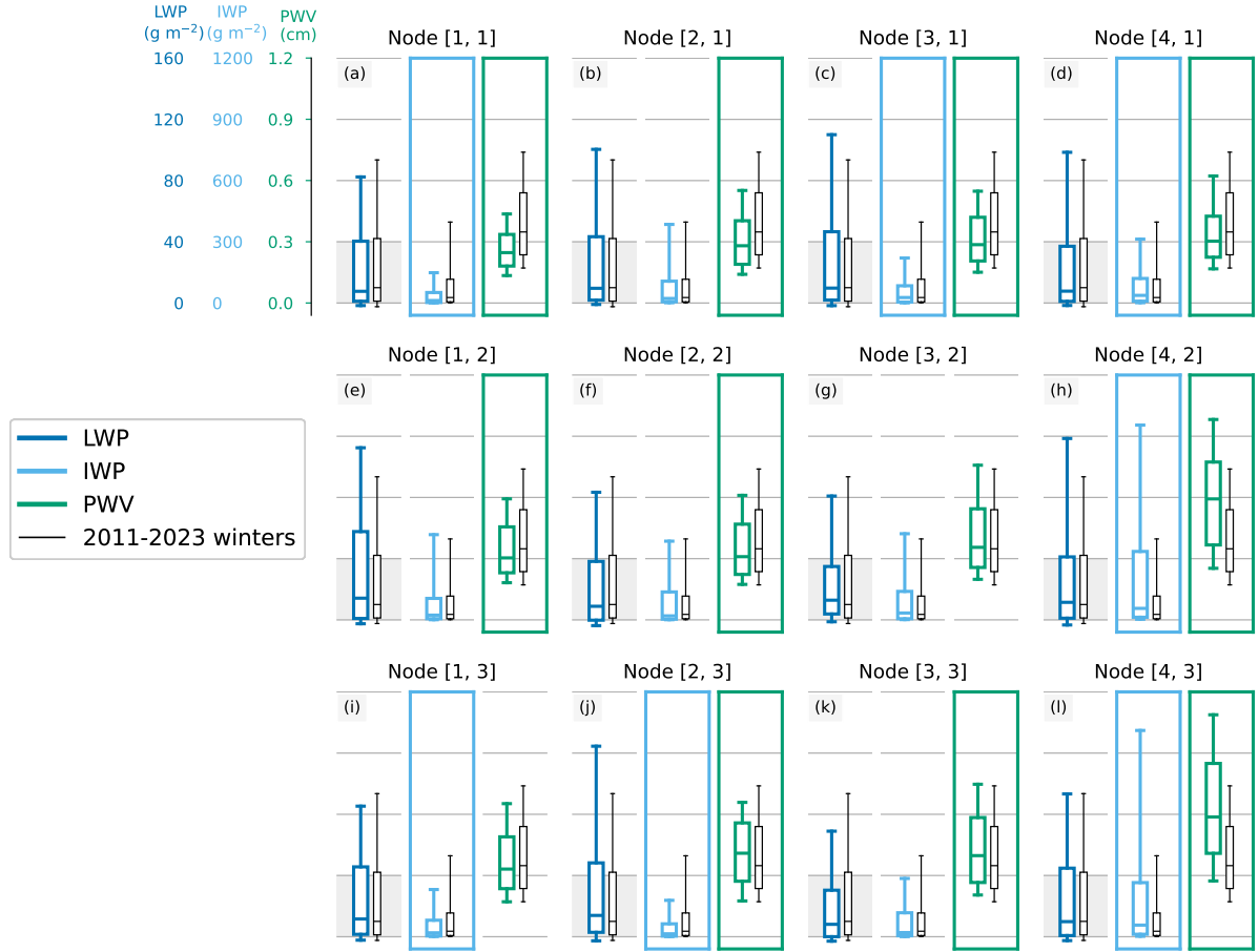
Figure 7. Liquid water path distributions during each of the large-scale circulation regimes characterized by SOMs are statistically indistinguishable from the climatological distribution while ice water path and precipitable water vapor vary significantly. Each node panel contains three box-and-whisker plots with whiskers out to the 10 th and 90 th percentiles of liquid water path (dark blue) on the left, ice water path (light blue) in the middle, and precipitable water vapor (green) on the right during each SOM node. Clear-sky cases are excluded from all distributions. Whiskers extend to the 10 th and 90 th percentiles. The black plots are all-winter climatology-the distribution over all 2011-2023 winters and therefore the same for all nodes. If the distribution for a given node is significantly different from climatology that of all 2011-2023 winters, that plot is outlined in the corresponding color.
