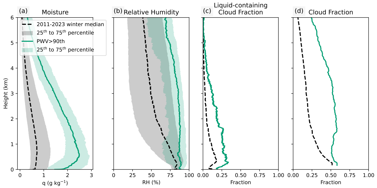
Figure A9. Comparing climatological 2011-2023 winter median vertical profiles (in black) of specific humidity (a), relative humidity (b), saturated layer fraction (c), and cloud fraction (d) to those when PWV is above its 90 th percentile (in green). Shaded regions demarcate the 25 th to 75 th percentile range over all cases while solid and dashed lines indicate the median.
