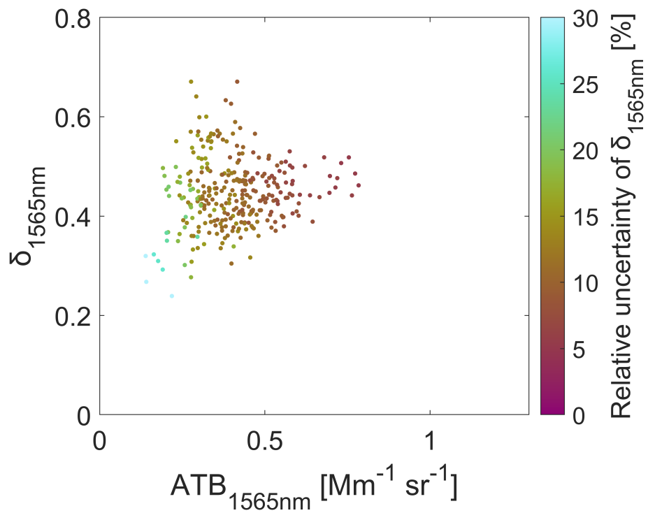
Figure 12. Scatterplot of ATB_{1565nm} versus \delta_{1565nm} at the volcanic plume layer extracted from hourly lidar data. The color indicates the relative uncertainty of \delta_{1565nm} .
