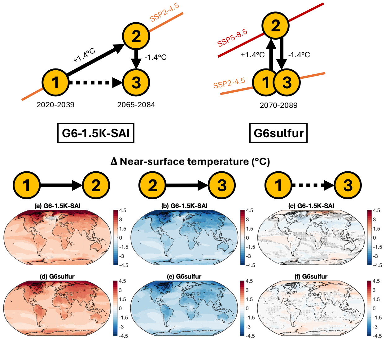
Figure 2. From Lee et al. (2026b): Maps of near-surface air temperature changes (in °C) for G6-1.5K-SAI and G6sulfur multi-model means, between three different periods: (1) the reference period, corresponding to the period over which the GMSAT targets are defined; (2) the warmed world; and (3) the new climate state reached under GHG plus SAI. The left column plots the difference between (1) and (2), representing the impacts of global warming alone; the middle column plots the difference between (2) and (3), representing the impacts of SAI alone; and the right side column plots the difference between (1) and (3), representing the combined impacts of warming and SAI. For G6-1.5K-SAI, period (1) is SSP2-4.5 2020-2039, period (2) is SSP2-4.5 2065-2084, and period (3) is G6-1.5K-SAI 2065-2084. For G6sulfur, all three periods are averages of 2070-2089 data, in which the amount of cooling is approximately the same (1.4°C) as the last 20 years of G6-1.5K-SAI. Shading represents areas where models disagree on the sign of the change (fewer than 3 out of 4 for G6-1.5K-SAI, and fewer than 4 out of 6 for G6sulfur).
