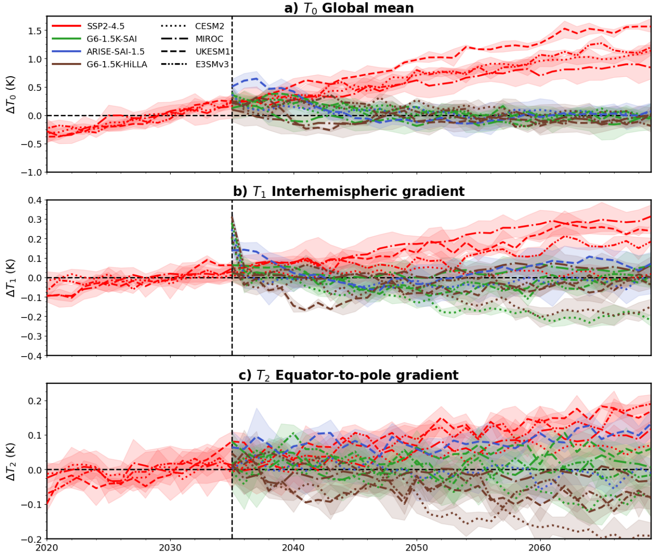
Figure A1. Evolution of a) global-mean temperature T_0 , b) interhemispheric temperature gradient T_1 , and c) equator-to-pole temperature gradient T_2 from 2020-2069 for SSP2-4.5 (red) and SAI scenarios (G6-1.5K-SAI, green; ARISE-SAI-1.5, blue; HiLLA-SAI, brown). Line style denotes the climate model (CESM, MIROC, UKESM and E3SM) and line shading show the ensemble spread.
