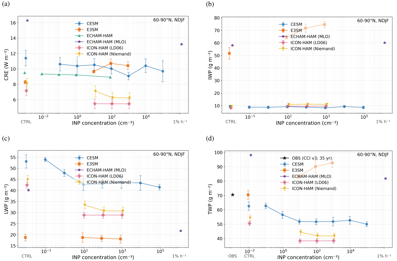
Figure A2. Arctic-mean (60–90°N) NDJF response as a function of INP concentration for all MCT-MIP Level 0 models and configurations. (a) Net cloud radiative effect (CRE, \text{W m}^{-2} ); the control value is shown at the left margin. (b) Ice water path (IWP, \text{g m}^{-2} ); E3SM's anomalously high and monotonically increasing IWP explains its warming CRE response. (c) Liquid water path (LWP, \text{g m}^{-2} ). (d) Total water path (TWP, \text{g m}^{-2} ). Error bars denote the inter-annual standard error of the mean.
