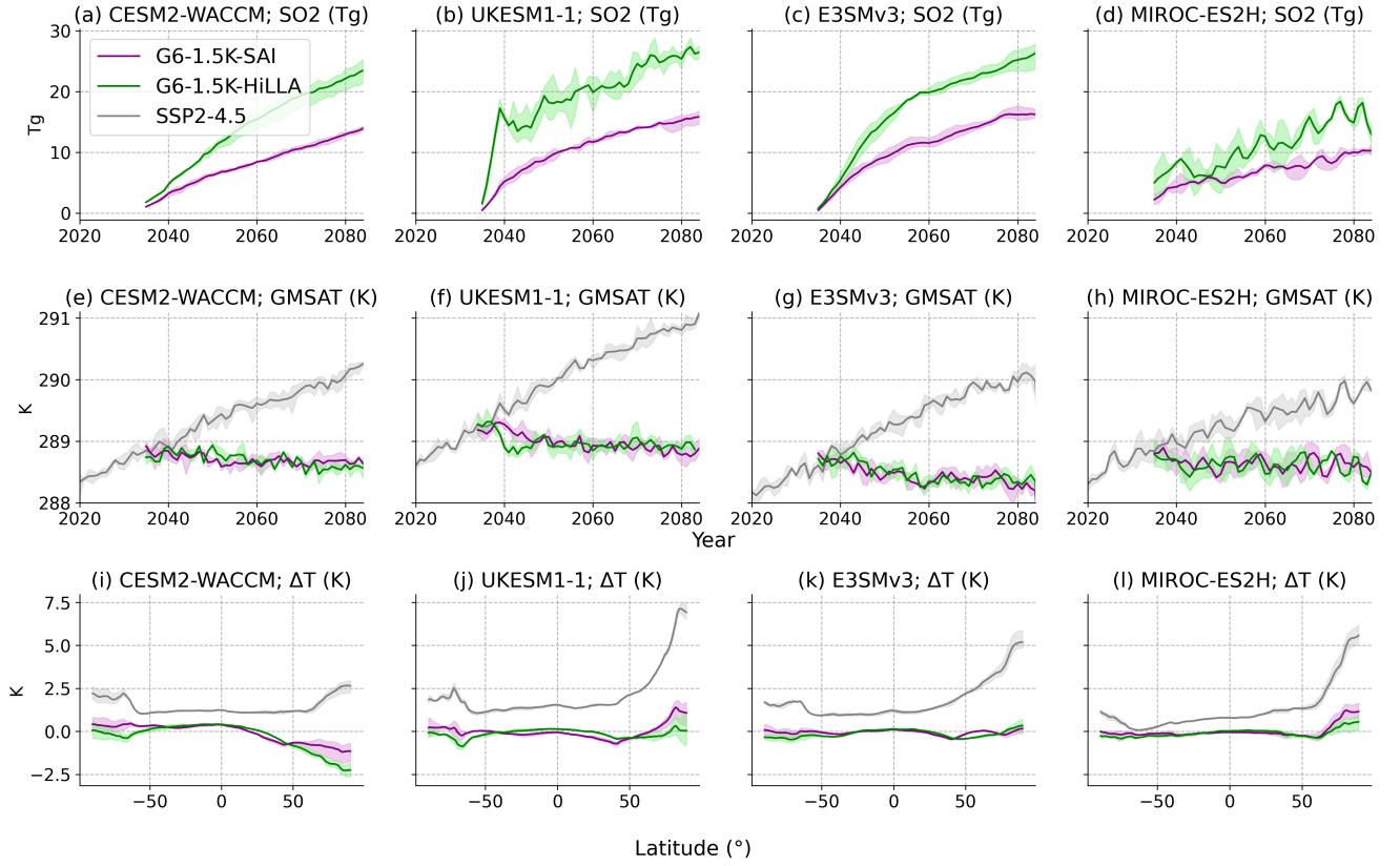
Figure 3. (a-d) Injection magnitude ( T_g SO 2 ), (e-h) Global mean surface air temperature (GMSAT), and (i-l) zonal mean temperature change relative to the 2020-2039 baseline ( \Delta T ), for the four models with G6-1.5K-SAI and G6-1.5K-HiLLA simulations. The solid lines show ensemble means and shaded areas show ensemble range, using the first three members for all scenarios.
