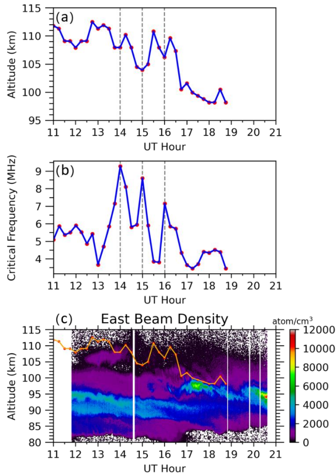
Figure 6. (a) Height and (b) critical frequency of the Es layer measured by the Wuhan ionosonde between 11:00 and 21:00 UT on 13 June 2013. Red dots indicate individual measurements. (c) Height variation of the Es layer (orange line) overlaid on the time–height contour of sodium density from the east beam. The dashed lines in (a) and (b) indicate gravity-wave perturbations in the Es layer.
