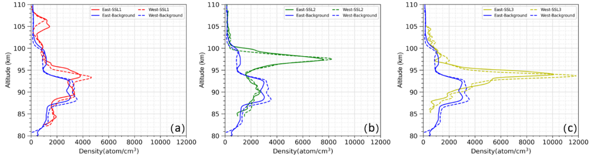
Figure 2. Maximum sodium density profiles of the SSL1 (a), SSL2 (b), and SSL3 (c) compared with the background sodium density. The solid line represents the east beam and the dashed line represents the west beam. SSL1, SSL2, SSL3 and background sodium density are plotted in red, green, yellow, and blue respectively.
