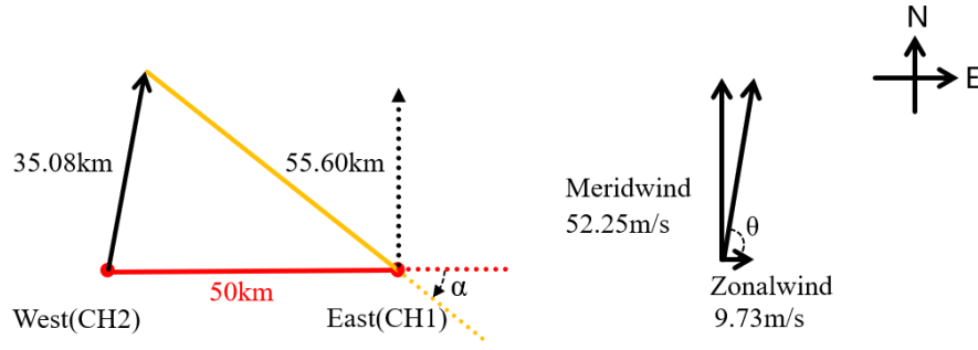
Figure 7. Schematic diagram of the SSL3 event. The red line indicates a 50 km separation between the two beams in the mesopause region. The solid black line represents the horizontal wind vector, and the yellow line represents the horizontal extent of the SSL.
