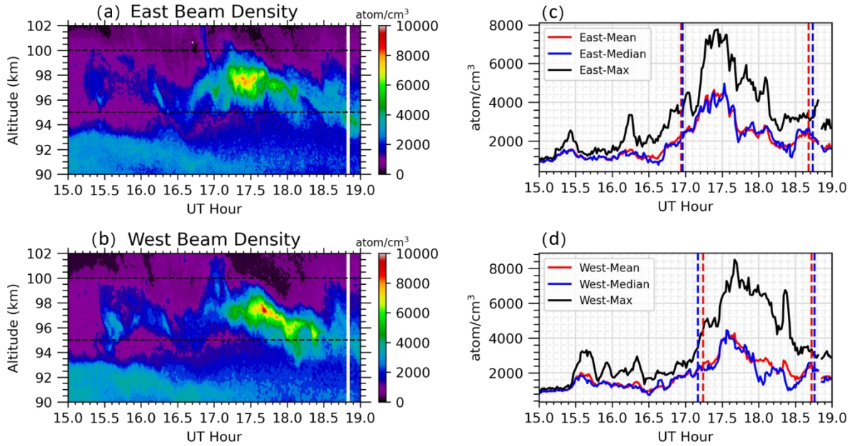
150 Figure 4. Time–height contours of SSL2 observed from the east beam (a) and west beam (b). Panels (c) and (d) show the corresponding time variations of sodium density within the altitude range of 95–100 km for the two beams. Red, blue, and black solid lines represent the mean, median, and maximum sodium densities, respectively. Vertical red and blue dashed lines indicate the onset and end times derived from mean and median sodium densities, defined as twice the background level.
