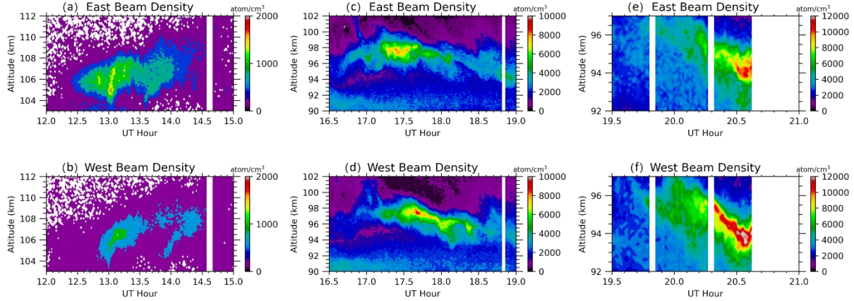
135 Figure 3. Time–height contours of SSL1 (a, b), SSL2 (c, d), and SSL3 (e, f). The upper panels show results from the east beam, and the lower panels show results from the west beam.
