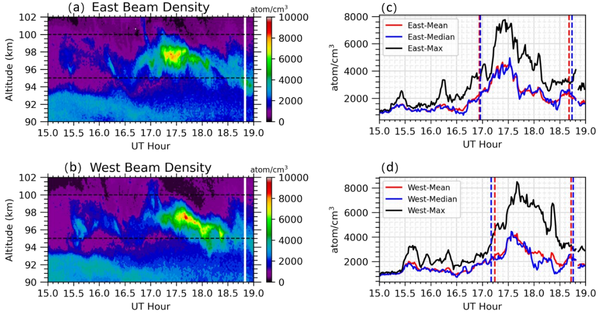
150 Figure 4. Time–height contours of SSL2 observed from the east beam (a) and west beam (b). Panels (c) and (d) show the | corresponding time variations of sodium density within the altitude range of 95–100 km height for the two beams. Red, blue, | and black solid lines represent the mean, median, and maximum sodium densities, respectively. Vertical red and blue dashed lines | indicate the onset and end times derived from mean and median sodium densities, defined as twice the background level.
