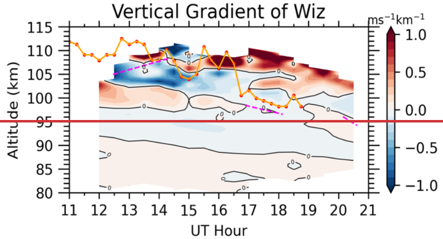
295 Figure 10. Time–height contour of vertical gradient of ion vertical drift derived from zonal wind measured by the USTC sodium lidar on 13 June 2013. Cold colors indicate negative dw_{iz}/dz (ion convergence region), while warm colors indicate positive dw_{iz}/dz (ion divergence region). The orange line denotes the altitude variation of the Es layer measured by the Wuhan ionosondes, and the dashed purple lines indicate the trajectories of the SSLs.
