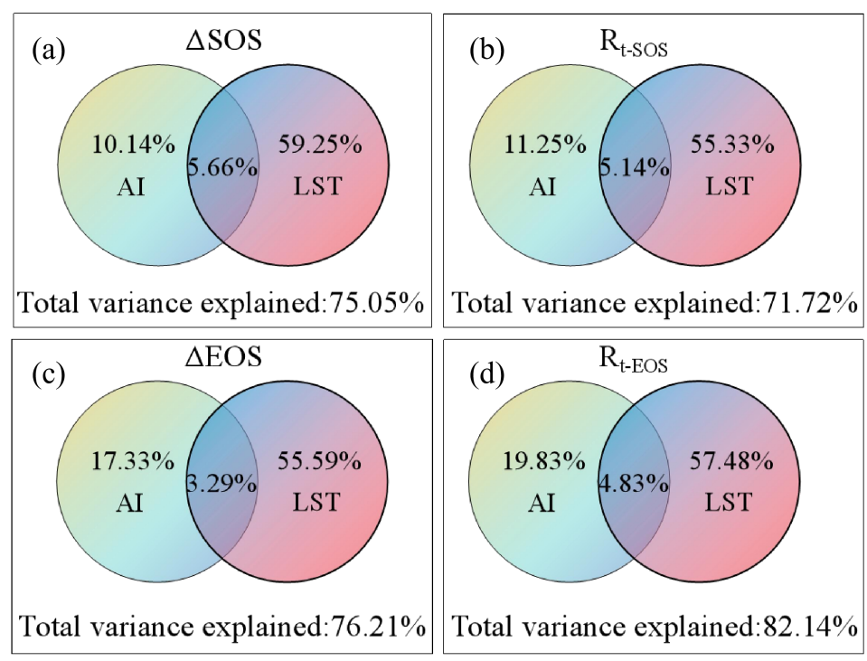
Figure 10. Venn diagrams illustrating the relative contributions of AI and LST to \Delta SOS, \Delta EOS, R_{t-SOS} , and R_{t-EOS} across 293 Chinese cities. Note: Values in each section represent the percentage of variance independently explained by AI or LST and their shared explanatory power in the overlapping region, and the total variance explained by both factors is labeled below each panel.
