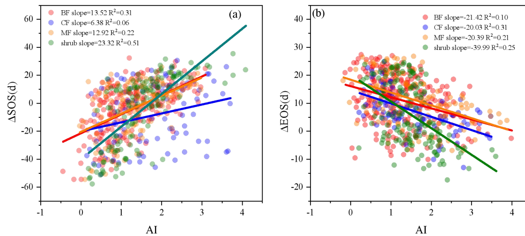
Figure 9. Relationships between AI and urban-rural phenological differences ( \Delta\text{SOS} , \Delta\text{EOS} ) across different vegetation types. Panel (a): Scatter plot of \Delta\text{SOS} versus AI with linear regression fits for each vegetation type. Panel (b): Scatter plot of \Delta\text{EOS} versus AI with linear regression fits for each vegetation type.
