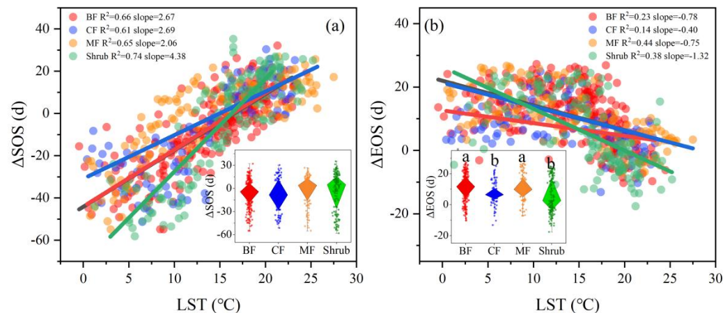
Figure 6. Relationships between LST and \Delta SOS/ \Delta EOS across the 293 cities for four vegetation types. The inset subplots compare the mean phenological differences among vegetation groups. BF: Broad-leaf forest, CF: Coniferous forest, MF: Mixed forest, Shrubs: Shrublands .
