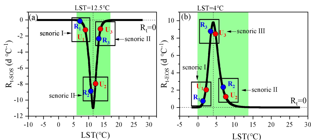
Figure 7. Schematic diagram of the three scenarios that likely occurred in urban (red dots) and rural (blue dots) regions for SOS (I: LST_{R1} < LST_{U1} < 12.5\text{ }^{\circ}\text{C} ; II: 12.5\text{ }^{\circ}\text{C} < LST_{R2} < LST_{U2} ; III: LST_{R3} < 12.5\text{ }^{\circ}\text{C} < LST_{U3} ) and EOS (I: LST_{R1} < LST_{U1} < 4\text{ }^{\circ}\text{C} ; II: 4\text{ }^{\circ}\text{C} < LST_{R2} < LST_{U2} ; III: LST_{R3} < 4\text{ }^{\circ}\text{C} < LST_{U3} ).
