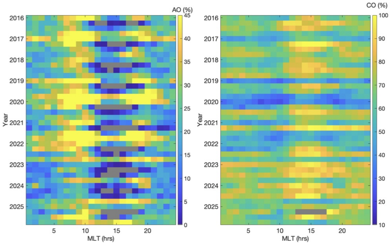
Figure 9. AO (left) and CO (right) as a function of month and MLT for the entire dataset, 2016–2025. The bin size is an hour. Months of Jan–Feb and Nov–Dec are included for all years. The data are normalised to the total number of images per bin. The gray colour marks the empty bins.
