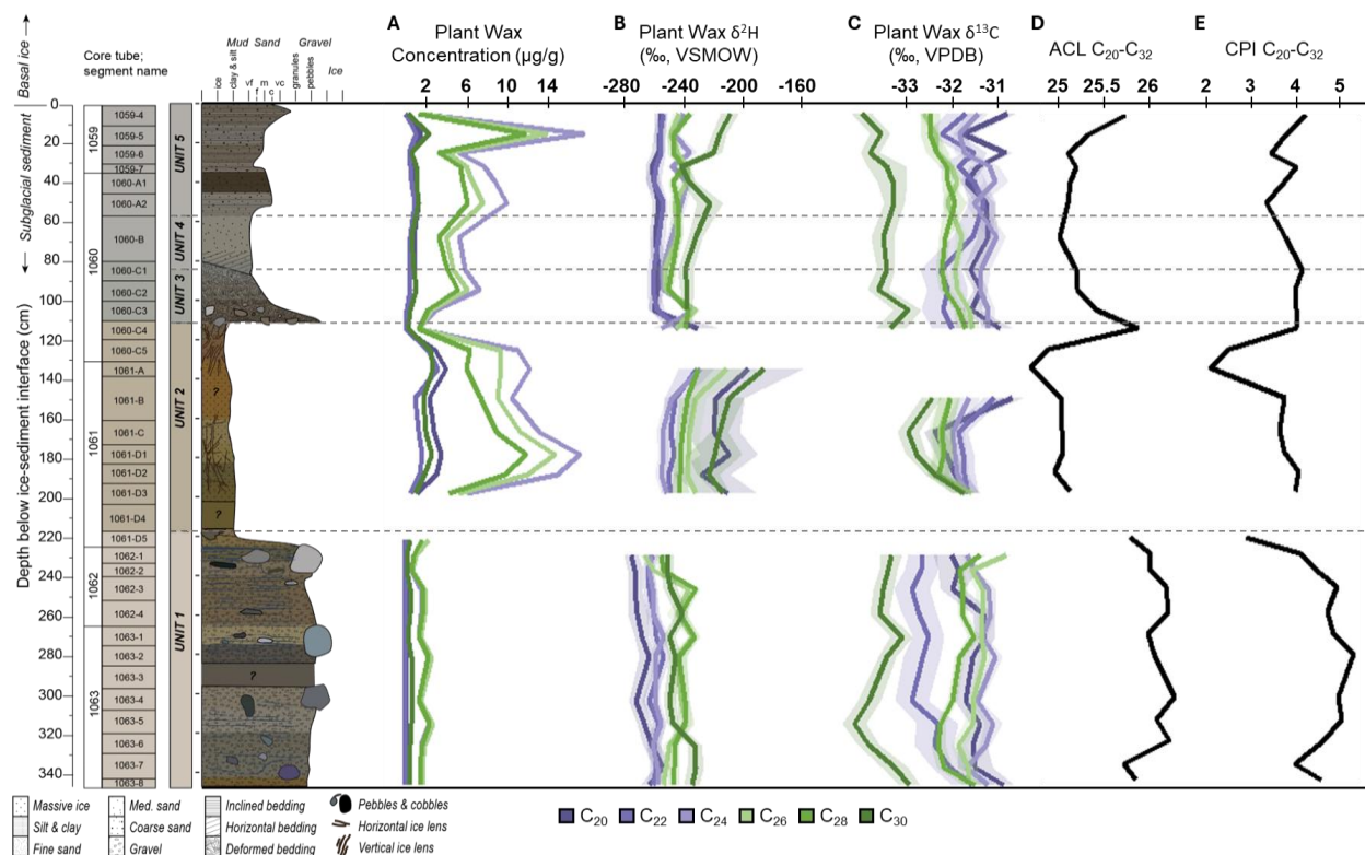
Figure S6. Down core plant wax data from Camp Century, northwestern Greenland. (A) Concentration of C 20 to C 30 n -alkanoic acids. (B–C) \delta^{13}\text{C} and \delta^2\text{H} of C 20 to C 30 n -alkanoic acids. (D) Average chain length (ACL) of even-chain n -alkanoic acids (C 20 –C 32 ). (E) Carbon preference index (CPI) for n -alkanoic acids (C 20 –C 32 ). Shading in B and C is the total uncertainty associated with the measured \delta^2\text{H} and \delta^{13}\text{C} values is the standard error of the mean (SEM), which includes the uncertainty in the peak-size and drift corrections, the replicate variability, and the methyl group correction.
