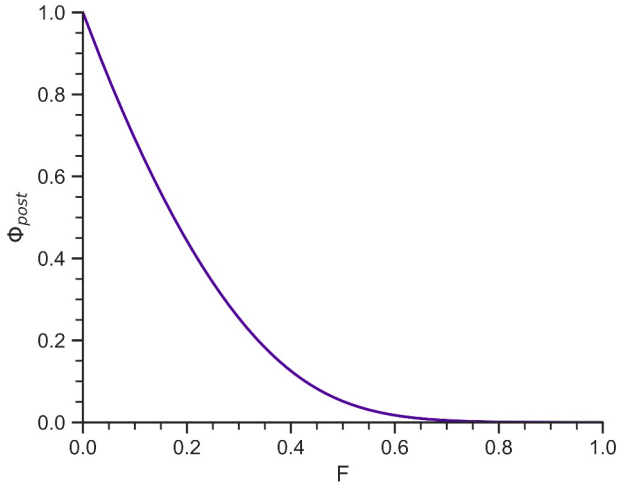
Figure A1: Relationship between the post-depositional He retention \phi_{post} and the normalized step length F .
