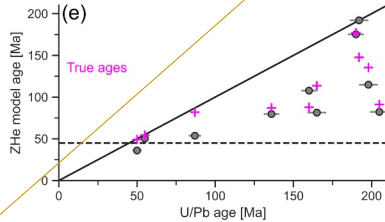
Figure 4: Overview of partial-reset-modeling strategies applied to a synthetic zircon U/Pb–(U–Th)/He dataset. All information on this dataset is provided at the top panel. (a) True temperature–time (T–t) paths for each grain. The grey shaded area marks the zircon (U–Th)/He (ZHe) partial-retention zone (grain-size of the synthetic grains; kinetic parameters of Reiners et al., 2004) and (b) ZHe–U/Pb age–age plot. The panels below show the three different interpretation strategies of Reiners et al. (2005; c–e), Fosdick et al. (2015; f–h) and this study (i–k), each in three analytical steps. Detailed description of the specific steps for each strategy in the text.
