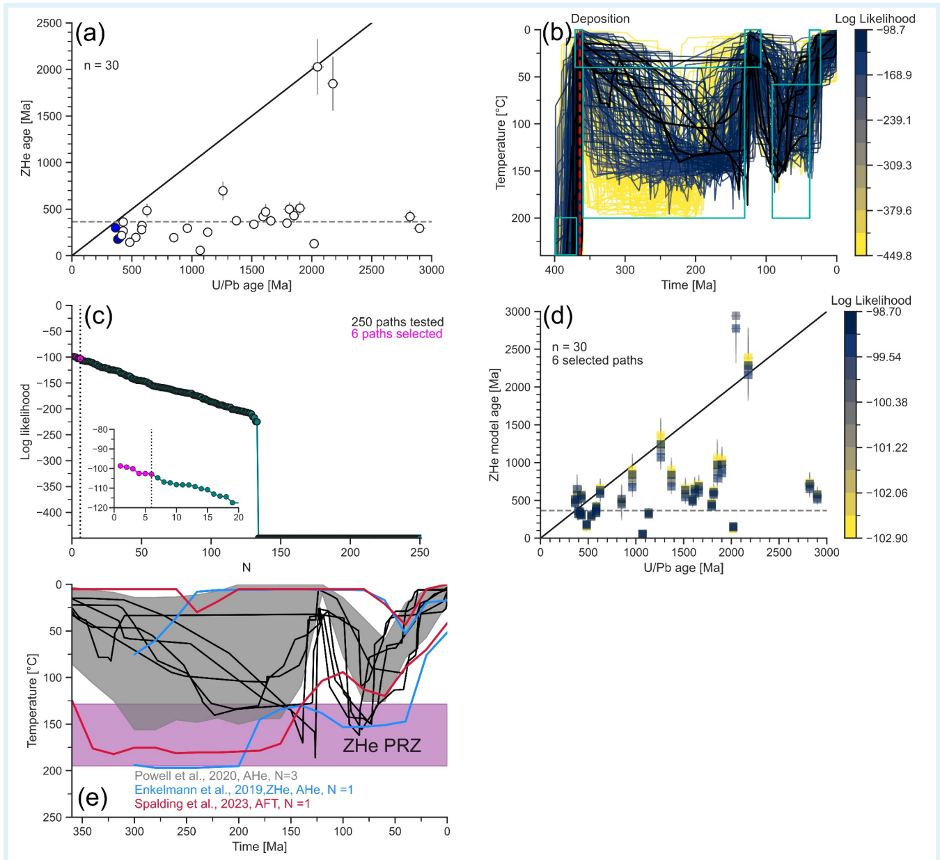
Figure 3: Zircon U/Pb-(U-Th)/He (ZHe) data and modeling results for an Imperial Formation sandstone from the Northern Canadian Cordillera. (a) Plot of measured ZHe age (corrected for \alpha -ejection; see Härtel et al., 2026) vs. U/Pb concordia ages with equal-age (solid), and depositional-age (dashed) lines. Blue symbols: syn-depositional grains. Bars show 2s uncertainties. (b)
