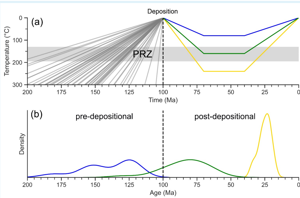
Figure 1: Schematic thermal histories and single-grain age distributions of unreset (blue), partially reset (green), and fully reset (yellow) sedimentary samples in the zircon (U-Th)/He (ZHe) system. (a) Example thermal histories for detrital grains with pre-depositional (grey) temperature-time (T-t) paths that represent simplified cooling paths for each grain and shared post-depositional paths (colored). The grey shaded area marks the partial retention zone (PRZ; kinetics of Reiners et al., 2004, for non-metamict zircon grains with equivalent spherical radii of 20–90 \mu\text{m} and 30 Myr holding time). (b) Kernel-density estimate (KDE) curves for synthetic age distributions reflecting the thermal histories in (a).
