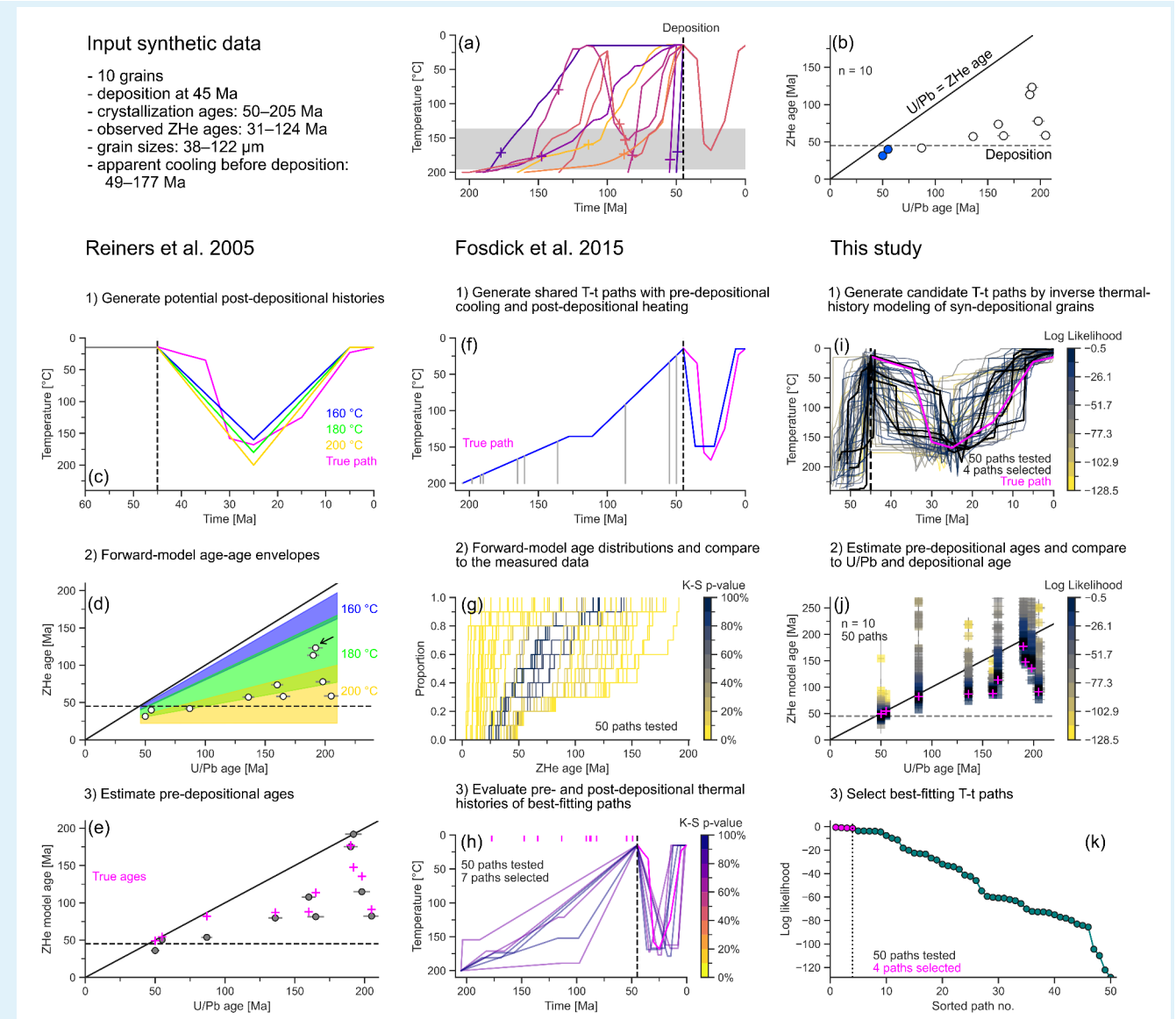
Figure 3: Overview of partial-reset-modeling strategies applied to a synthetic zircon U/Pb-(U-Th)/He dataset. All information on
