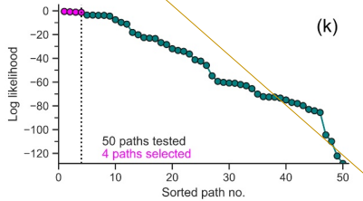
Figure 4: Overview of partial-reset-modeling strategies applied to a synthetic zircon U/Pb–(U–Th)/He dataset. All information on this dataset is provided at the top panel. (a) True temperature–time (T–t) paths for each grain. The grey shaded area marks the zircon (U–Th)/He (ZHe) partial-retention zone (grain-size of the synthetic grains; kinetic parameters of Reiners et al., 2004) and (b) ZHe–U/Pb age–age plot. The panels below show the three different interpretation strategies of Reiners et al. (2005; c–e), Fosdick et al. (2015; f–h) and this study (i–k), each in three analytical steps. Detailed description of the specific steps for each strategy in the text.
