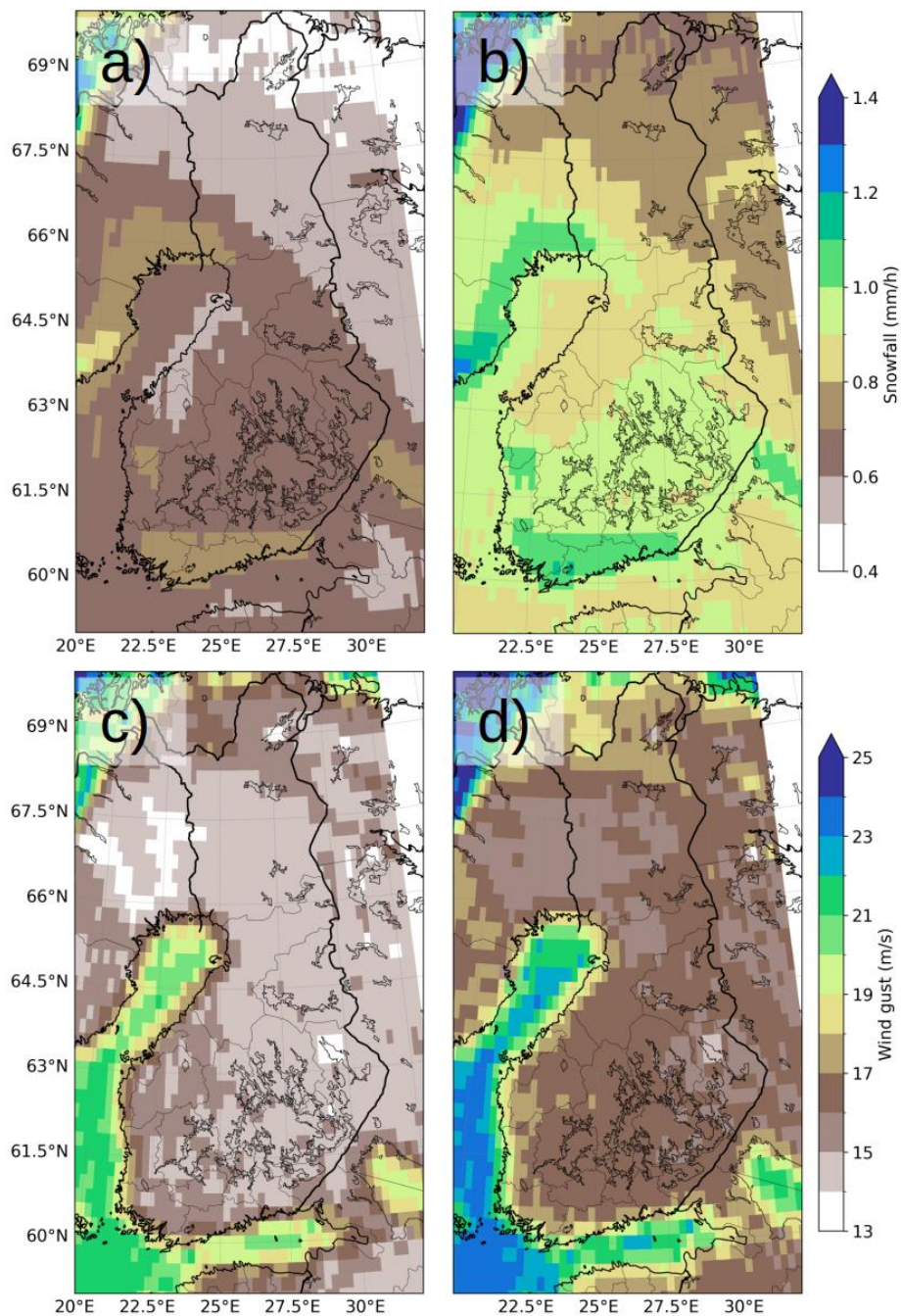
590 Appendix D1. Average hourly snowfall (a and b) and wind gust (c and d) during single events when the 95 th (a and c) and 98 th (b and d) percentile was used as a threshold value from October to March in 1960-2024 based on ERA5.
