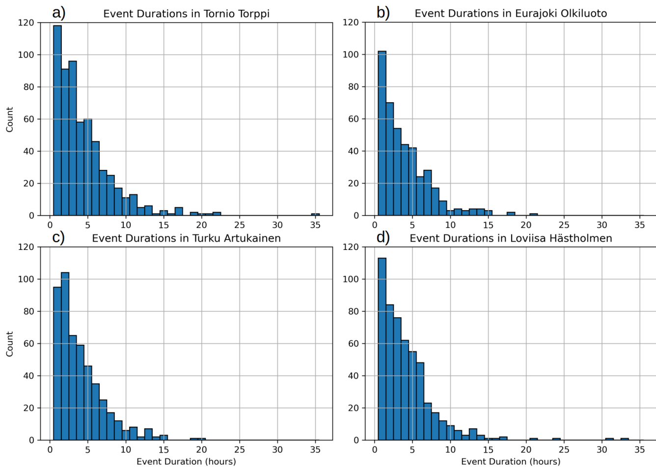
580 Appendix B1. Histograms of SWG compound event's durations in Tornio Torppi (a), Eurajoki Olkiluoto (b), Turku Artukainen (c) and Loviisa Hästholmen (d) for the threshold value of 95 th percentile. Histograms show the number of consecutive hours when snowfall and wind gust exceeded their threshold value simultaneously during October-March 1960-2024 based on ERA5.
