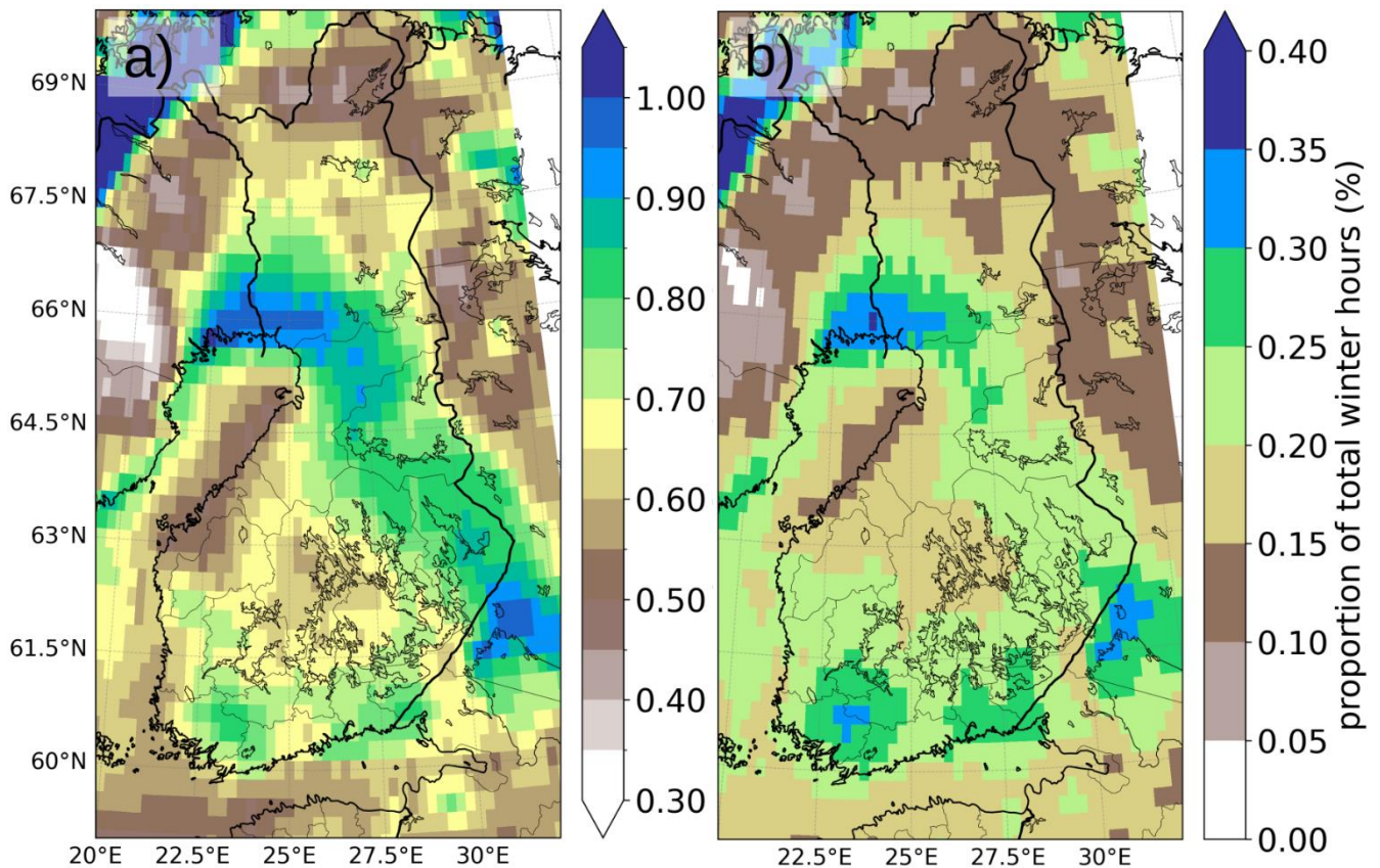
Figure 3. Proportion of total winter hours when co-occurring hourly snowfall and wind gust (SWG) exceeded their 95 th (a) and 98 th (b) percentiles from October to March in 1960-2024 based on ERA5. Note the different scaling in colorbars.
