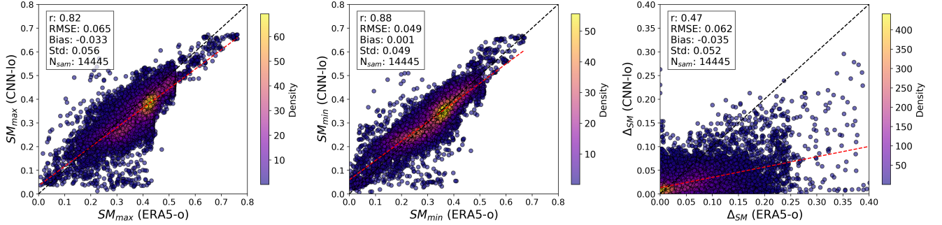
Figure 8. Scatter plots comparing CNN-lo and ERA5-o SM for days with isolated precipitation events ( p_t > 10 mm and p_{t-1} = 0 mm) in 2019. Panels show: (1) maximum SM value ( SM_{max} ); (2) minimum SM value ( SM_{min} ); and (3) the resulting diurnal SM amplitude ( \Delta_{SM} = SM_{max} - SM_{min} ), all in m^3 m^{-3} . Each point represents one pixel-day. Statistical metrics include total correlation ( r ), root mean square error (RMSE, m^3 m^{-3} ), bias (Bias, m^3 m^{-3} ), standard deviation (Std, m^3 m^{-3} ), and number of samples ( N_{samples} ). The dashed black line represents the 1:1 line; the red dashed line is the linear regression fit. The colorbar indicates the local density of dots in the scatterplot.
