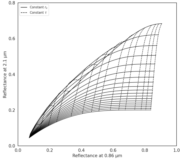
Figure 2. Nakajima-King retrieval grid representing the central operational assumption ( v_{\text{eff}} = 0.10 ), evaluated at \text{SZA} = 40^\circ , \text{VZA} = 0^\circ , \text{RAZ} = 0^\circ . The grid maps the top-of-atmosphere reflectances at 0.86 \mu\text{m} and 2.1 \mu\text{m} to a unique solution for \tau (dashed lines) and r_e (solid lines).
