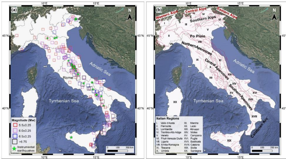
Figure 1 (a) Selected dataset of 191 earthquakes with M_w \geq 5.5 from the CPTI15 catalogue (Rovida et al., 2022). Square colours and sizes are proportional to the earthquake magnitude estimate. Starred events. Green stars indicate the subset of 24 earthquakes for which instrumental solutions are available. (b) Map of the main physiographic structures and tectonic lineaments of Italy (Bigi et al., 1989) cited in the catalogue text. Roman numerals (I to XX) refer to the Italian administrative regions with the names detailed in the legend. Basemap source: Google Satellite imagery. Map data ©2015 Google.
