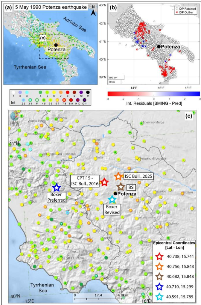
Figure 2 The May 5, 1990 (Mw 5.8 - GCMT) Potenza earthquake. (a) Macroseismic intensity distribution provided by DBMI15 (Locati et al., 2022) and derived from of the BMING dataset (Bollettino Macrosismico ING (BMING-), from Gasparini et al., (1991b). (b) Intensity residuals (blue = positive; red = negative) between BMING observations and predictions from the IPE of Gomez-Capera et al. (2024). Crosses indicate the 116 IDPs identified as outliers by the pre-processing procedure. (c) Comparison of epicentral locations: the red, orange, and brown star represents the reference instrumental location epicentral solutions from CPTI15 (International Seismological Centre, ISC Bulletin, 2016); the orange star indicates the updated ISC solution (ISC Bulletin, 2025); the brown star represents the instrumental location from BSI; the blue star indicates the (2025), and BSI, respectively. Blue and light blue stars indicate the macroseismic epicentres derived with Boxer solution derived from the preferred (BMING) and revised macroseismic field; the light blue star represents the Boxer epicentre obtained from the revised field. The map sources: Maps in panels (a) and (c) are derived from the CPTI15-DBMI15 catalogue (Locati et al., 2022; Rovida et al., 2022), which uses the NASA SRTM30 PLUS Digital Elevation Model ( https://www.earthdata.nasa.gov/data/instruments/srtm ) as background.
