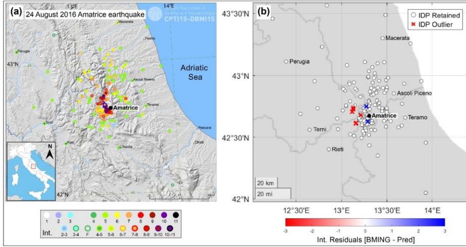
Figure 3 The August 24, 2016 (Mw 6.18) Amatrice earthquake. (a) Macroseismic intensity distribution provided by DBMI15 (Locati et al., 2022) and derived from of the ROSAL019 dataset, from Rossi et al. (2019; ROSAL019). (b) Intensity residuals (blue = positive; red = negative) between ROSAL019 observations and values predicted predictions from the adopted IPE. Blue crosses of Gomez-Capera et al. (2024). Crosses indicate the 8 IDPs identified as intensity outliers by the pre-processing procedure and removed from the analysis. Blue crosses highlight the localities of with positive residuals (Pescara del Tronto and Amatrice, I = 10 ), whereas red crosses indicate the sites of outliers with negative residuals (Terracina, I = 5-6 ; Castel S. Maria, Cittareale, Savelli, and Valcardara, I = 5 ). The map source in panel (a) is the derived from CPTI15-DBMI15 catalogue (Locati et al., 2022; Rovida et al., 2022), which and uses the NASA SRTM Digital Elevation Model ( https://www.earthdata.nasa.gov/data/instruments/srtm/ ) ITALY DEM as background.
