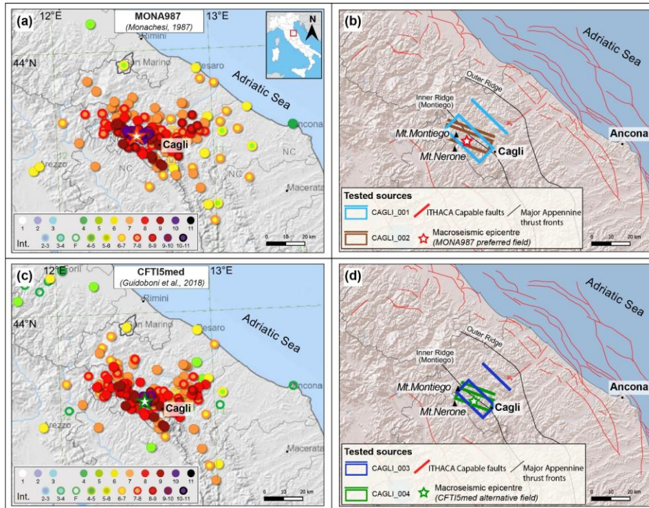
Figure 8 The June 3, 1781 Cagli earthquake. (a) Macroseismic intensity distribution from the MONA987 dataset (from Monachesi, 1987). (b) Tested source configurations (CAGLI_001 and CAGLI_002). (c) Macroseismic intensity distribution from the CFTI5med dataset (from Guidoboni et al., 2018). (d) Tested source configurations (CAGLI_003 and CAGLI_004). Red lines represent capable faults from the ITHACA database (ITHACA Working Group, 2019), while black lines indicate the main frontal thrusts of the Apennines, including the Montegio thrust cited in the text. Red and green stars indicate represent the macroseismic epicentres derived from MONA987 and CFTI5med datasets, respectively. The map sources in panels (a) and (c) is derived from the CPTI15-DBMI15 catalogue (Locati et al., 2022; Rovida et al., 2022), which uses the NASA SRTM Digital Elevation Model ( https://www.earthdata.nasa.gov/data/instruments/srtm ) as background. The maps in ITALY DEM, whereas panels (b) and (d) are generated using the Esri Shaded Relief basemap. Sources: Esri | Powered by Esri.
