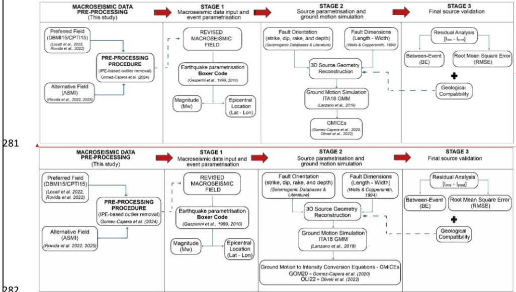
Figure 4 Schematic representation of the integrated workflow adopted for seismogenic source reconstruction, including the macroseismic data pre-processing step. The dashed blue arrows illustrate how the output of the pre-processing (i.e. indicate that the revised macroseismic field serves as the primary input to Stage 1, and how while the results from Stage 3 are used to iteratively used to validate and refine the 3D source geometry. Notes: GMM, Ground Motion Model; GMICES, Ground Motion to Intensity
