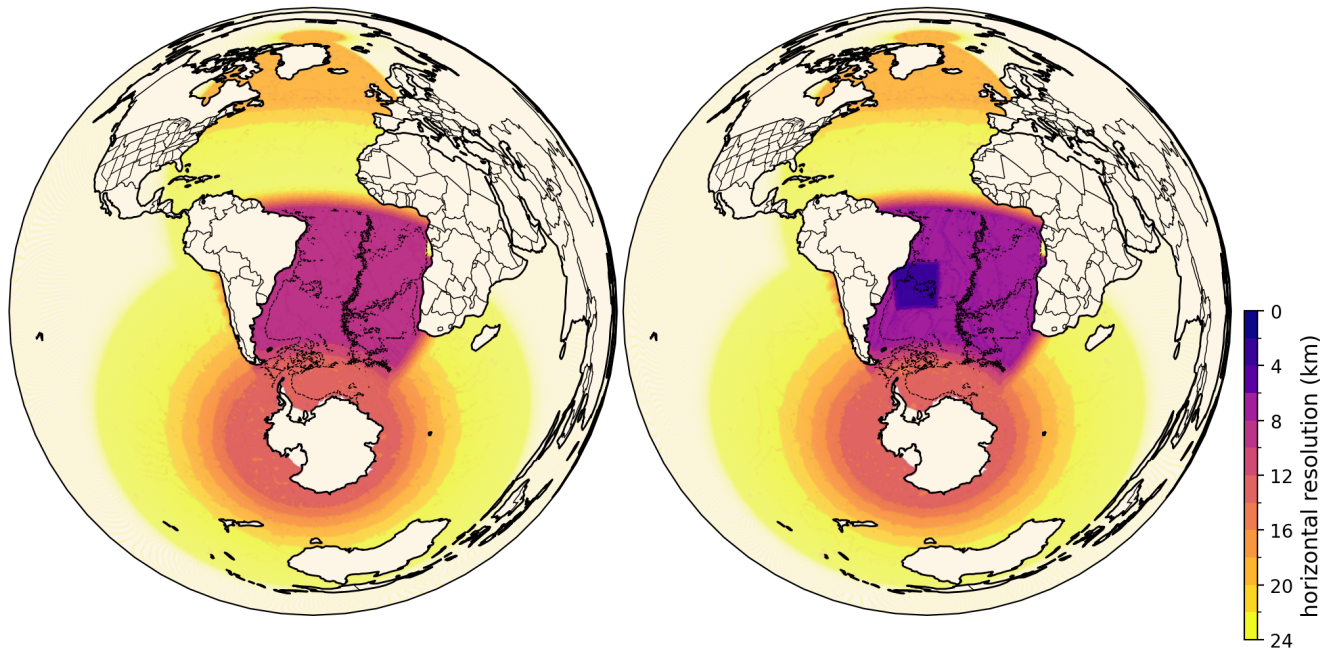
Figure A2. Panel a) Square root of grid-cell area (FESOM R and FESOM V) of the entire globe. Panel b) Same as panel a, but of FESOM H and FESOM VH. Dashed black contour marks the isobath of 3000 m and solid black contour the continents.
