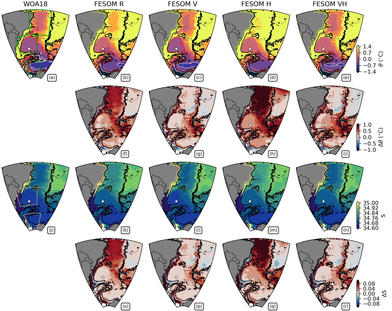
Figure 7. Mean potential temperature ( \theta ; panels a–e) and salinity (panels j–n) from 1994 to 2005 at the deepest valid level at each horizontal grid point, and the corresponding mean biases relative to WOA18 ( \Delta\theta , panels f–i; \Delta S , panels o–r). Columns correspond to WOA18 (reference), FESOM R, FESOM V, FESOM H, and FESOM VH, from left to right. The black contour indicates the 3000 m isobath, the red contour marks the \theta = 0.0^\circ\text{C} isotherm, and the white contour marks the \theta = -0.7^\circ\text{C} isotherm. White diamonds mark the position of the virtual profile depicted in Figure A4. Rectangles in the WOA18 panels (a and j) represent, from north to south, the Brazil Basin, Argentine Basin, and Weddell Sea.
