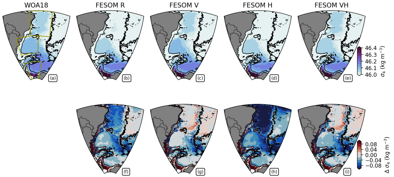
Figure A6. Mean potential density referenced to 4000 m ( \sigma_4 ; panels a–e) from 1994 to 2005 at the deepest valid level at each horizontal grid point, and the corresponding mean biases relative to WOA18 ( \Delta\sigma_4 , panels f–i). Columns correspond to WOA18 (reference), FESOM R, FESOM V, FESOM H, and FESOM VH, from left to right. The black contour indicates the 3000 m isobath. Rectangles in the WOA18 panel (a) represent, from north to south, the Brazil Basin, Argentine Basin, and Weddell Sea.
