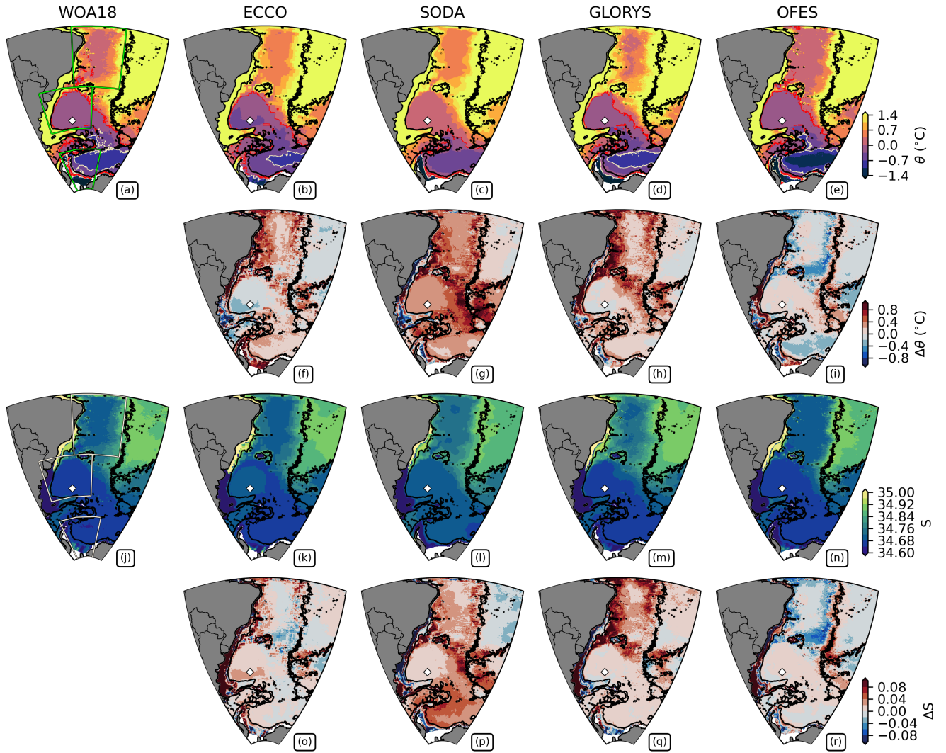
Figure 2. Mean potential temperature ( \theta ; panels a–e) and salinity (panels j–n) from 1994 to 2005 at the deepest valid level at each horizontal grid point, and the corresponding mean biases relative to WOA18 ( \Delta\theta , panels f–i; \Delta S , panels o–r). Columns correspond to WOA18 (reference), ECCO, SODA, GLORYS, and OFES, from left to right. The black contour indicates the 3000 m isobath, the red contour marks the \theta = 0.0^\circ\text{C} isotherm, and the white contour marks the \theta = -0.7^\circ\text{C} isotherm. White diamonds mark the position of the virtual profile depicted in Figure A4. Rectangles in the WOA18 panels (a and j) represent, from north to south, the Brazil Basin, Argentine Basin, and Weddell Sea.
