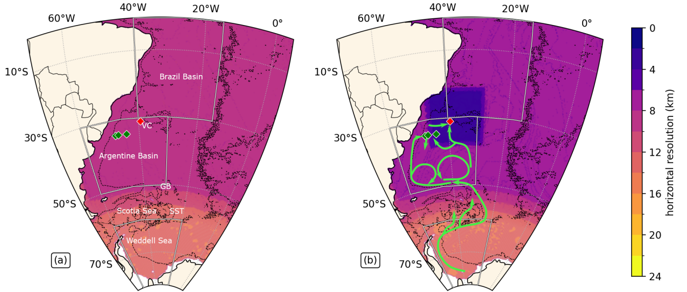
Figure 1. Panel a) Square root of grid-cell area (FESOM R and FESOM V) of the study region. Panel b) Same as panel a, but of FESOM H and FESOM VH. Green diamonds mark CTD sites BB, C, and D and red diamond marks the approximate location of the three moorings within the Vema Channel. Rectangles represent, from north to south, the Brazil and Argentine basins and the Weddell Sea, while VC marks the Vema Channel, GB the Georgia Basin, and SST the South Sandwich Trench. Dashed black contour marks the isobath of 3000 m and solid black contour the continents. Green arrows are a schematic of the main pathways of AABW.
