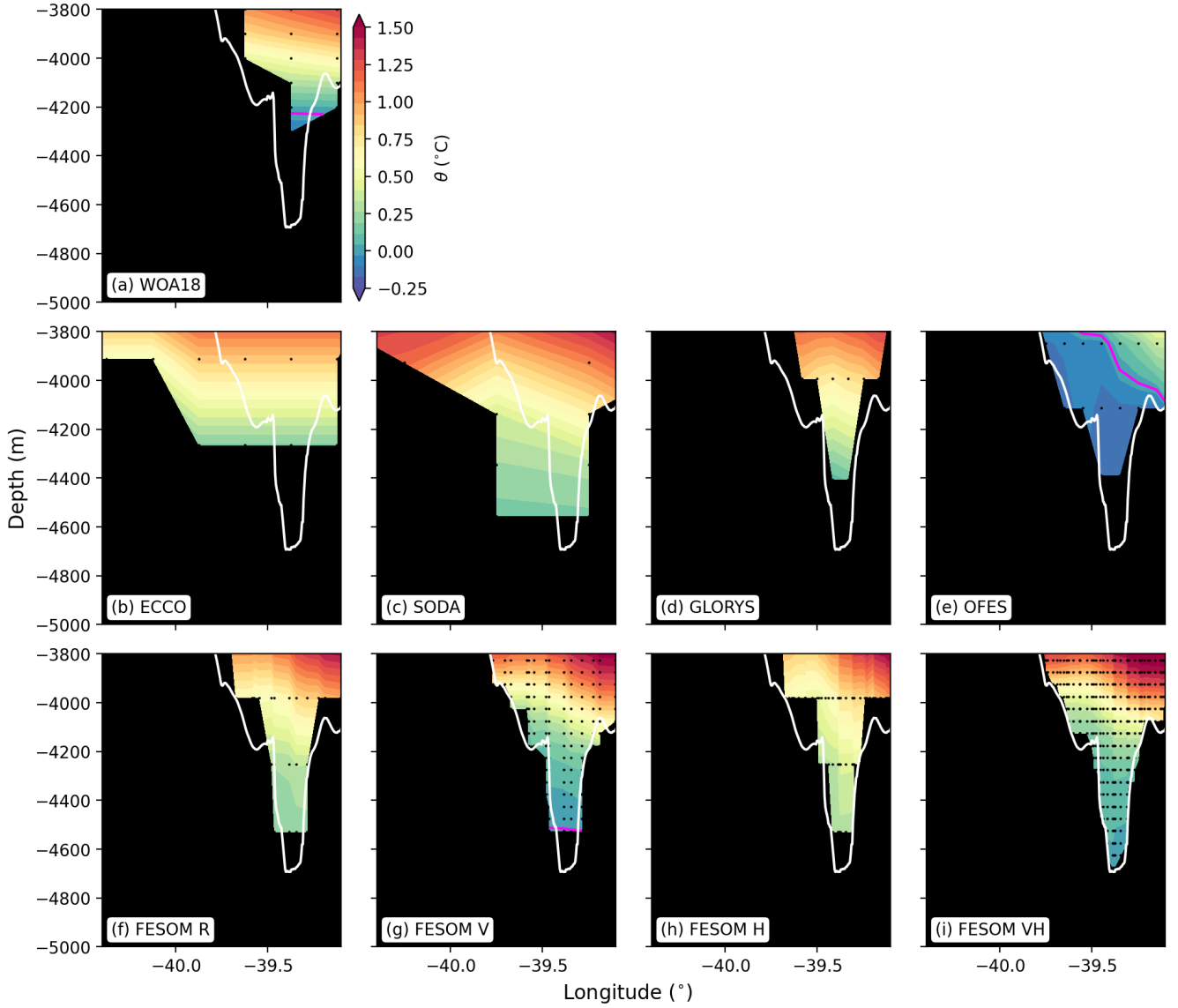
Figure 4. Time-averaged potential temperature ( \theta ) from 1995 to 2004 across Vema Channel at the nearest available latitude to 31.3^{\circ}\text{S} of: WOA18 (a), ECCO (b), SODA (c), GLORYS (d), OFES (e), FESOM R (f), FESOM V (g), FESOM H (h), and FESOM VH (i). Black dots are the grid points, white line is the bathymetry of the General Bathymetric Chart of the Oceans (GEBCO) and magenta line is the isotherm of 0.00^{\circ}\text{C} .
