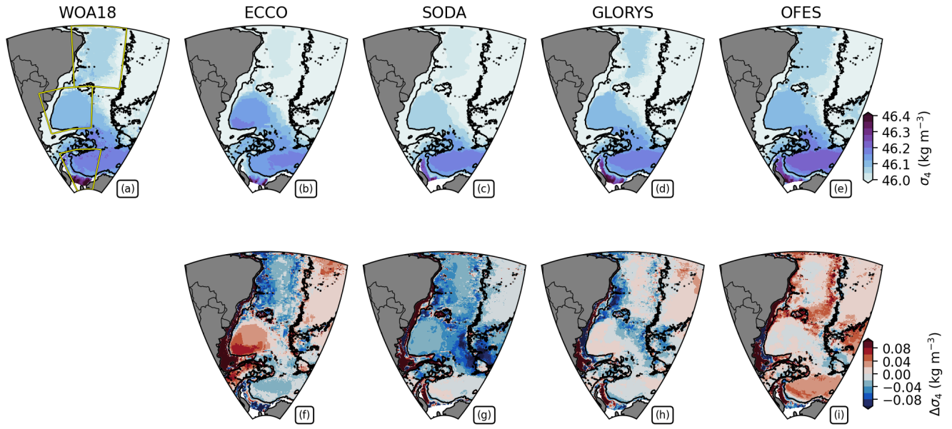
Figure A3. Mean potential density referenced to 4000 m ( \sigma_4 ; panels a–e) from 1994 to 2005 at the deepest valid level at each horizontal grid point, and the corresponding mean biases relative to WOA18 ( \Delta\sigma_4 , panels f–i). Columns correspond to WOA18 (reference), ECCO, SODA, GLORYS, and OFES, from left to right. The black contour indicates the 3000 m isobath. Rectangles in the WOA18 panel (a) represent, from north to south, the Brazil Basin, Argentine Basin, and Weddell Sea.
