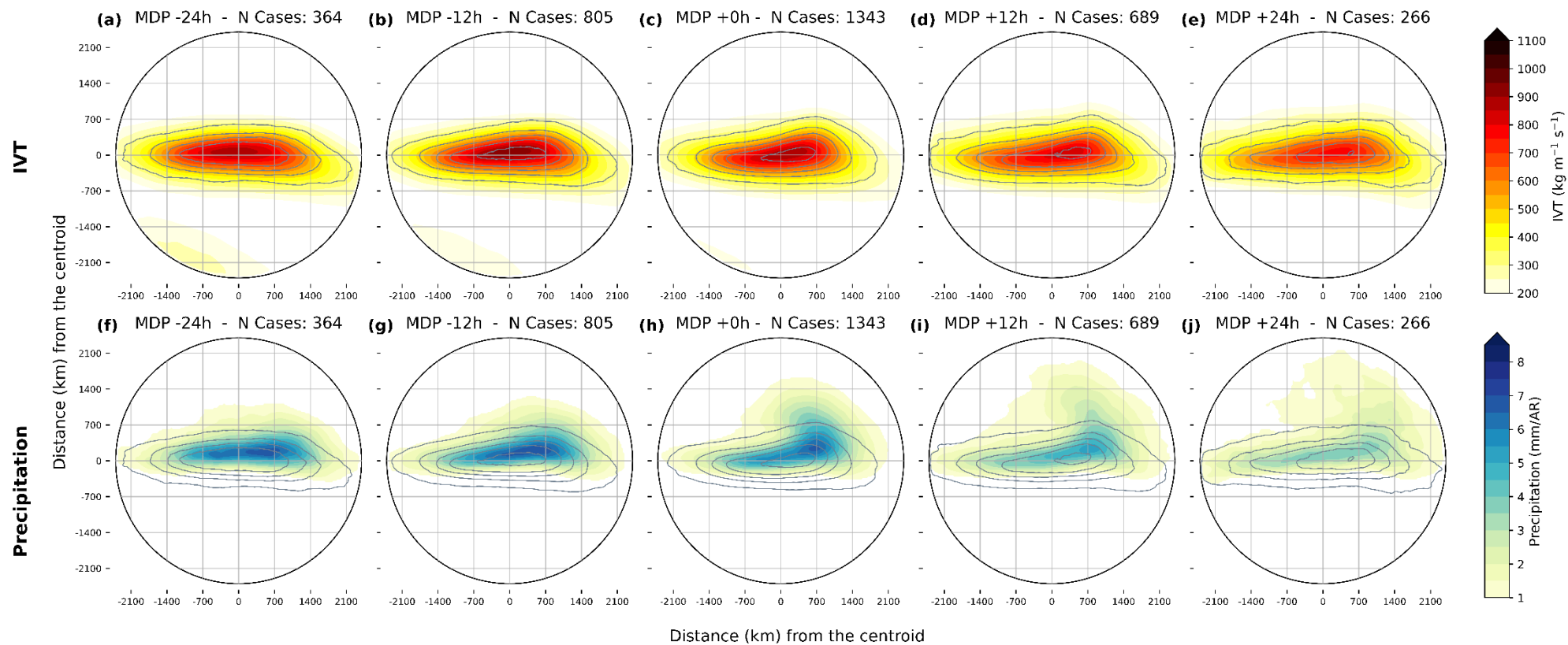
Figure 7: Temporal evolution of composites for WCB-coupled AR events, around the ETC's MDP (same timeline as Fig- 6). Top row (a-e): IVT (kg m -1 s -1 /AR). Bottom row (f-j): Total precipitation (mm/AR).
