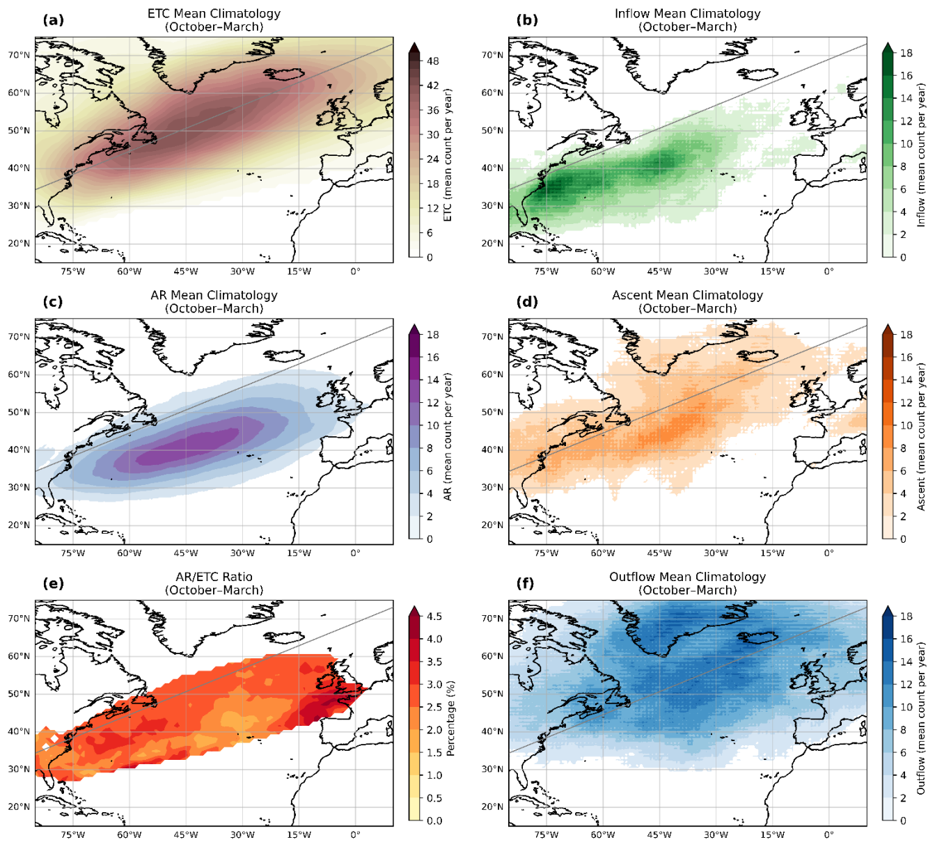
335 Figure 2: Extended winter (October-March) climatology (1979-2023) of (a) all ETCs frequency, (b) WCB inflow frequency, (c) AR frequency, (d) WCB ascent frequency, (e) AR/ETC Ratio (AR count per year / ETC count per year), and (f) WCB outflow frequency. Grey line represents the axis of the ETC climatology's distribution shown in (a), for easier orientation.
