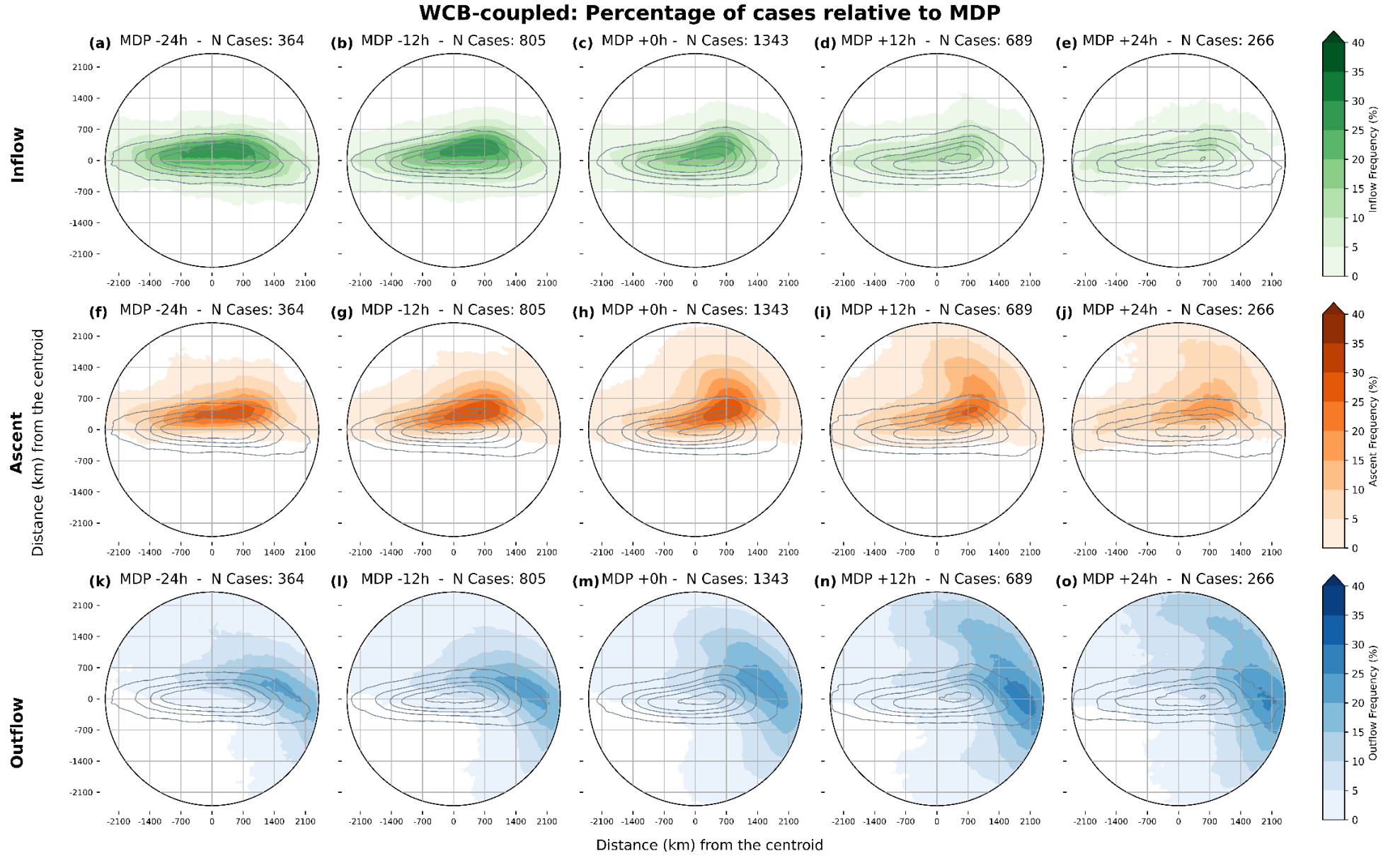
Figure 6: Temporal evolution of WCB phase frequency (%) for WCB-coupled AR events, centered on the time of the associated ETC's MDP. Rows show (a-e) WCB inflow, (f-j) WCB ascent, and (k-o) WCB outflow frequency. Rows show fields at MDP-24h, MDP-12h, MDP, MDP+12h, and MDP+24h. Grey contours represent AR relative frequency (from 10% to 90%).
