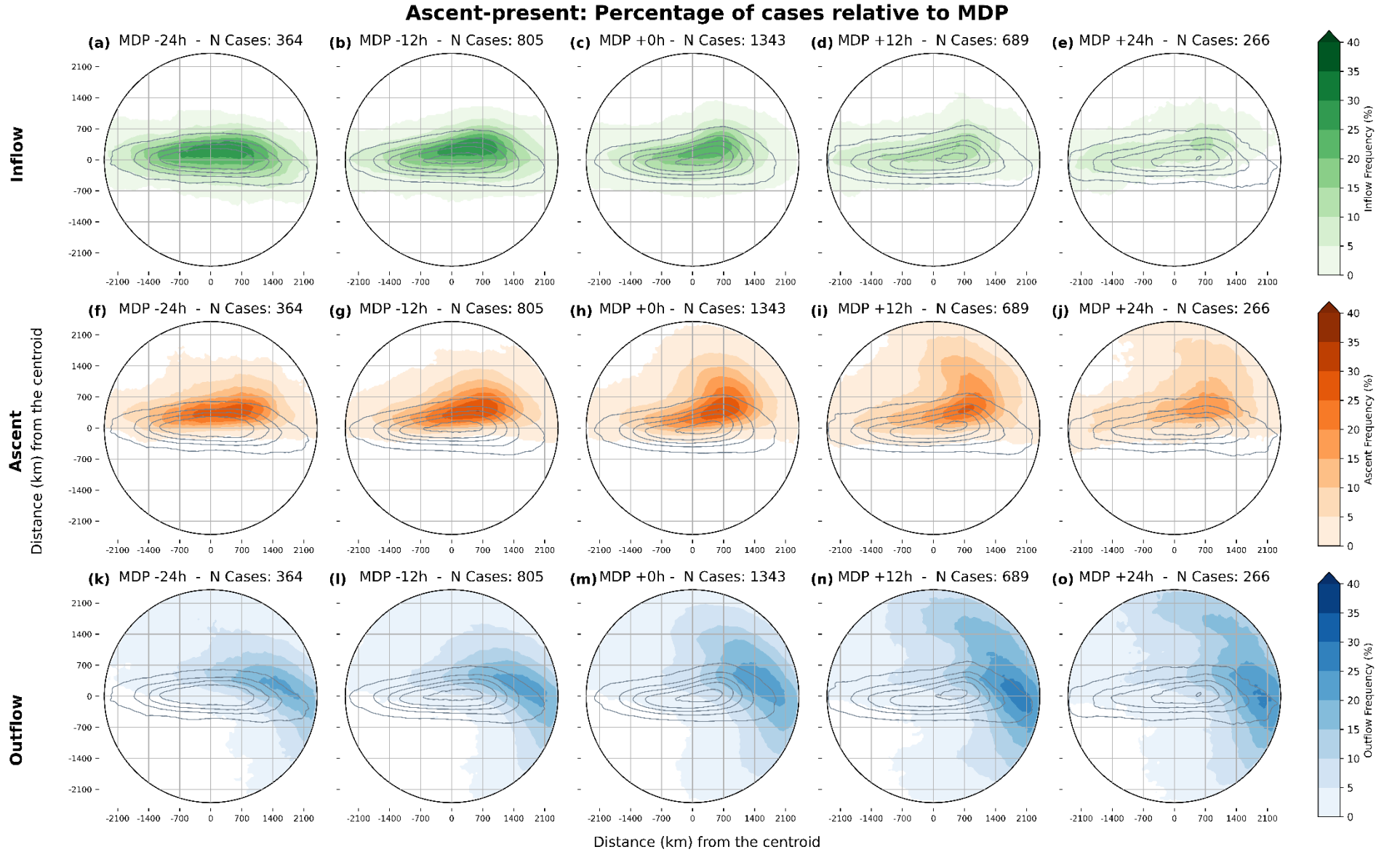
Figure 6: Temporal evolution of WCB phase frequency (%) for WCB-influenced ascent-present AR events, centered on the time of the associated ETC's MDP. Rows show (a-e) WCB inflow, (f-j) WCB ascent, and (k-o) WCB outflow frequency. Rows show fields at MDP-24h, MDP-12h, MDP, MDP+12h, and MDP+24h. Grey contours represent AR relative frequency (from 10% to 90%).
