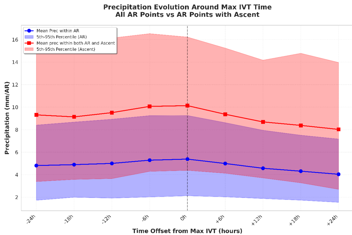
Figure 8: Precipitation change relative to the time of maximum IVT within the AR (0h). The blue line shows the mean precipitation and the blue shading represents the precipitation distribution between the 5 th and 95 th percentiles over the entire AR area, while the red line shows the mean precipitation and the red shading represents the precipitation distribution between the 5 th and 95 th percentiles over the region where the AR and the ascent overlap (i.e., the superimposed area).
