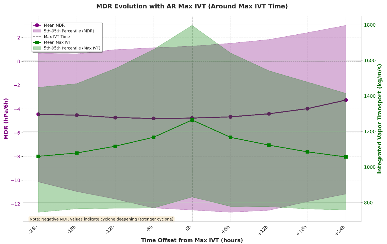
Figure 9: Evolution of IVT (green) and the associated MDP-MDR (purple) around the time of maximum IVT within the AR. The maximum IVT is defined as the highest IVT value within the AR area. MDP-The MDR is calculated for each ETC that has an associated AR. Shading colours represent the distribution of MDP-MDR (purple) and Max IVT (green) between the 5 th and 95 th percentiles.
