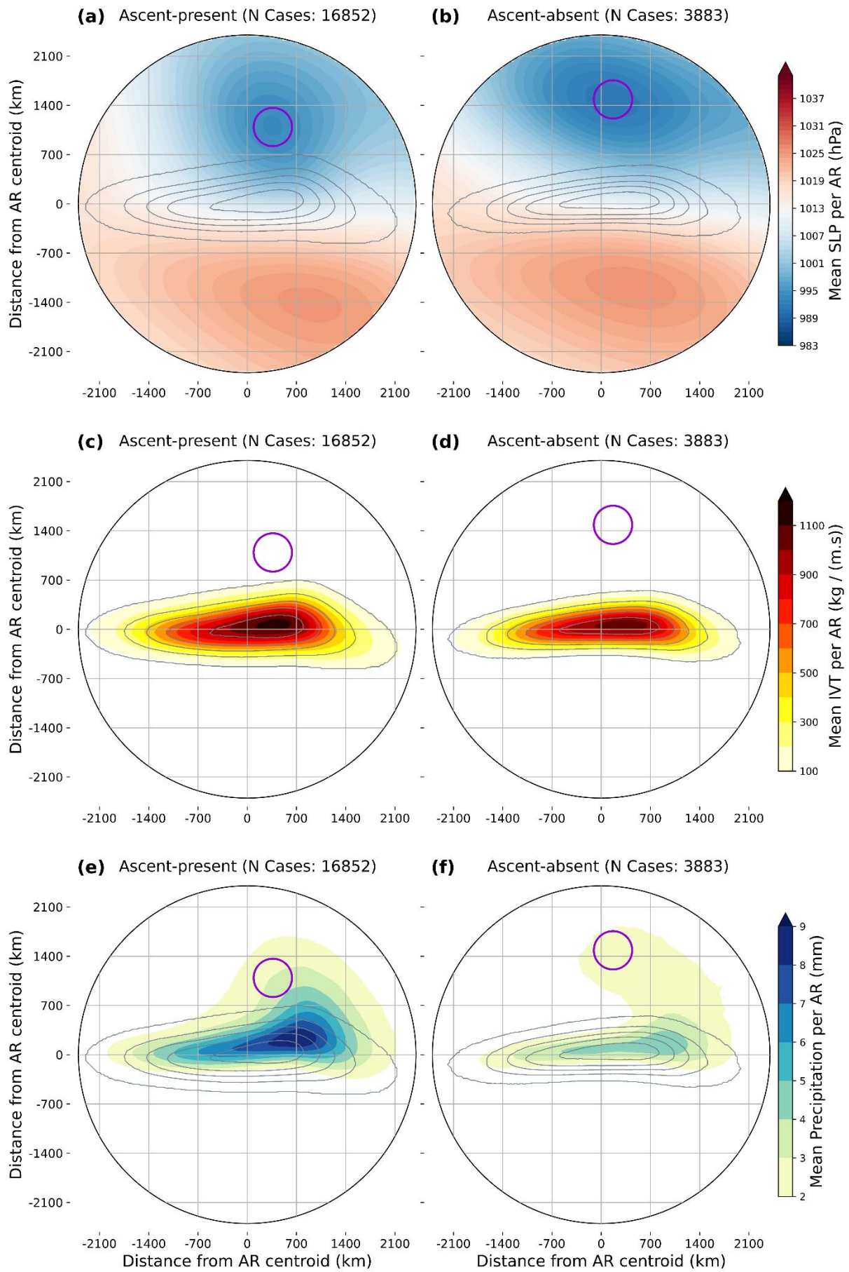
505 Figure 4: Composite fields centered on AR centroids for events with (left column) and without (right column) the WCB ascent phase: (a, b) Sea-level pressure (SLP) (hPa); (c, d) Vertically integrated water vapor transport (IVT) ( \text{kg m}^{-1} \text{s}^{-1} ); (e, f) Total precipitation (mm). Grey contours show the relative frequency of AR occurrence (10% to 90% intervals). The (0,0) point marks the AR centroid. Purple circle represents the location of the low-pressure center from the SLP composite. Grey contours show the relative frequency of AR occurrence (drawn at 20% intervals, from 10% to 90%).
