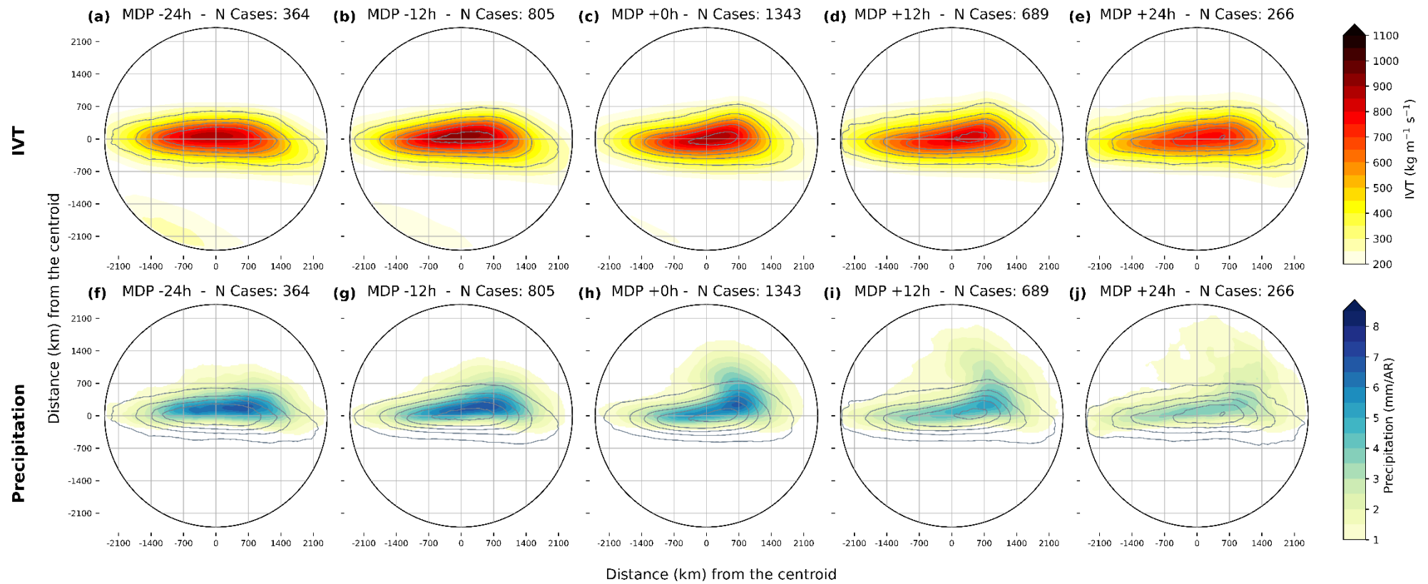
Figure 7: Temporal evolution of composites for WCB-influenced ascent-present AR events, around the ETC's MDP (same timeline as Fig- 6). Top row (a-e): IVT ( \text{kg m}^{-1} \text{s}^{-1}/\text{AR} ). Bottom row (f-j): Total precipitation ( \text{mm}/\text{AR} ).
