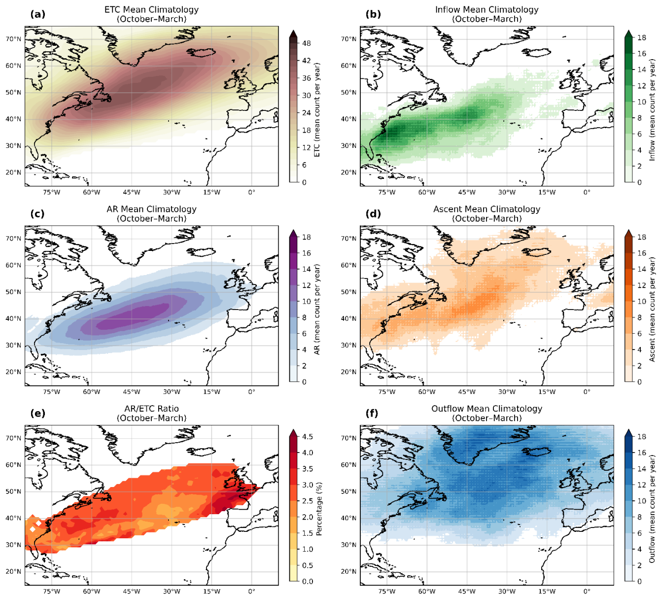
Figure 2: Extended winter (October-March) climatology (1979-2023) of (a) all Extratropical Cyclones (ETCs) frequency, (b) WCB inflow frequency, (c) Atmospheric River (AR) frequency, (d) WCB ascent frequency, (e) frequency of ETCs associated with an AR/ETC Ratio (AR count per year / ETC count per year) , and (f) WCB outflow frequency. Note the coherent spatial pattern from the Gulf Stream region northeastward, with AR and WCB inflow maxima positioned downstream of the primary SST gradient and upstream of the peak ETC and WCB ascent activity. Grey line represents the axis of the ETC climatology's distribution showed shown in (a), for easier orientation.
