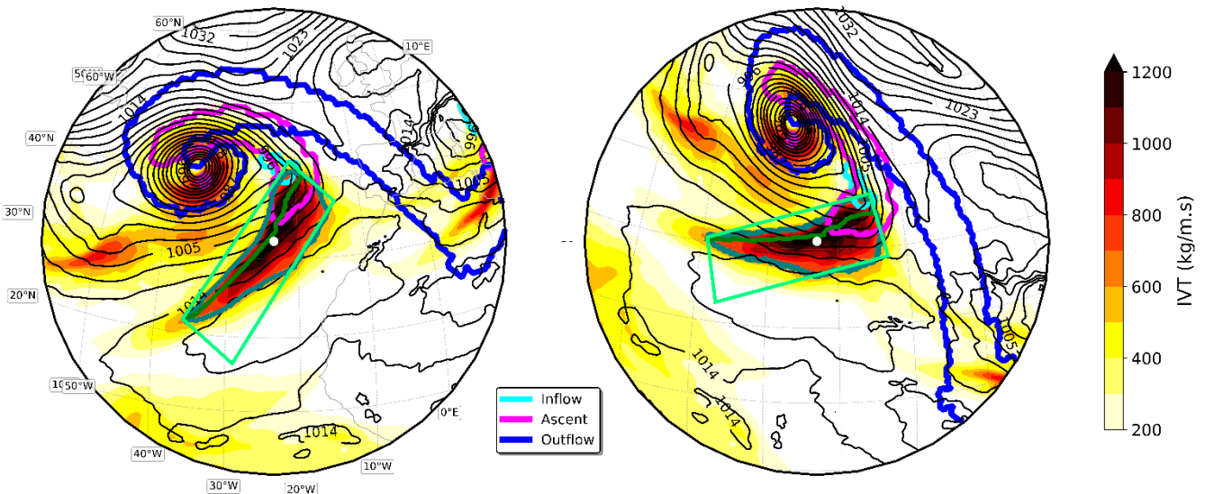
Figure 1: Schematic of the rotational composite methodology. (a) Original fields for a case study on 10 December 2022, 12 UTC, showing an atmospheric river AR (AR, dark-green contour), the warm conveyor belt WCB (WCB) inflow (light blue), ascent (pink), and outflow (blue) phases, sea-level pressure (SLP, black contours), and IVT (shaded in \text{kg m}^{-1} \text{s}^{-1} ). The ETC center is located northwest of the AR. The light-green box denotes the search region for WCB ascent influence. The white point marks the AR centroid and the green line inside the AR represents its axis. (b) The same fields after application of the rotational and latitude-correction algorithm, aligning the AR axis zonally (west-to-east, green line inside the AR) for compositing.
