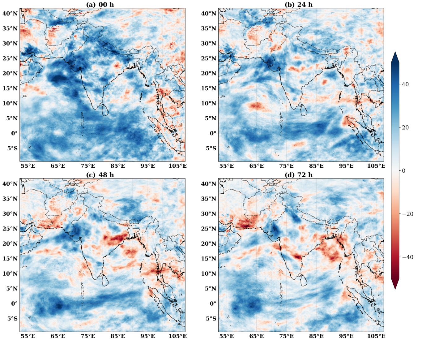
Figure 8. Spatial distribution of the total-energy-TE impact parameter-metric at forecast lead times of 00, 24, 48, and 72 h. Positive values indicate improvement due to RO assimilation.
