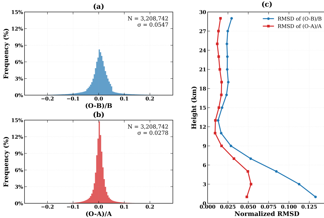
Figure 6. Histograms of the normalized (a) observation-minus-background (O-B) and (b) observation-minus-analysis (O-A) departures, and (c) vertical profiles of the corresponding normalized RMSD for assimilated bending-angle observations in the RMX-BA experiment.
