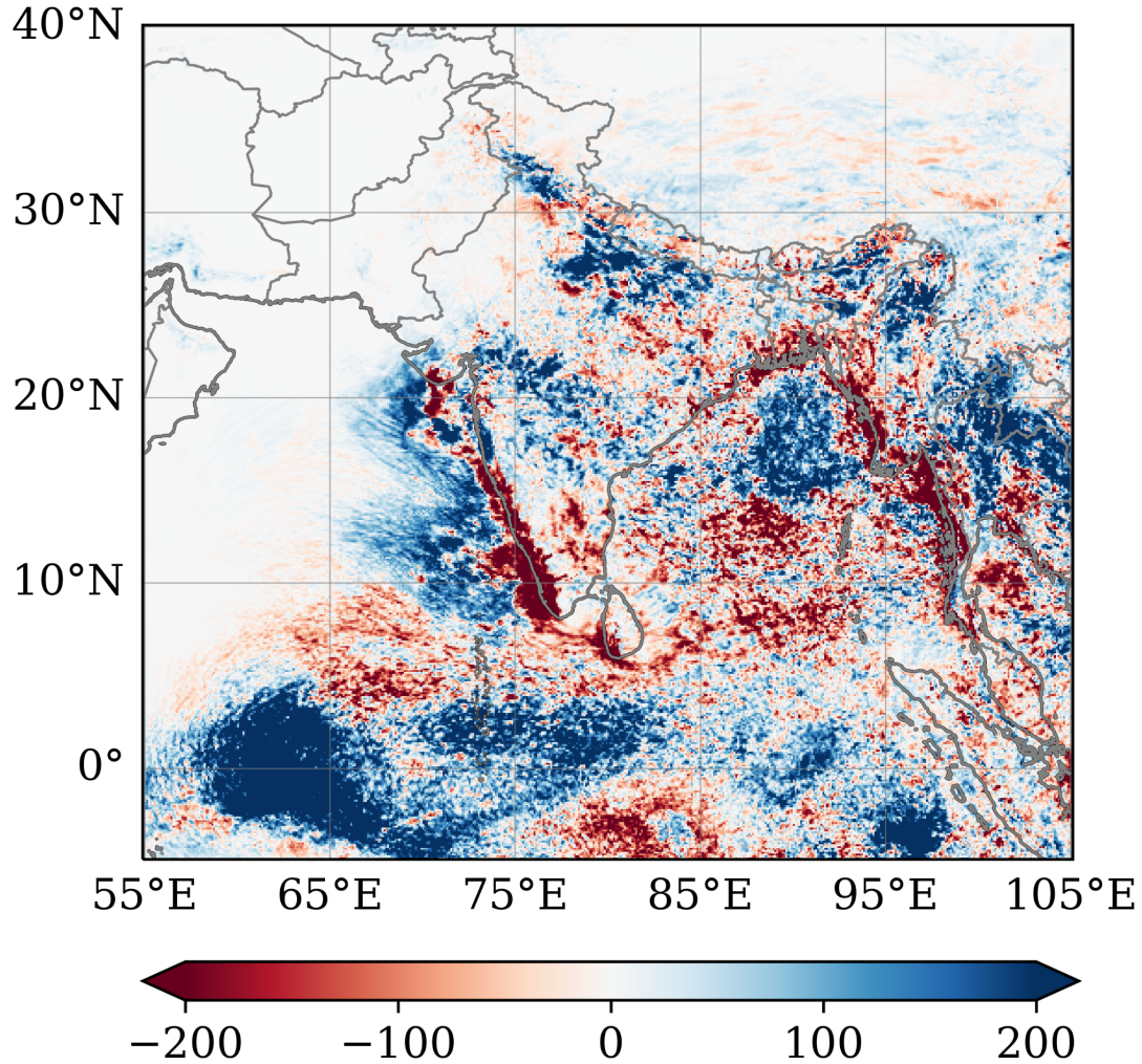
Figure 14. Spatial distribution of the rainfall impact parameter metric (mm) . Positive values denote reduced rainfall error due to RO assimilation.
