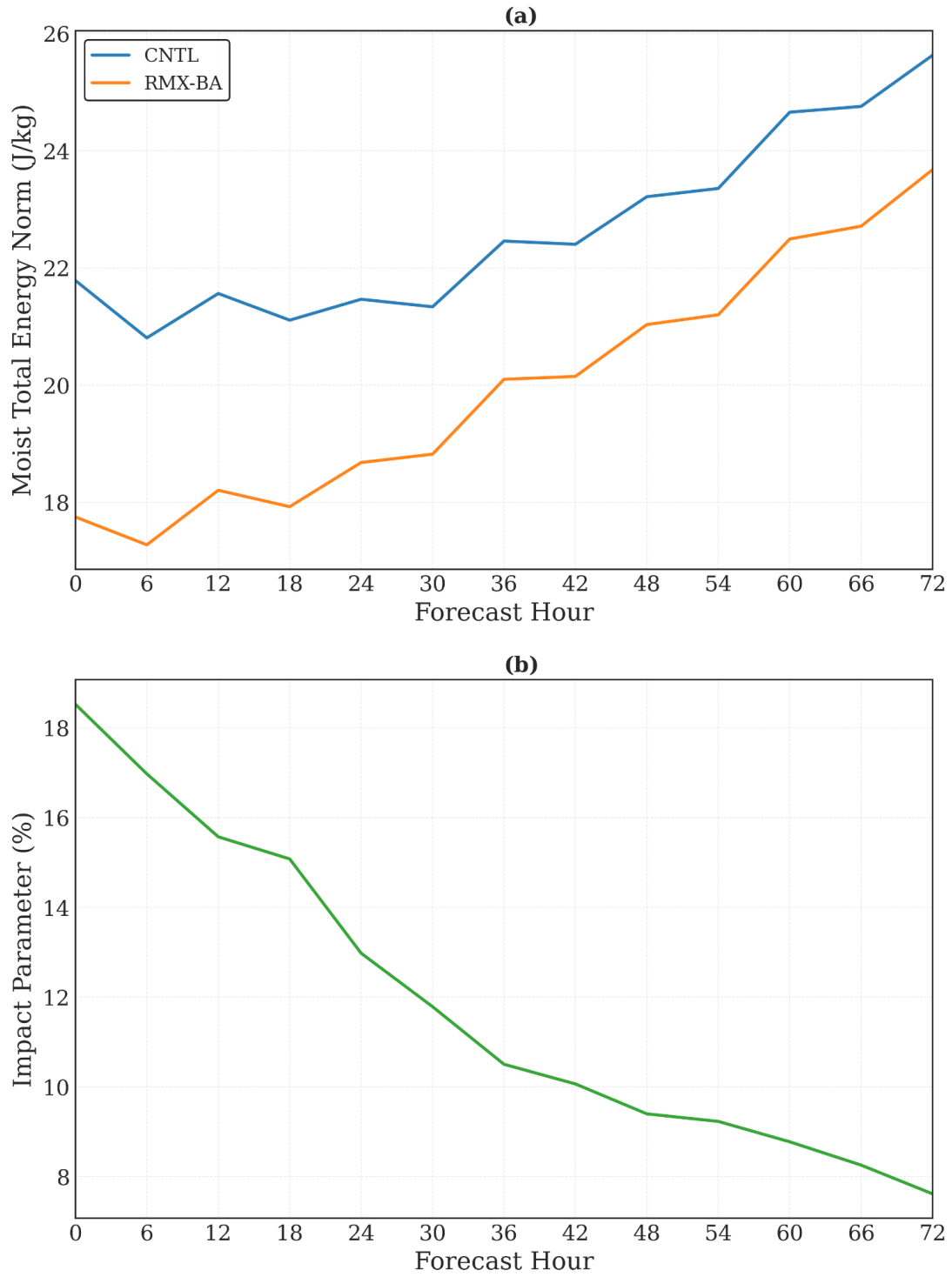
Figure 7. Domain-averaged moist total energy norm for CNTL and RMX-BA as a function of forecast lead time, together with the corresponding impact parameter metric derived from the total-energy norm.
