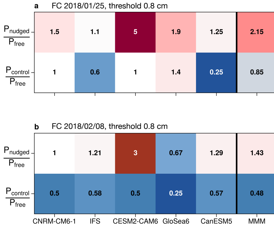
Figure 9. Non-parameteric Non-parametric RR calculated for 5 models (for which appropriate snow depth data was available) for southern UK and Ireland snow depth, with a threshold of 0.8 cm. Values are shown for early (a) and late (b) SSWFeb18 initialization dates, and a multi-model mean, calculated by averaging RR after calculating for individual models, is also shown. The version of GloSea6 shown is UKMO-GloSea6.
