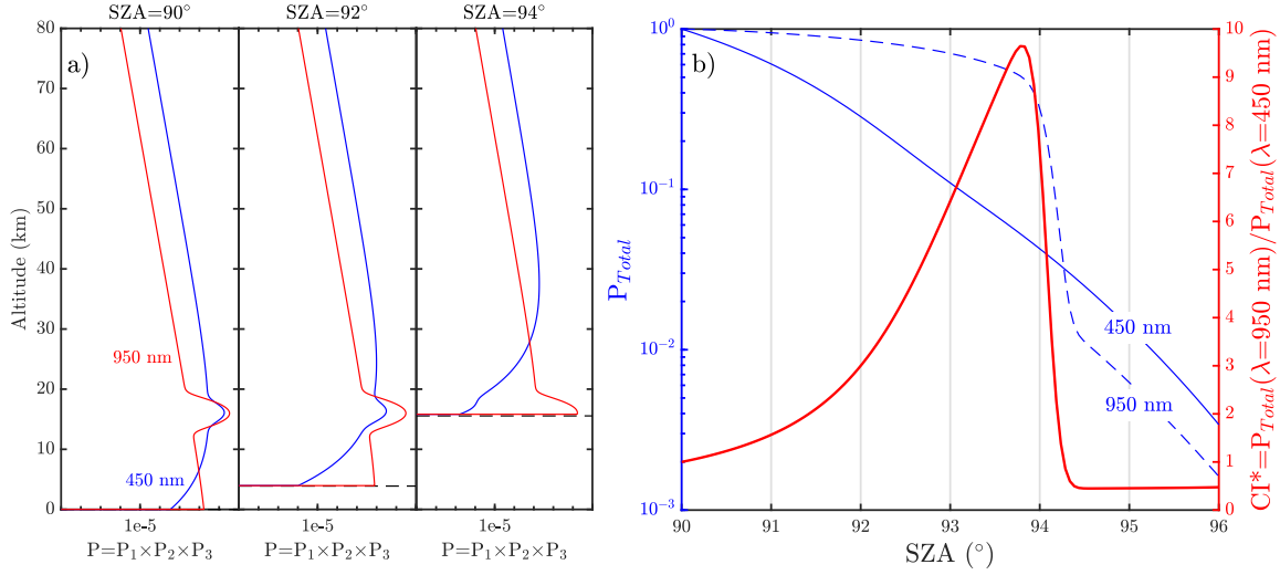
Figure 4. (a) Vertical profiles of P at 450 nm (blue lines) and 950 nm (red lines) for \text{SZA} = 90^\circ , 92^\circ , and 94^\circ . The atmospheric scenario is the same as in Figs. 2 and 3. (b) Variation of P_{\text{Total}} at 450 nm (blue solid line) and 950 nm (blue dashed line) with SZA for the atmospheric conditions of Figs. 2 and 3. The red solid line represents \text{CI}^* obtained from P_{\text{Total}} at 450 and 950 nm.
