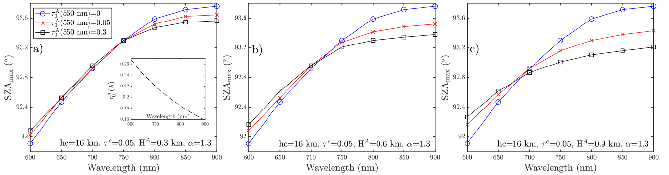
Figure 13. Variation of SZA_{max} with wavelength derived from CI^R for a cloud layer located at h_C = 16\text{ km} with optical depth \tau_C = 0.05 . Results are shown for different aerosol scenarios characterized by \tau_0^A(550\text{ nm}) = 0 (blue line), 0.05 (red line), and 0.3 (black line), and for three aerosol scale heights: H^A = 0.3\text{ km} (panel a), 0.6\text{ km} (panel b), and 0.9\text{ km} (panel c). The spectral dependence of \tau_0^A is parameterized using an Ångström exponent \alpha = 1.3 , whose corresponding curve is shown in the inset of panel (a).
