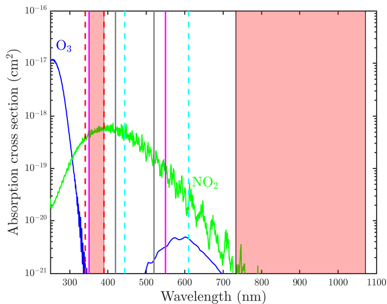
Figure 6. Absorption cross sections of NO 2 (green) and O 3 (blue) from Burrows et al. (1998) and Molina and Molina (1986), respectively. The gray and purple solid vertical lines indicate the wavelength pairs selected by Gomez-Martin et al. (2021) and Sarkissian et al. (1991), respectively, for the computation of the CI. The red and cyan dashed vertical lines indicate the wavelength pairs adopted by Lauster et al. (2022) for the UV and visible CI, respectively. The red shaded regions represent the wavelength ranges employed by Toledo et al. (2016).
