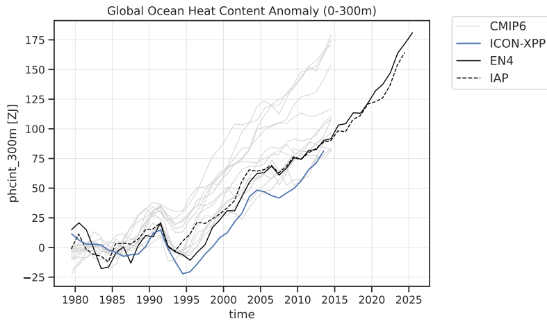
Figure 15. Time series of ocean heat content anomaly for the upper 300 m relative to the 1995-2014 average in zettajoules (ZJ). The black lines show the reference datasets, the blue line the ICON-XPP results and the thin gray lines results from the CMIP6 model ensemble.
