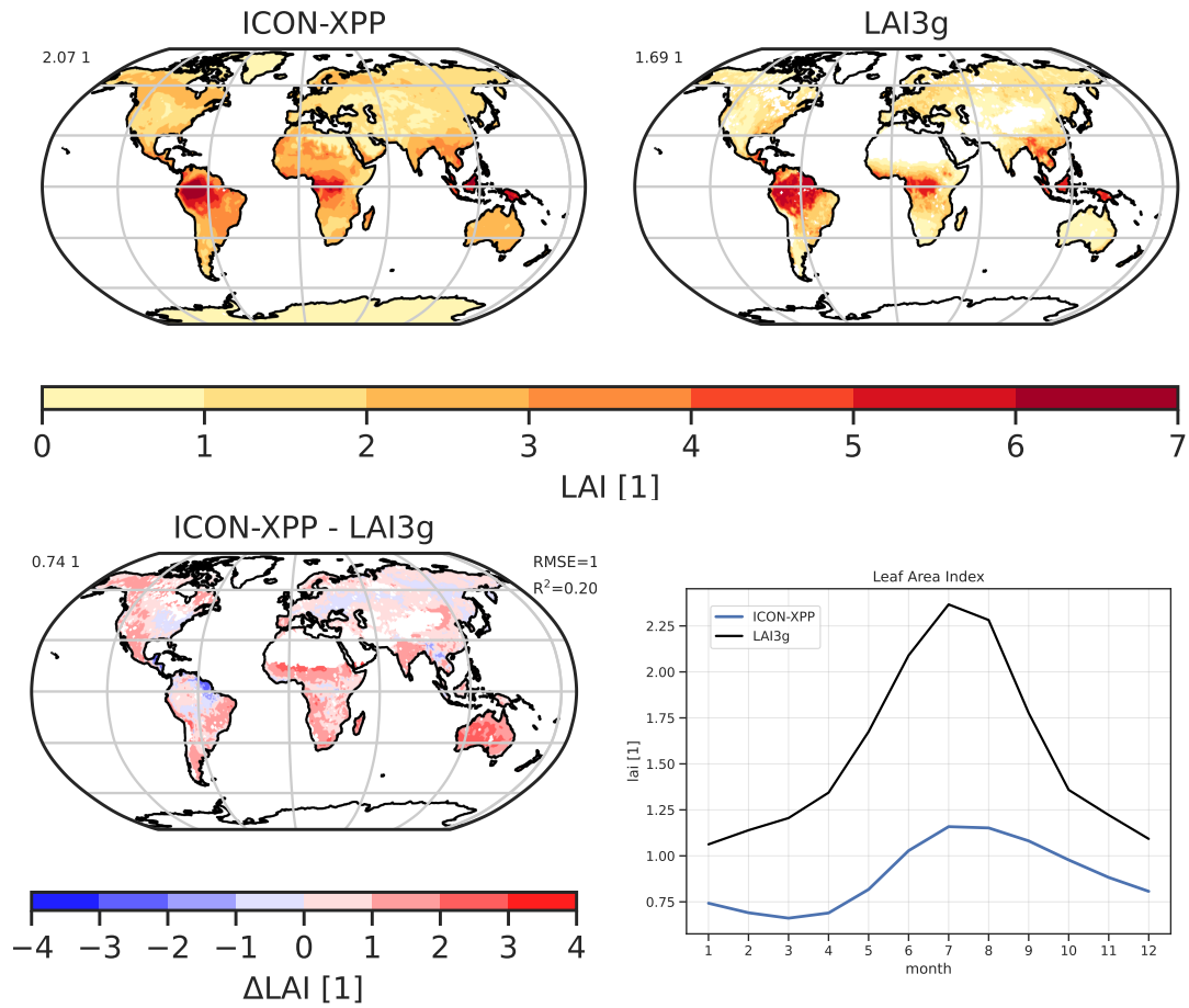
Figure 16. Average Leaf Area Index (LAI) from ICON-XPP averaged over the period 1995-2004 (top left), from the LAI3g observational dataset over the same period (top right) and their difference (bottom left). The average seasonal cycles averaged over the Northern Hemisphere are shown in the bottom right.
