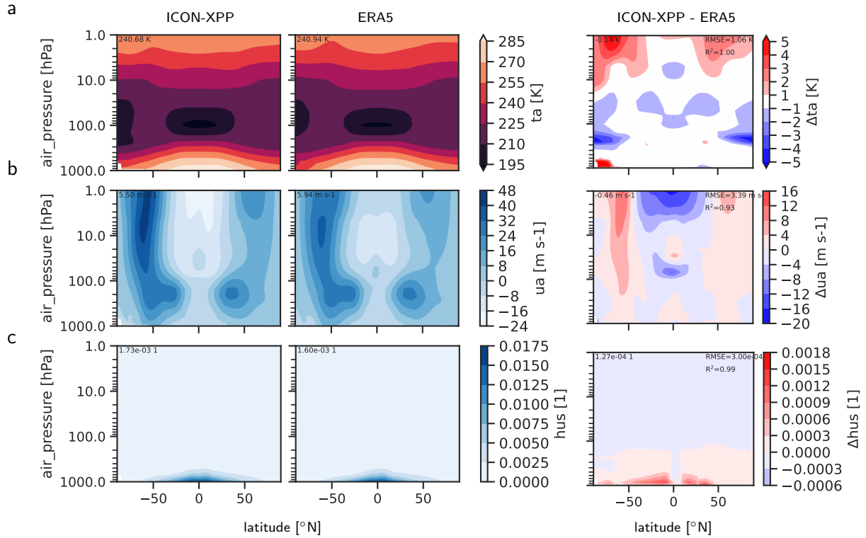
Figure 9. Zonal multi-year annual mean bias in (a) temperature, (b) zonal wind speed, and (c) specific humidity from ICON-XPP compared with ERA5.
