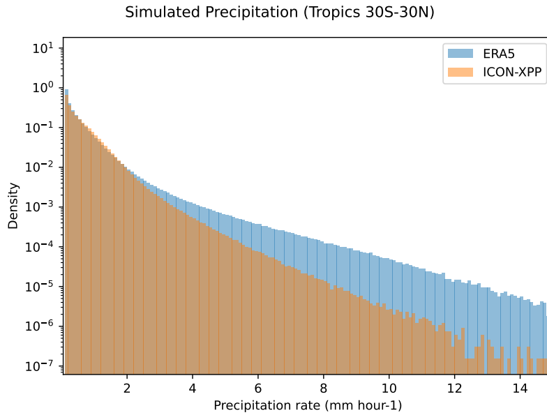
Figure 7. Probability density of the precipitation rates in the Tropics ( 30^{\circ}\text{S} - 30^{\circ}\text{N} ) calculated over the time period 2010-2014 from ICON-XPP (orange) compared with ERA5 (blue). All data have been regridded to the same regular 1^{\circ}\times 1^{\circ} lat-lon grid and averaged to 6-hourly intervals.
