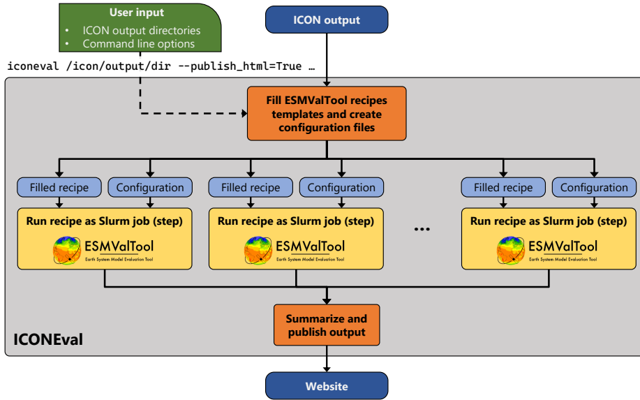
Figure 1. Schematic overview of ICONEval. Based on ICON output (from one or multiple simulations), ICONEval fills ESMValTool recipes and creates corresponding configuration files. These recipes are run in parallel by ESMValTool using Slurm job (steps). Finally, results are summarized and (if desired) published to a website for easy access.
