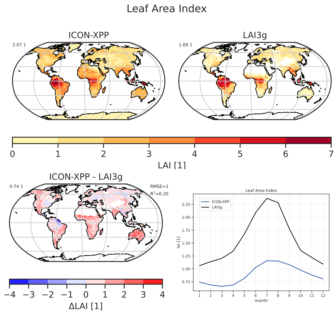
Figure 16. Average Leaf Area Index ( LAI ) from ICON-XPP averaged over the period 1995-2004 (top left), from the LAI3g observational dataset over the same period (top right) and their difference (bottom left). The average seasonal cycles averaged over the Northern Hemisphere are shown in the bottom right.
