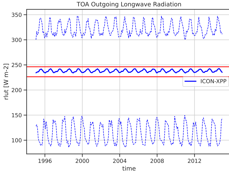
Figure 2. Time series of global monthly mean (solid line) and minimum/maximum (across all grid cells, dashed lines) TOA outgoing longwave radiation. Red horizontal lines show "reasonable" upper and lower limits for the global mean calculated from minimum and maximum global monthly mean values found in reference datasets (i.e. observations, reanalyses) across all months and all reference datasets.
