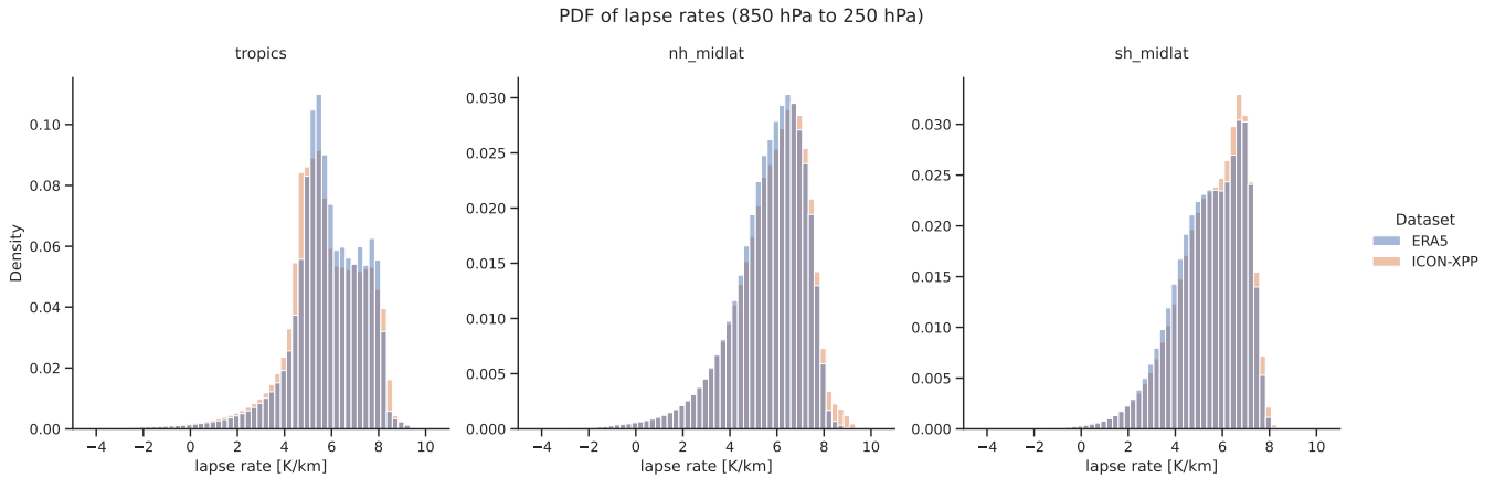
Figure 5. Probability density functions of the 3-dim lapse rates from ERA5 (blue) and ICON-XPP (orange) in the altitude range 850 hPa to 250 hPa calculated from monthly mean temperatures over the time period 1995-2014. From left to right: Tropics (30°S-30°N), Northern Hemisphere mid-latitudes (40°N-60°N) and Southern Hemisphere mid-latitudes (60°S-40°S).
