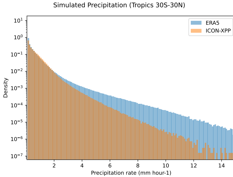
Figure 7. Probability density of the precipitation rates in the Tropics (30°S-30°N) calculated over the time period 2010-2014 from ICON-XPP (orange) compared with ERA5 (blue). All data have been regridded to the same regular 1°x1° lat-lon grid and averaged to 6-hourly intervals.
