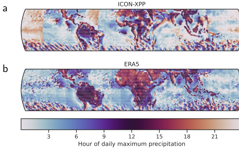
Figure 8. Hour of daily maximum precipitation (local time) in the Tropics ( 30^{\circ}\text{S} - 30^{\circ}\text{N} ) for June-July-August calculated over the time period 2010-2014 from (a) ICON-XPP compared with (b) ERA5. The ERA5 data have a time resolution of 1 hour, the ICON-XPP of 6 hours. A time resolution of less than hourly is not optimal and might introduce some artifacts as can be seen by the striped appearance of the ICON-XPP panel.
