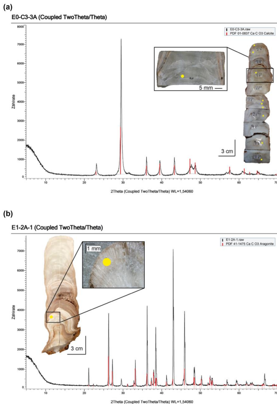
Figure S 2 (a) X-ray diffraction (XRD) pattern showing the characteristic diffraction peaks (2 \theta ) of calcite for a sample from stalagmite E0-C. The image on the right displays the remaining stalagmite cubes from the thin section preparation, from which sample powder was drilled for XRD analysis (yellow dots). The inset indicates the location of the sample corresponding to the presented diffraction pattern. All eight additional samples analyzed from stalagmite E0-C exhibited the same calcite pattern and are therefore not shown. (b) XRD pattern showing the characteristic diffraction peaks (2 \theta ) of aragonite for a sample from the bottom part of stalagmite E1 (yellow dot on the scan). The presence of millimeter-sized needle-like crystals with a silky luster suggested an aragonitic phase, which was confirmed by XRD analysis. Peak positions and intensity data were analyzed using Diffrac.Suite EVA software (Bruker).
