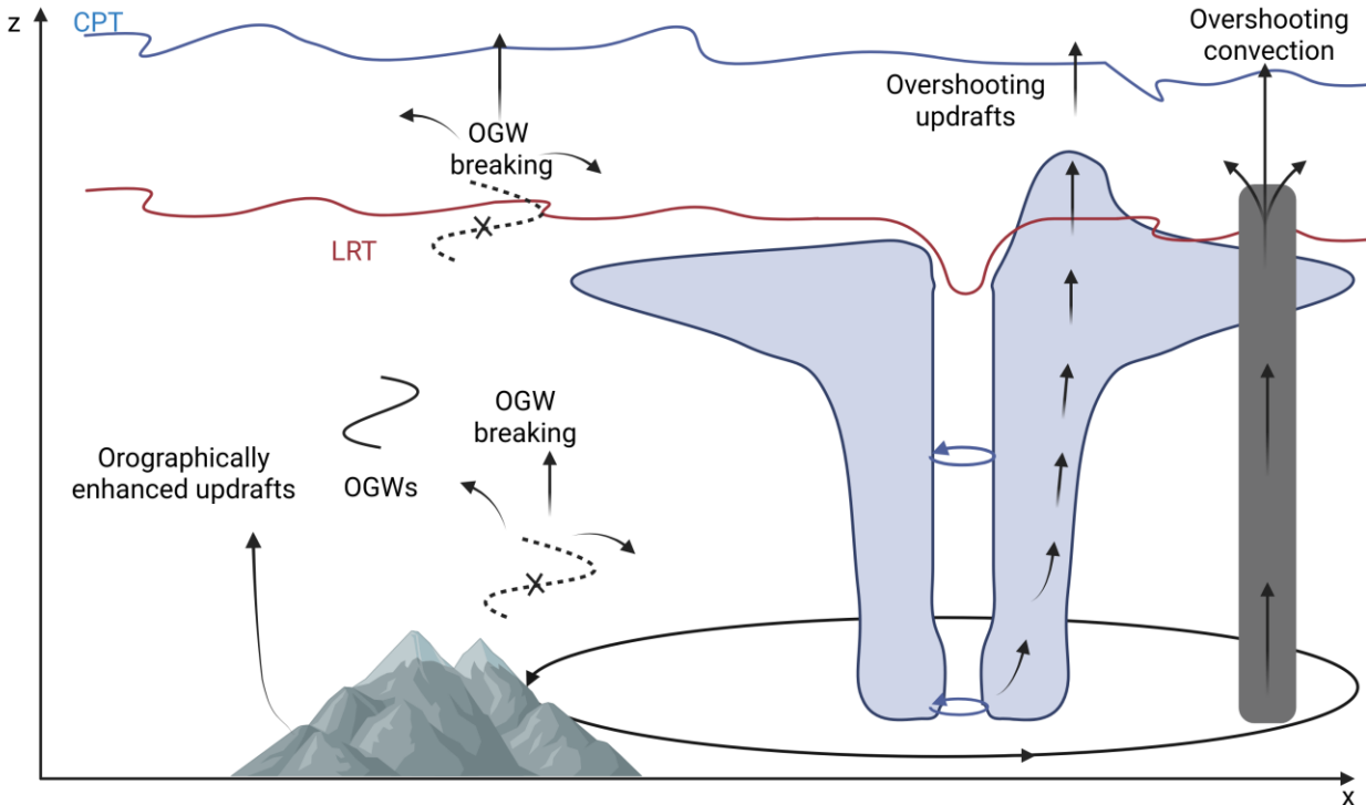
Figure 9 (previously Figure 7). Sketch of the troposphere-to-stratosphere transport arising from the interaction of a typhoon with orography based on the illustration by Gordon and Homeyer (2025) of a tropical cyclone cross section. It points out the significant contributions of orographic updraft enhancement and orographic gravity wave (OGW) breaking close to the tropopause and near the surface. The blue line represents the Cold Point Tropopause (CPT) and the red one the Lapse Rate Tropopause (LRT).
