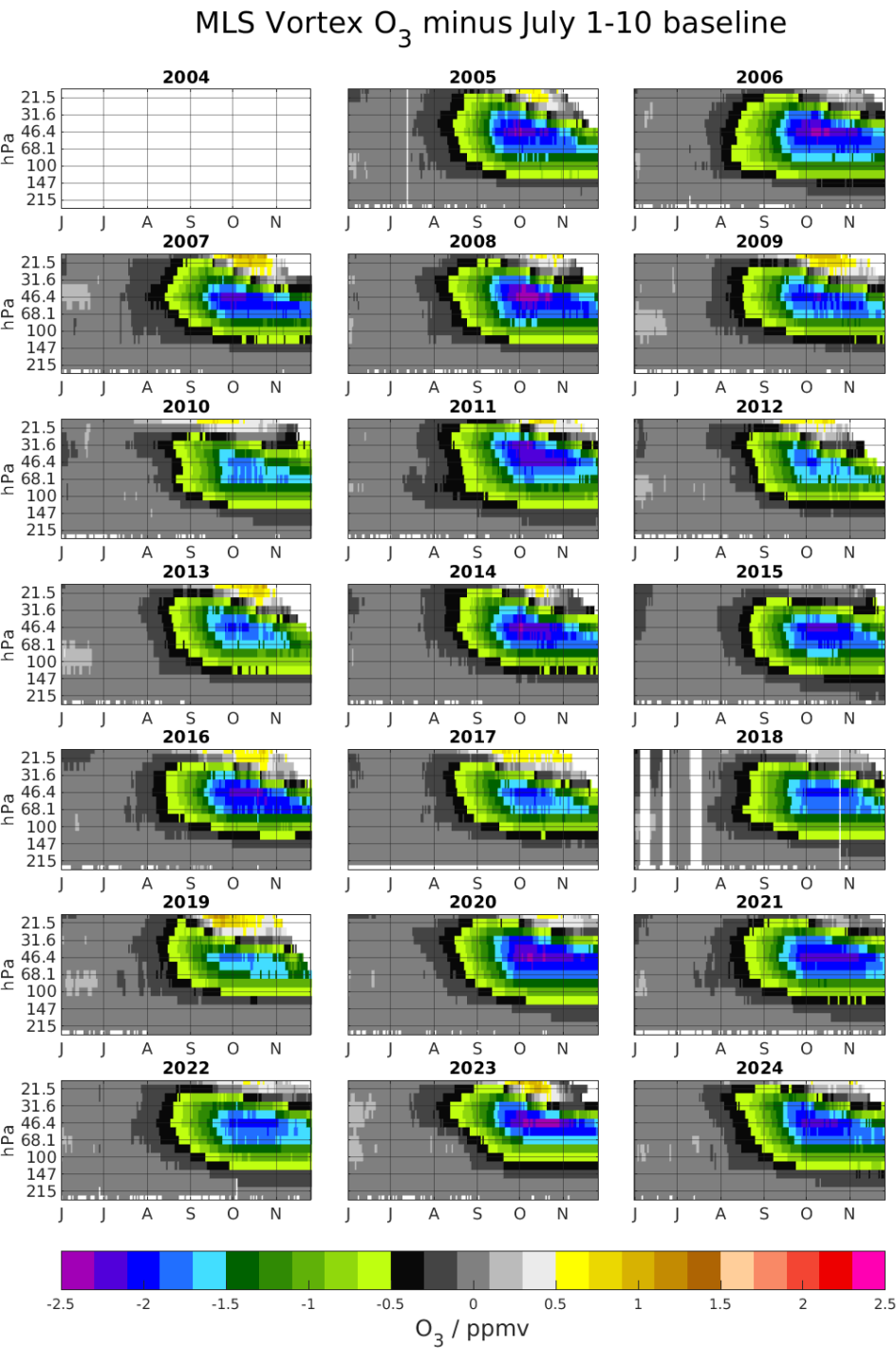
1011 1012 Figure 1. June to November vortex-average lower stratospheric ozone profiles over the range 215– 1013 21 hPa for 2005-2024. The respective July 1-10 average is subtracted for each year to remove 1014 interannual variability of early-winter (baseline) conditions. Partial 2004 is not included because 1015 MLS operations had not begun in July, so this baseline could not be calculated
