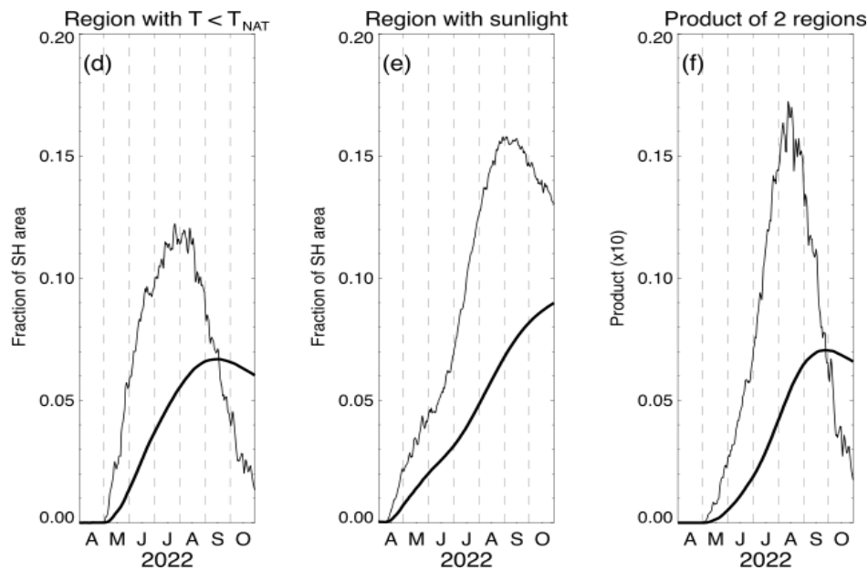
Figure 8. The lower stratospheric layer-average Antarctic vortex area with T < T_{\text{NAT}} for (a) 2019 and (d) 2022; the lower stratospheric layer-average Antarctic vortex area exposed to sunlight for (b) 2019 and (e) 2022; and the product (multiplied by 10) of these two layer-average areas for (c) 2019 and (f) 2022. Layer averages are calculated over potential temperature levels from 330 K to 620 K. The thin lines depict daily quantities, whereas the thick lines are time-averaged values of these quantities through each day of the year, from April 1. The layer-average area diagnostics are expressed as a fraction of the total Southern Hemisphere (SH) area.
