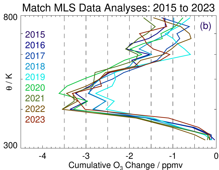
Figure 18. Profiles of maximum cumulative ozone change (with a negative value representing a loss) from the Match technique inside the Antarctic vortex, based on weekly averages in the winter/spring for (a) 2005–2014 and (b) 2015–2023.
