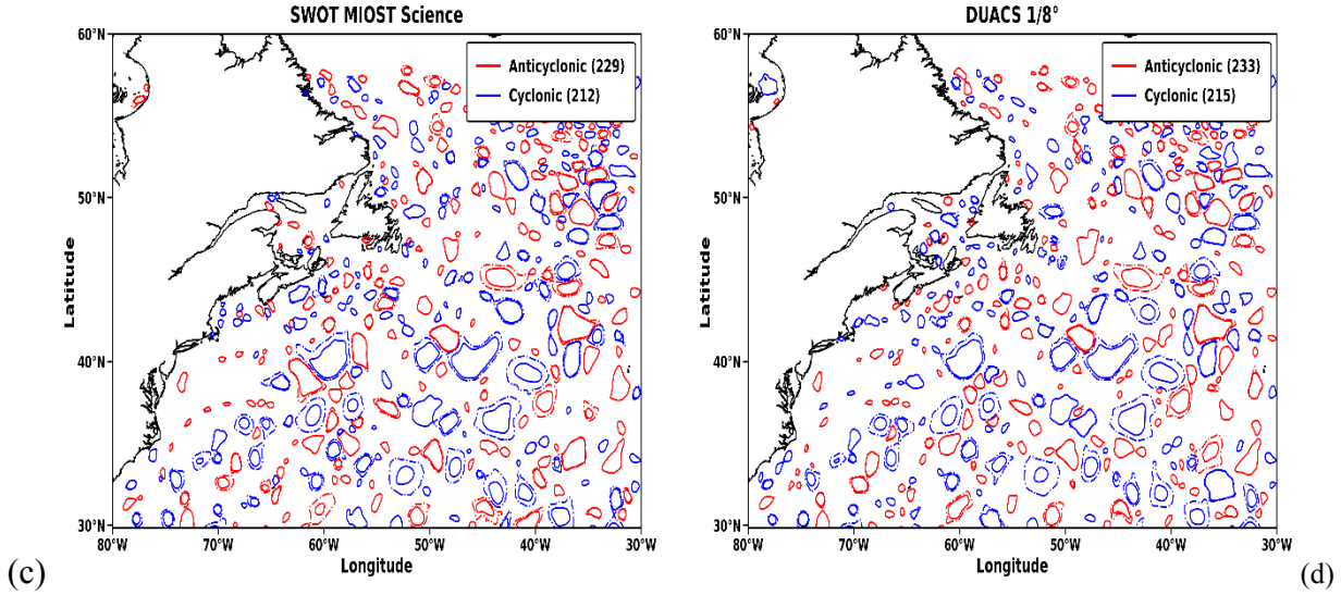
Fig.3. Eddy identification in North-Atlantic area, after a Bessel filtering of SSH field (cm) with a cutoff of 500 km, valid for 1 st January 2025, for: (a) GLORYS12V1 (re-gridded onto 1/8° regular grid), (b) GLORYS2V4 (re-gridded onto 1/8° regular grid), (c) SWOT MIOST Science, (d) AVISO DUACS 1/8°.
