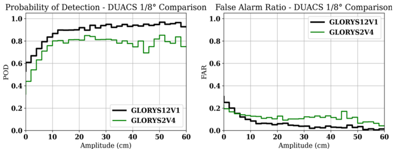
Fig. 11. On the top: histograms of the probability of detection (POD; left) and the false alarm ratio (FAR; right), over the evaluation period, evaluated as a function of amplitude (cm) for comparison with DUACS 1/8°. In the bottom: histograms of the POD and FAR as a function of amplitude (cm), over the evaluation period, for the comparison with SWOT MIOST Science.
