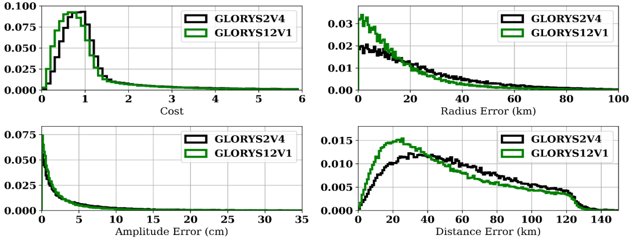
Fig. 14. Normalized histograms of values for matched eddies between SWOT MIOST Science and GLORYS2V4 (black line) or GLORYS12V1 (green line), in (a). While in (b), the comparison between DUACS 1/8° and GLORYS2V4 (black line) or GLORYS12V1 (green line). The distribution of values for the total cost is shown in the top panel on the left. Also shown are the normalized distributions of differences in terms of radius in the top on the right, amplitude in the bottom on the right, and distance between eddy positions, in the bottom on the right.
