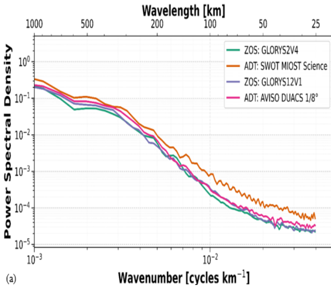
Fig.2. Power spectral density (PSD) of ADT (ZOS) for the four datasets on 1 January 2025, computed over the selected North Atlantic region. All products were re-mapped onto the same 1/8^\circ regular grid. Panel (a) shows the PSD along the zonal (ky)
