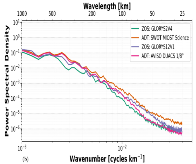
Fig.2. Power spectral density (PSD) of ADT (ZOS) for the four datasets on 1 January 2025, computed over the selected North Atlantic region. All products were re-mapped onto the same 1/8^\circ regular grid. Panel (a) shows the PSD along the zonal (ky)
