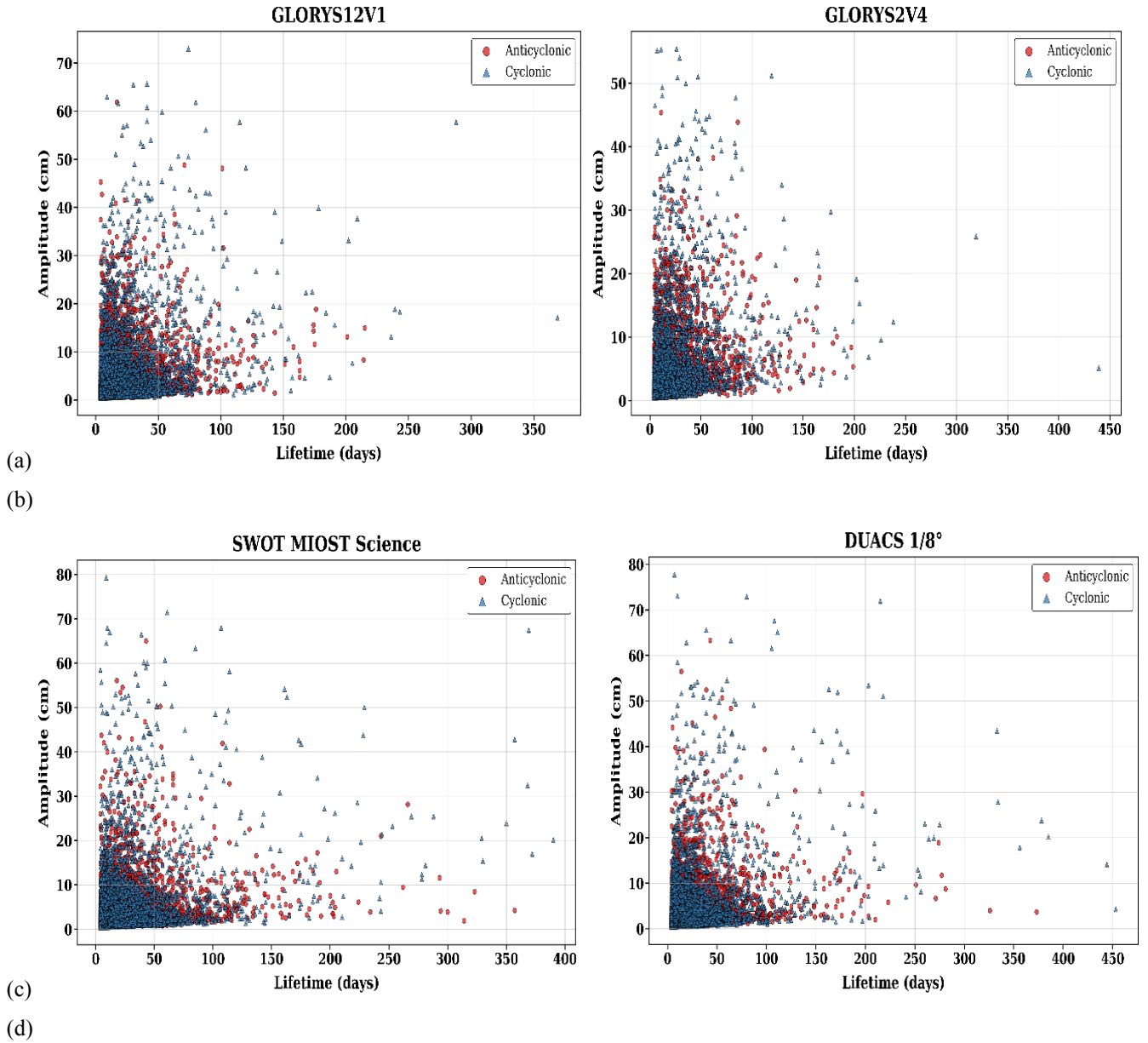
Fig.5. Scatter plots of identified eddies, with a lifetime threshold of 4 days, between Amplitude vs Lifetime of eddies for (a) GLORYS12V1, (b) GLORYS2V4, (c) SWOT MIOST Science, (d) AVISO DUACS 1/8°. Each eddy is counted only once. Most eddies have an amplitude of less than 10 cm. However, their mean lifetime is lower than 50 days. The amplitude is calculated at the trace level, by averaging the amplitude over the entire lifetime of the eddy.
