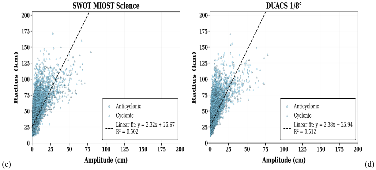
Fig. 4. Scatter plots of detected eddies, with a minimum lifetime threshold of 4 days, between Radius and Amplitude, from 2023-08-01 to 2025-05-01, for (a) GLORYS12V1 (remapped onto AVISO grid), (b) GLORYS2V4 (remapped onto AVISO grid), (c) SWOT MIOST Science, and (d) AVISO DUACS 1/8°. The eddy amplitude and the eddy radius are calculated at the trace level, by averaging the amplitude and radius over the entire lifetime of the eddy.
