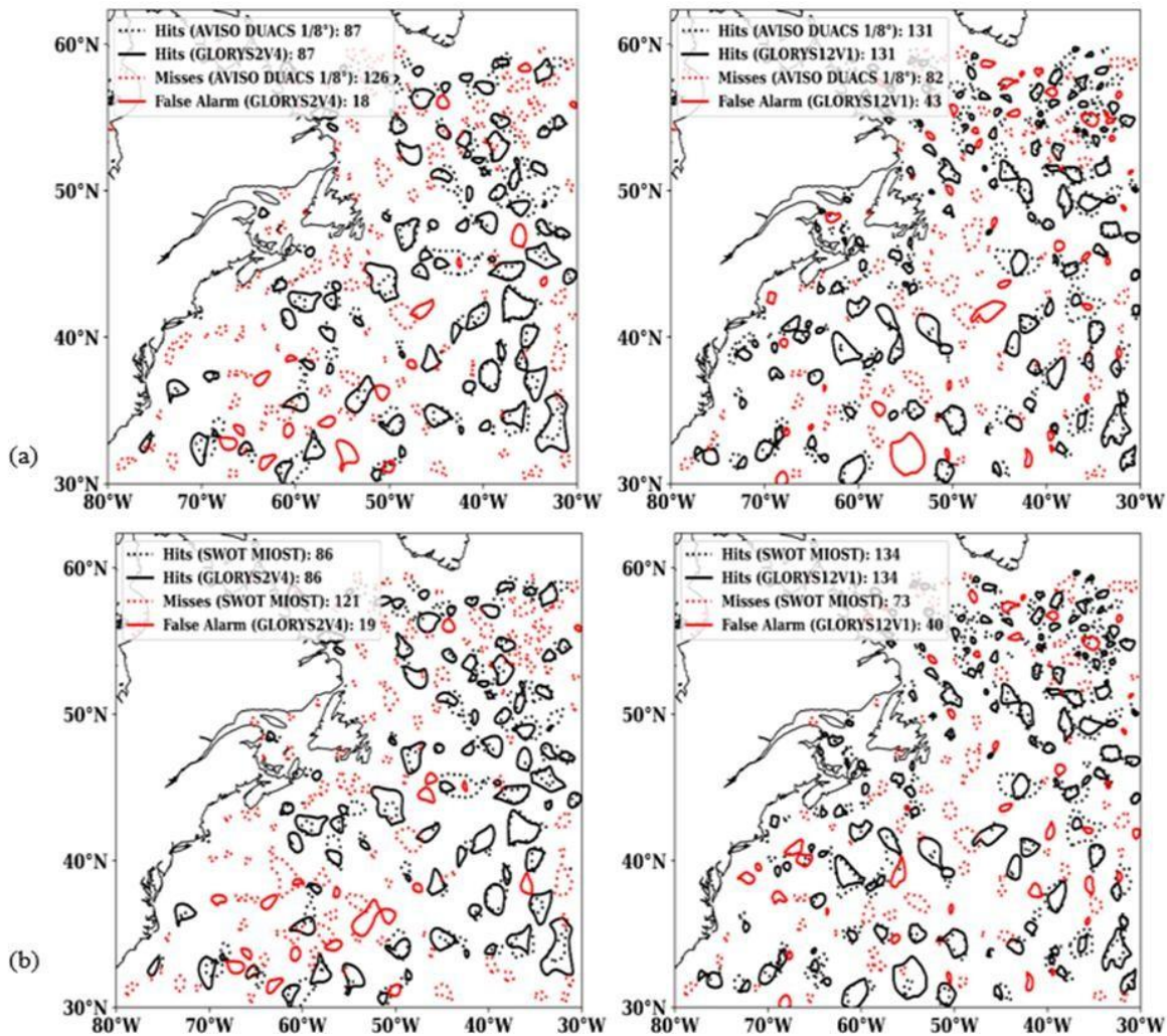
Fig. 5. The first one (a) is an example showing Anticyclonic eddy matching statistics for 1st January 2025 for GLORYS2V4 (left), and GLORYS12V1 (right), compared with DUACS. Eddies for which a corresponding match is found (hits) between DUACS and GLORYS2V4/GLORYS12V1 are shown as dotted and solid black contours. Eddies identified in DUACS (satellite data) with no corresponding eddy in GLORYS2V4/GLORYS12V1 are deemed misses (red dotted contours). Eddies identified in GLORYS2V4/GLORYS12V1 but without a corresponding eddy to DUACS are deemed false alarms. The second one (b) is an example showing Anticyclonic eddy matching statistics for 1st January 2025 for GLORYS2V4 (left), and GLORYS12V1 (right), compared with SWOT (satellite data)..
