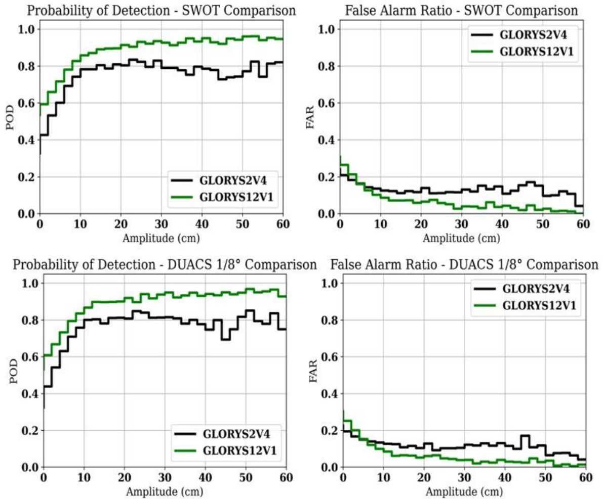
Fig. 10. On the top: histograms of the probability of detection (POD; left) and the false alarm ratio (FAR; right), over the evaluation period, evaluated as a function of amplitude (cm) for comparison with SWOT. In the bottom: histograms of the POD and FAR as a function of amplitude (cm), over the evaluation period, for the comparison with DUACS. The amplitude of hits and misses refers to the satellite (reference) eddies, while the amplitude of false alarms refers to those of unmatched eddies detected in the reanalysis."
