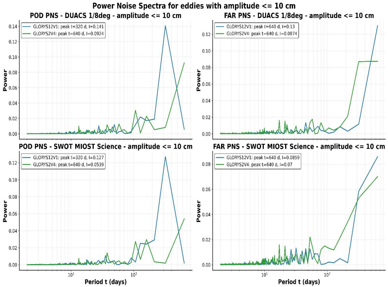
Fig. C4. (a) POD and FAR time series for eddies with amplitudes \leq 10 cm for the comparisons with DUACS 1/8^\circ and SWOT MIOST Science. (b) Corresponding power spectra. A 4-day minimum-lifetime threshold is used.
