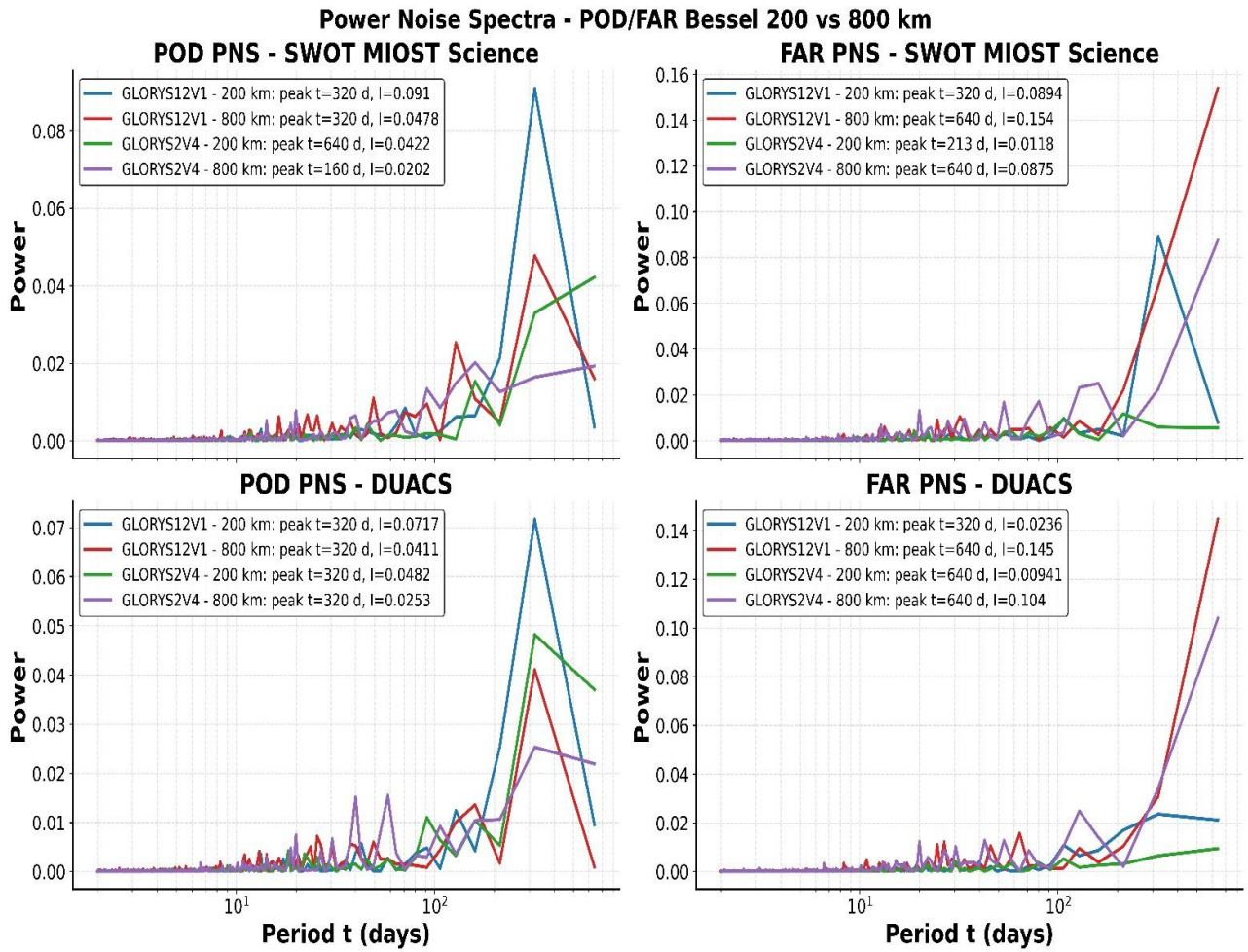
Fig. D3. POD and FAR time series obtained using Bessel-filter cutoff wavelengths of 200 and 800 km for the comparisons with (a) SWOT MIOST Science and (b) DUACS 1/8^\circ . Panel (c) shows the corresponding power spectra. A 4-day minimum-lifetime threshold is used.
