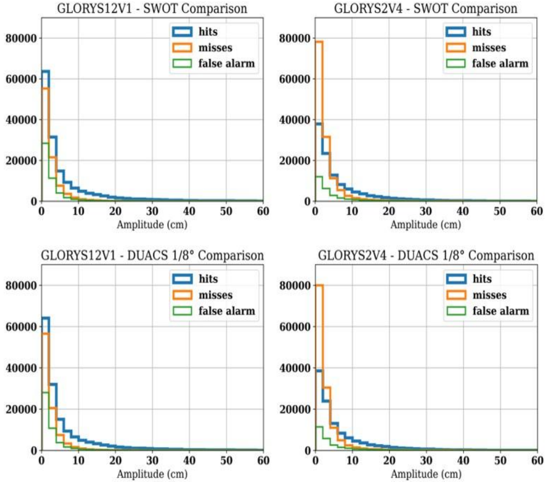
Fig.9. On the top: eddy matching histograms for the total number of hits (blue), misses (orange), false alarms (green) for GLORYS12V1 (left) and GLORYS2V4 (right), compiled as a function of amplitude (cm) over the evaluation period, for SWOT comparison. In the bottom: eddy matching histograms compiled as a function of amplitude (cm) over the evaluation period, for comparison with DUACS 1/8°. The amplitude of hits and misses refers to the satellite (reference) eddies, while the amplitude of false alarms refers to those of unmatched eddies, detected in the reanalysis.
