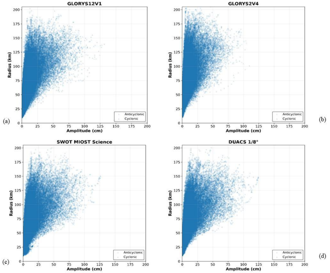
Fig. 3. Scatter plots of detected eddies, with a minimum lifetime threshold of 4 days, between Radius and Amplitude, from 2023-08-01 to 2025-05-01, for (a) GLORYS12V1 (bilinear remapped onto DUACS and SWOT grid), (b) GLORYS2V4 (bilinear remapped onto DUACS and SWOT grid), (c) SWOT MIOST Science, and (d) AVISO DUACS 1/8°. The eddy amplitude and the eddy radius are calculated at the track level, by averaging the amplitude and radius over the entire lifetime of the eddy.
