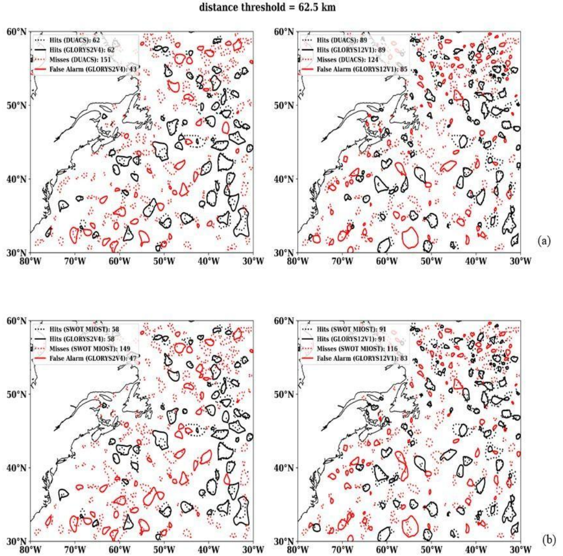
Fig. D1. Anticyclonic-eddy matching on 1 January 2025 using a maximum centroid distance of 62.5 km. GLORYS2V4 is shown on the left and GLORYS12V1 on the right, for the comparisons with (a) DUACS 1/8° and (b) SWOT MIOST Science.
