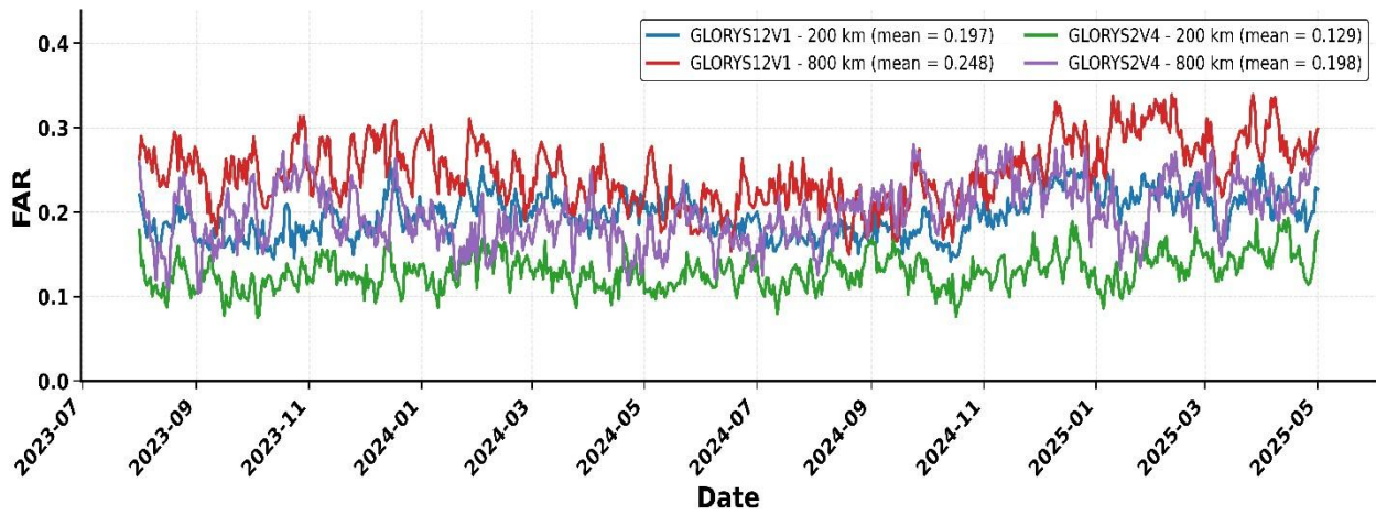
False Alarm Ratio - SWOT MIOST Science: 200 vs 800 km Bessel filter
