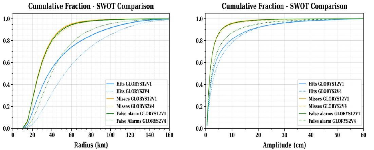
Fig.12. Cumulative distribution of hits (blue), misses (orange) and false alarms (green) for GLORYS12V1 (solid) and for GLORYS2V4 (dotted) as a function of radius (left) and amplitude (right), for the comparison with SWOT, with a lifetime threshold of 4 days. The radius and the amplitude of hits and misses refers to the satellite (reference) eddies, while the radius and the amplitude of false alarms refers to the unmatched eddies detected in the reanalysis.”
