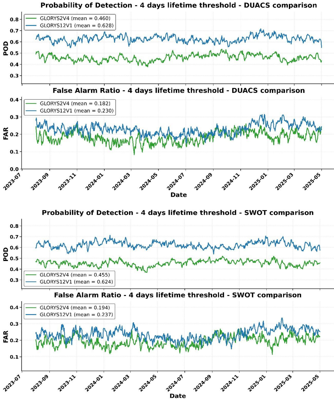
Fig.6. Timeseries of matching statistics for GLORYS2V4 and GLORYS12V1, compared with DUACS 1/8°, over the period from 1st August 2023 to 1st May 2025, for a 4-day minimum lifetime threshold (a). and in the bottom, the timeseries with SWOT MIOST Science, over the period from 1st August 2023 to 1 May 2025, for a 4-day minimum lifetime threshold (b).
