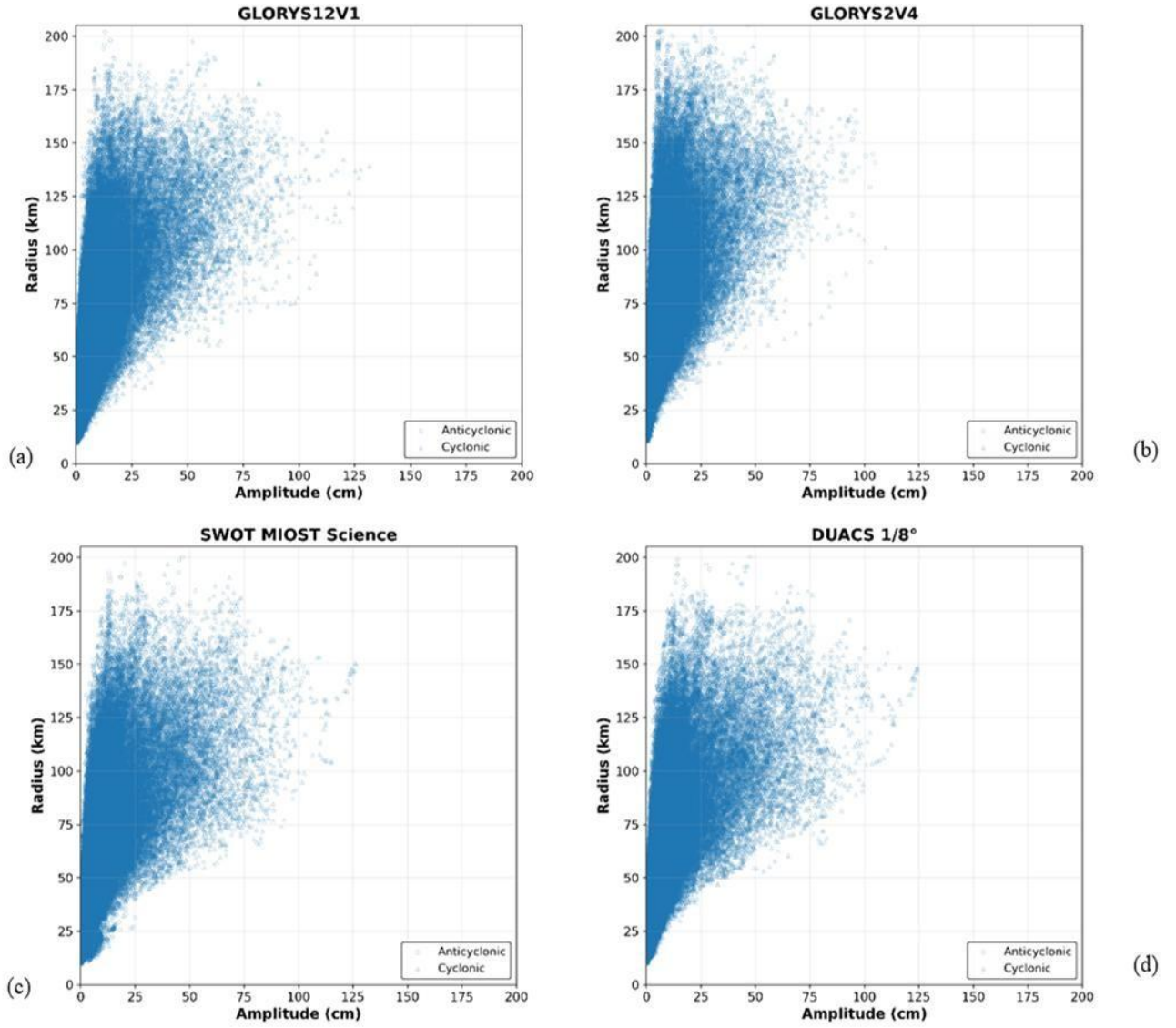
Fig. 3. Scatter plots of detected eddies, with a minimum lifetime threshold of 4 days, between Radius and Amplitude, from 2023-0801 to 2025-05-01, for (a) GLORYS12V1 (bilinear remapped onto DUACS and SWOT grid), (b) GLORYS2V4 (bilinear remapped onto DUACS and SWOT grid), (c) SWOT MIOST Science, and (d) AVISO DUACS 1/8°. The eddy amplitude and the eddy radius are calculated at the track level, by averaging the amplitude and radius over the entire lifetime of the eddy.
