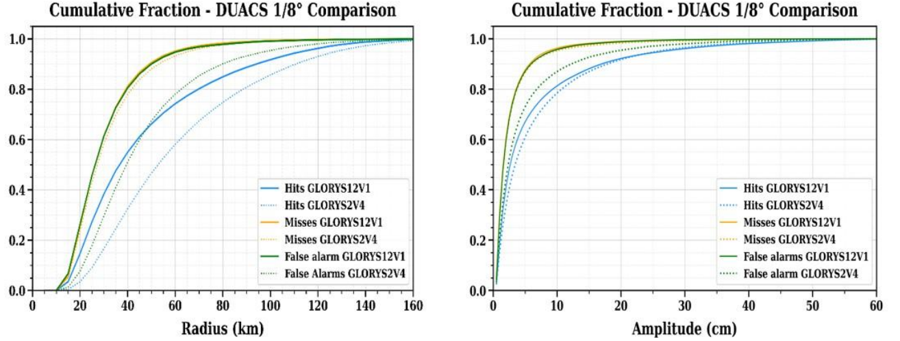
Fig. 11. Cumulative distribution of hits (blue), misses (orange) and false alarms (green) for GLORYS12V1 (solid) and for GLORYS2V4 (dotted) as a function of radius (left) and amplitude (right), for the comparison with DUACS, with a lifetime threshold of 4 days. The radius and the amplitude of hits and misses refers to the satellite (reference) eddies, while the radius and the amplitude of false alarms refers to the unmatched eddies detected in the reanalysis.
