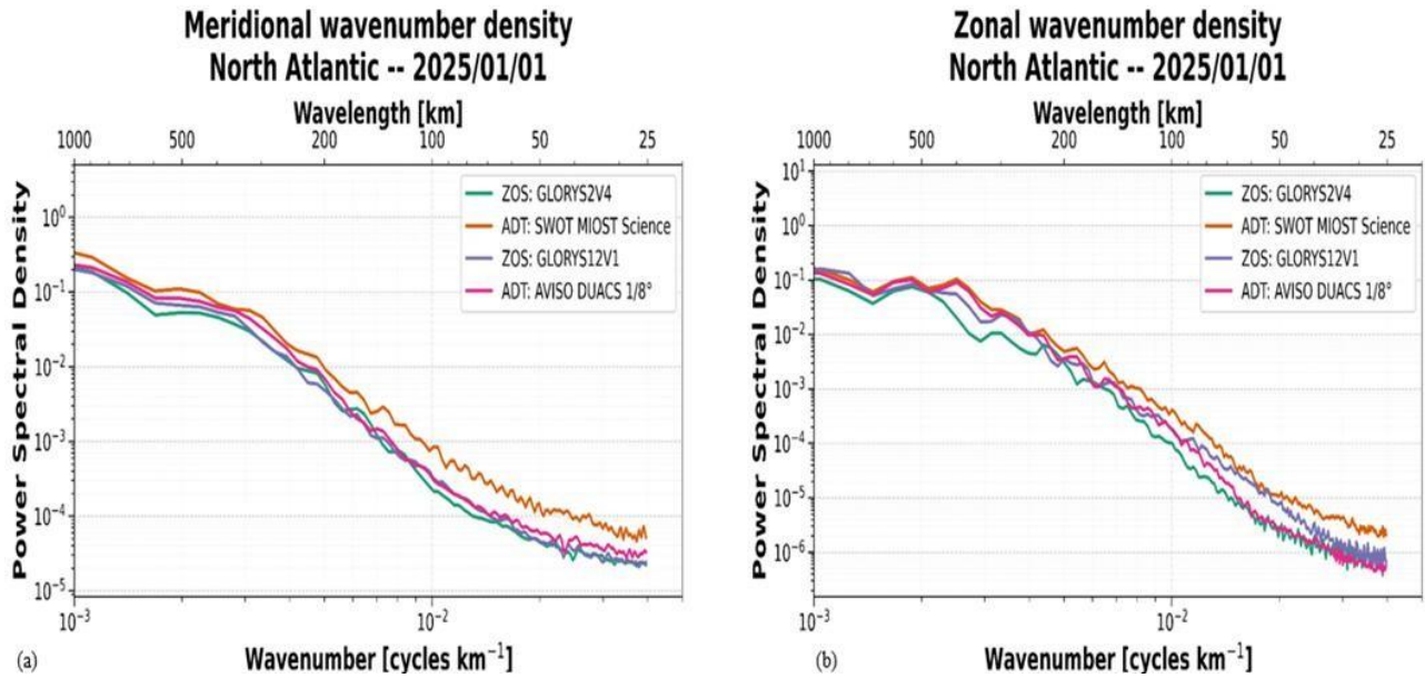
Fig.2. Power spectral density of SSH, corresponding to ADT for the satellite altimetry products, for the four datasets on 1 January 2025 over the selected North Atlantic region. All fields were projected onto a Lambert Azimuthal Equal-Area coordinate system and interpolated onto a regular kilometre-scale grid with dx = dy = 12.5 km, before computing the spectra. Panel (a) shows the meridional spectrum and panel (b) the zonal spectrum. Wavenumbers are expressed in cycles / km, with the corresponding wavelengths shown in kilometres on the upper x-axis.
