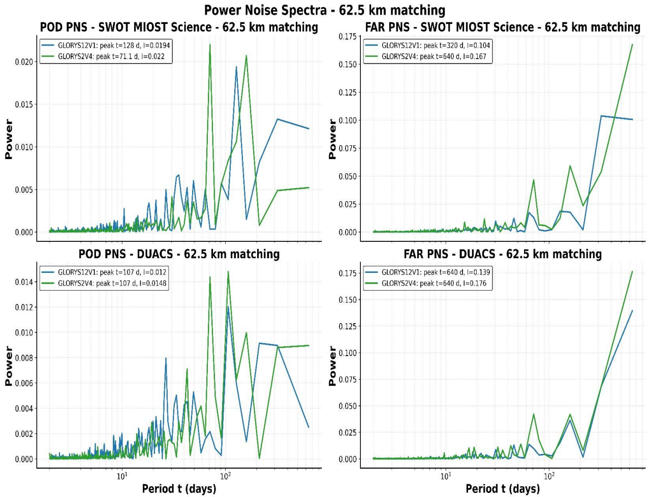
Fig. D2. (a) Time series for the verification metrics, for the comparison with SWOT MIOST Science and DUACS 1/8^\circ comparison, with a minimum lifetime threshold of 4 days. In (b) power spectra for all the time series presented in (a).
