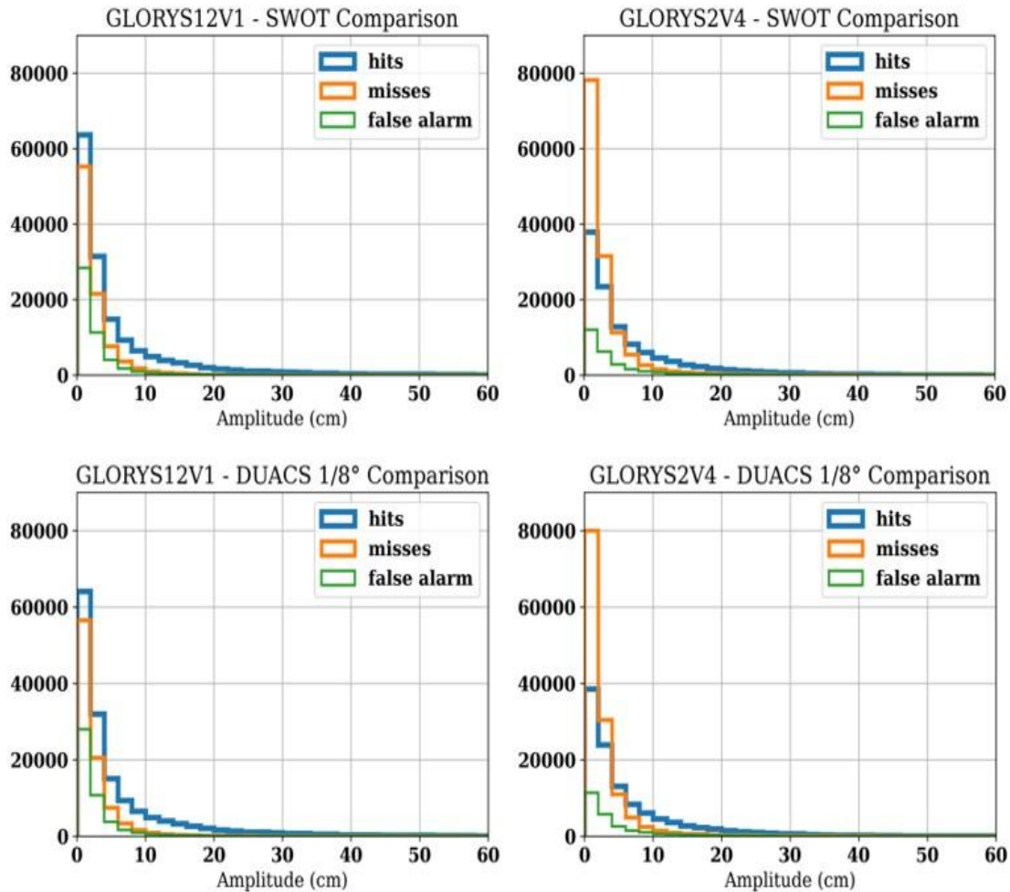
Fig.9. On the top: eddy matching histograms for the total number of hits (blue), misses (orange), false alarms (green) for GLORYS12V1 (left) and GLORYS2V4 (right), compiled as a function of amplitude (cm) over the evaluation period, for SWOT comparison. In the bottom: eddy matching histograms compiled as a function of amplitude (cm) over the evaluation period, for comparison with DUACS 1/8°. The amplitude of hits and misses refers to the satellite (reference) eddies, while the amplitude of false alarms refers to those of unmatched eddies, detected in the reanalysis.
