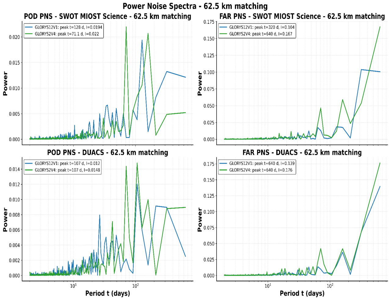
Fig. D2. (a) Time series for the verification metrics, for the comparison with SWOT MIOST Science and DUACS 1/8° comparison, with a minimum lifetime threshold of 4 days. In (b) power spectra for all the time series presented in (a).
