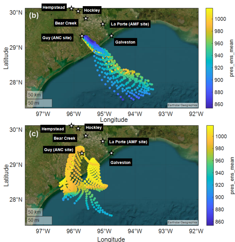
Figure 8 Estimated CCN concentration vertical profiles (a) using TBS measurements for both flights on September 6 at the supersaturations of 0.13%, 0.35%, 0.47%, 0.63%, and 0.8% with ARMTRAJ TBS 24-hour back-trajectories for the TBS flight altitude higher than 1000 m (b) and near ground (c).
