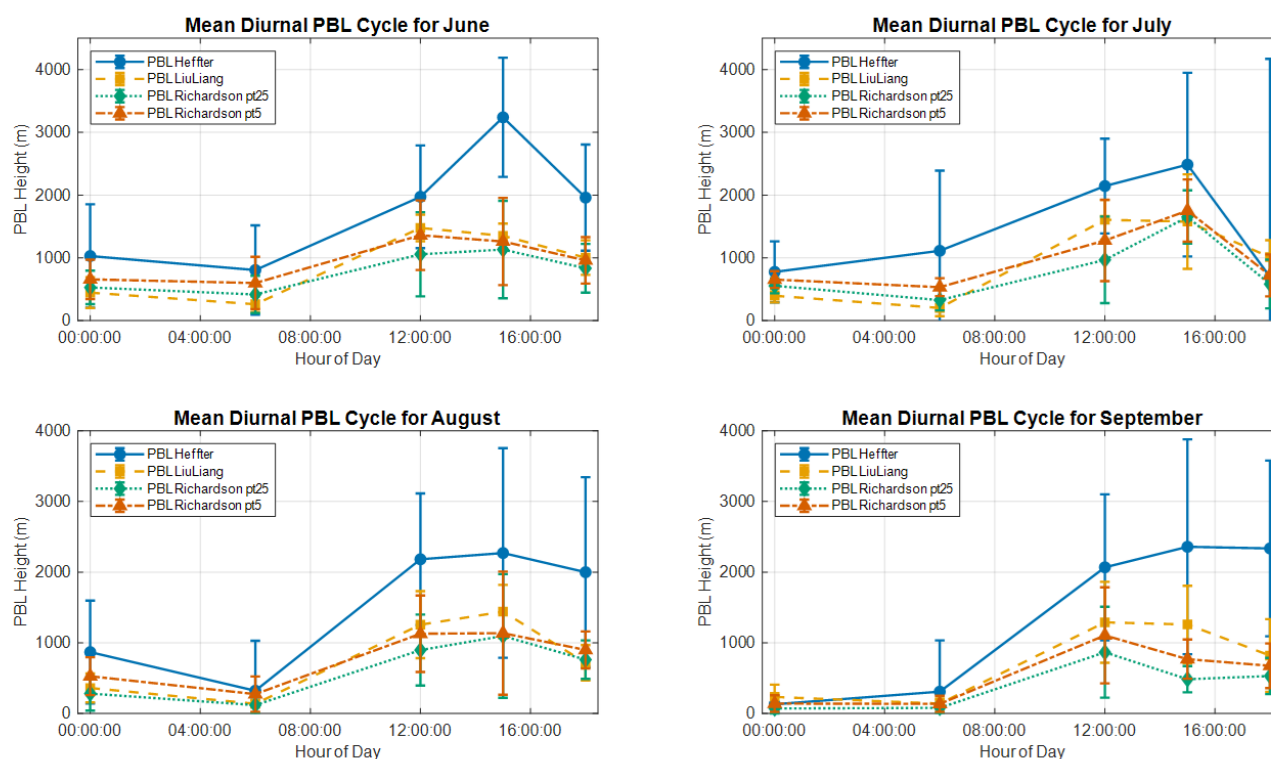
Figure 5. Diurnal variation in UTC time of mean planetary boundary layer (PBL) height for June (1–14), July (2–14), August (2–14), and September (2–14) 2022. Dots indicate the mean PBL height at each sampling time; error bars show the standard deviation of PBL height during each sampling period.
