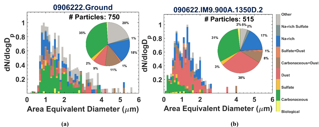
Figure 9 Size-resolved particle classifications from CCSEM/EDX at (a) ground (750 particles analyzed) and (b) 1350 m altitude (515 particles analyzed) for flight on September 6, 2022. The inset shows the percentage of each CCSEM/EDX-derived particle class.
