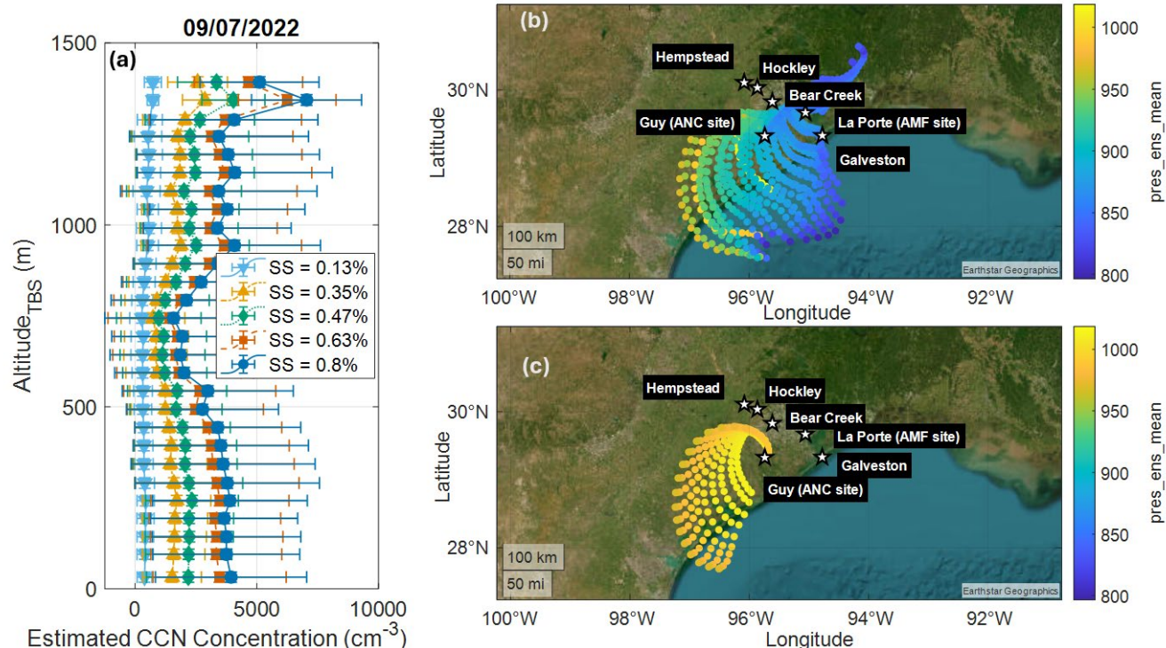
515 Figure 10. Estimated CCN concentration vertical profiles (a) using TBS measurements for all flights on September 7 at the supersaturations of 0.13%, 0.35%, 0.47%, 0.63%, and 0.8% with ARMTRAJ TBS 24-hour back-trajectories for the TBS flight altitude higher than 1000 m (b) and near ground (c).
