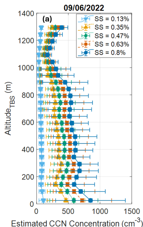
Figure 8 Estimated CCN concentration vertical profiles (a) using TBS measurements for both flights on September 6 at the supersaturations of 0.13%, 0.35%, 0.47%, 0.63%, and 0.8% with ARMTRAJ TBS 24-hour back-trajectories for the TBS flight altitude higher than 1000 m (b) and near ground (c).
