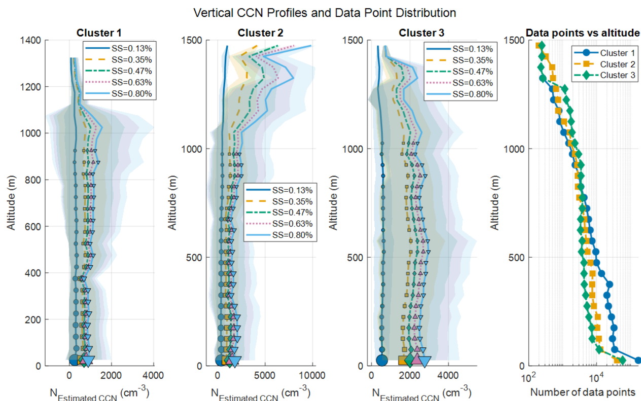
Figure 7. Estimated CCN concentration vertical profiles as a function of TBS altitude for each cluster (a - c), with the number of data points collected at the corresponding altitude for three clusters (d).
