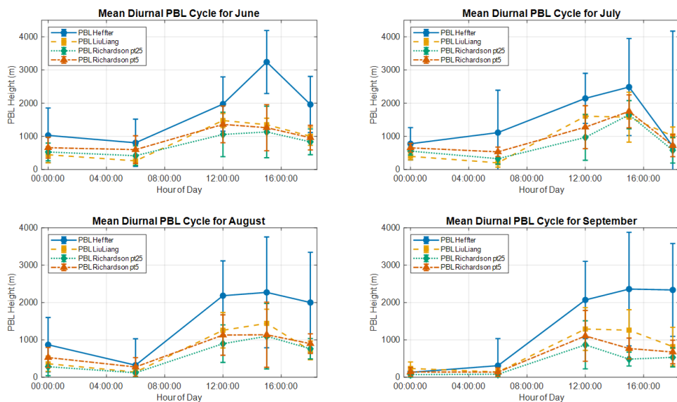
Figure 54. Diurnal variation in UTC time of mean planetary boundary layer (PBL) height for June (1–14), July (2–14), August (2–14), and September (2–14) 2022. Dots indicate the mean PBL height at each sampling time; error bars show the standard deviation of PBL height during each sampling period.
