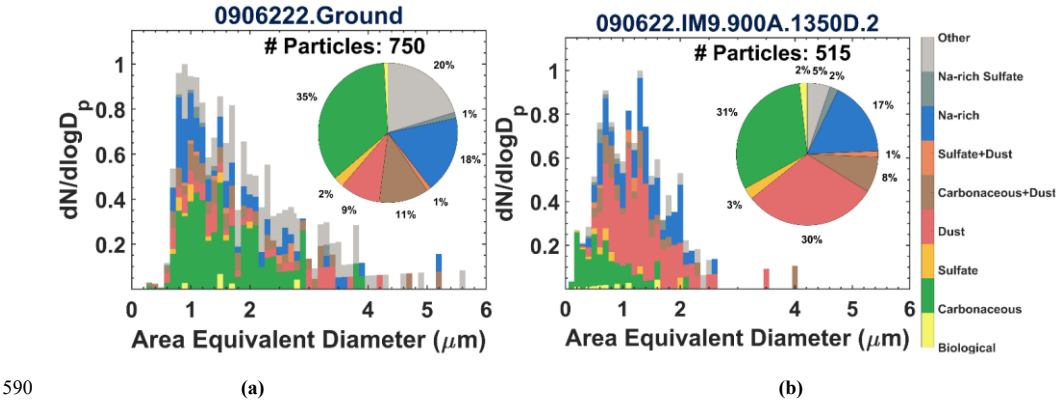
Figure 9 Size-resolved particle classifications from CCSEM/EDX at (a) ground (750 particles analyzed) and (b) 1350 m altitude (515 particles analyzed) for flight on September 6, 2022. The inset shows the percentage of each CCSEM/EDX-derived particle class.
