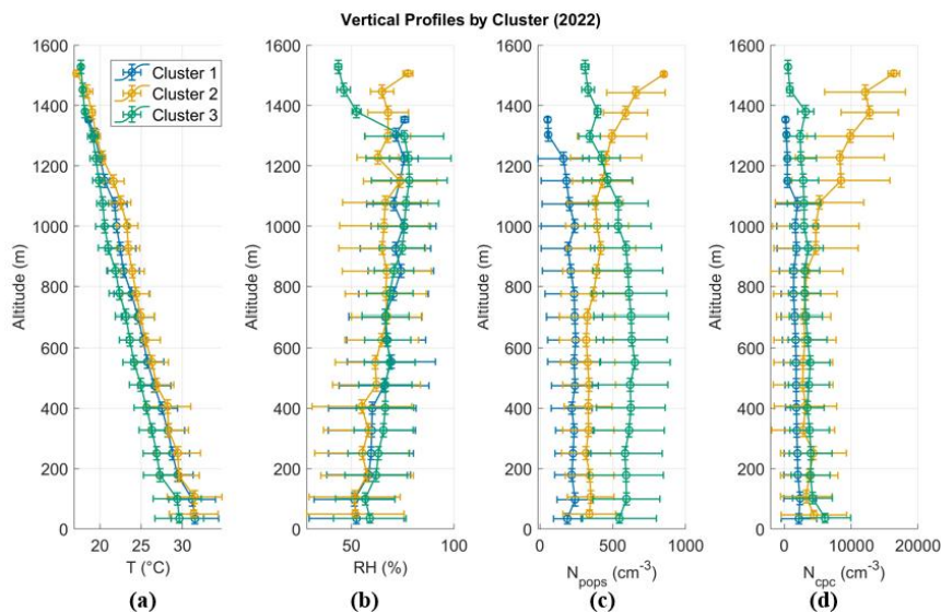
Figure 46. Atmospheric conditions observed during various cluster-influenced flights in the 2022 TRACER campaign. The subplots include: (a) ambient temperature; (b) ambient relative humidity; (c) total particle concentration measured by the portable optical particle spectrometer (POPS, particles ranging from 135 to 3,000 nm) total-particle concentration measured by the condensation particle counter (CPC, particles greater than 10 nm); and (d)total particle concentration measured by the condensation particle counter (CPC, particles greater than 10 nm)–total-particle concentration measured by the portable optical particle spectrometer (POPS, particles ranging from 135 to 3,000 nm). The square symbols represent the averaged mean values of the sampling periods, while the error bars denote the standard deviation of the measurements.
