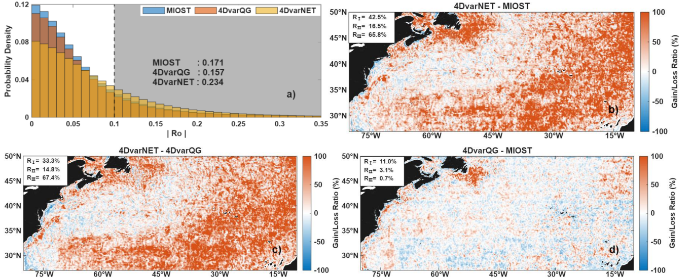
320 Figure 7: (a) PDFs of the absolute Rossby number |R_o| for the three L4 products. Mean |R_o| values are annotated. (b–d) Spatial distributions of the |R_o| gain/loss ratio between pairs of products. Warm colors indicate regions where the first-listed product exhibits larger |R_o| relative to the reference product, while cold colors indicate regions where it exhibits smaller |R_o| . Insets report region-averaged gain/loss ratios ( R ) over the three predefined dynamical regimes.
