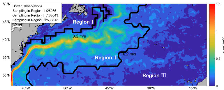
205 Figure 2: Mean surface velocity and dynamic regime partition derived from DUACS geostrophic velocity fields over 27 July 2023–20 April 2024. Black contours delineate the boundaries of the three dynamic regimes, broadly following the 0.2 \text{ m/s} speed contour. Moderate spatial smoothing was applied to ensure coherent regime boundaries. The number of drifter samples within each regime is annotated in the upper-left corner.
