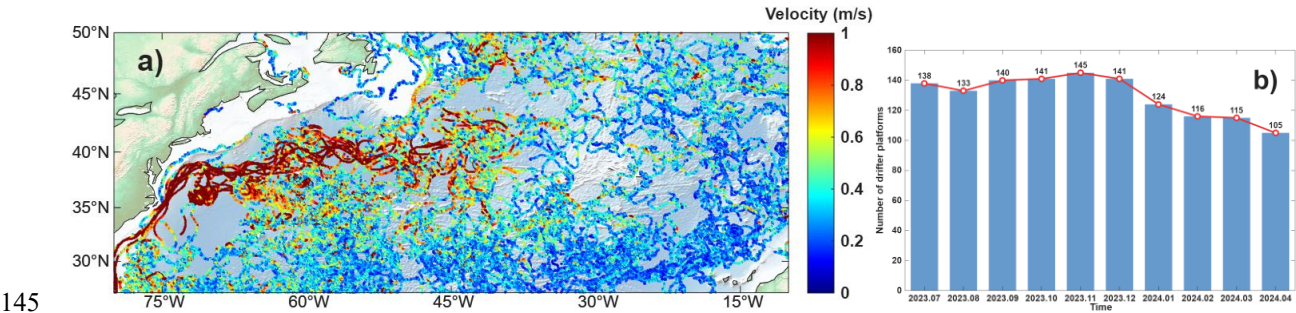
Figure 1: (a) Study area and spatial distribution of drifter platforms. The background shading represents ocean bathymetry, and the trajectories of the drifters are indicated by lines, with line color representing drifter speed magnitude. (b) Temporal distribution of drifter platforms in the North Atlantic during the study period.
