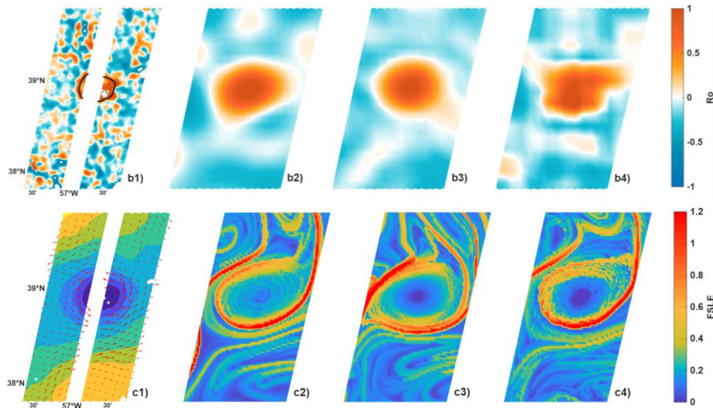
Figure 9: Case 1 (SWOT L3 cycle 002, pass 145; 16 August 2023). Spatial comparison of: (a) sea surface height anomaly (SSHA), (b) Rossby number ( R_o ), (c) Geostrophic current of SWOT L3 (left column) and FSLE derived from three L4 products (MIOST, 4DvarQG, 4DvarNET). White crosses mark SWOT-identified eddy cores; colored crosses indicate reconstructed cores from each product. Note that R_o color scales differ to account for sharper gradients and higher amplitudes in SWOT L3 relative to L4 reconstructions.
