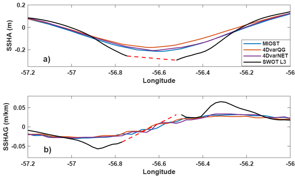
Figure 10: Cross-sectional comparison of SSHA and its along-track gradient across the eddy core in Case 1 (section indicated in Figure 8a1). (a) SSHA profiles and (b) corresponding SSHA gradients from SWOT L3 and L4 products. Differences in amplitude and gradient sharpness highlight the products' varying ability to reconstruct eddy intensity and frontal structure.
