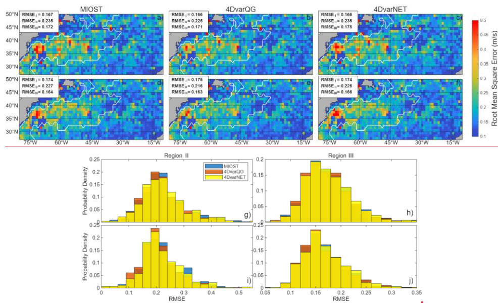
Figure 33: (a-f) The RMSE of L4 products computed on 1^{\circ} \times 1^{\circ} grids. Columns correspond to different L4 products, and rows correspond to meridional (top) and zonal (bottom) velocity components. Region-averaged velocity RMSE within each dynamic regime are indicated in the upper-left annotation of each panel. (g-j) PDFs of the RMSE in Regions II and III, for zonal and meridional velocity components.
