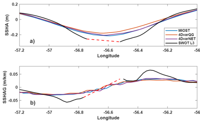
Figure 10: Cross-sectional comparison of SSH and its along-track gradient across the eddy core in Case 1 (section indicated in Figure 8a1). (a) SSH profiles and (b) corresponding SSH gradients from SWOT L3 and L4 products. Differences in amplitude and gradient sharpness highlight the products' varying ability to reconstruct eddy intensity and frontal structure.
