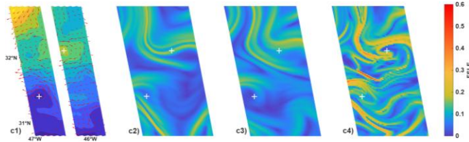
Figure 13: Case 3 (SWOT L3 cycle 001, pass 324; 1 August 2023), presented with the same layout and diagnostics as Figure 8.
