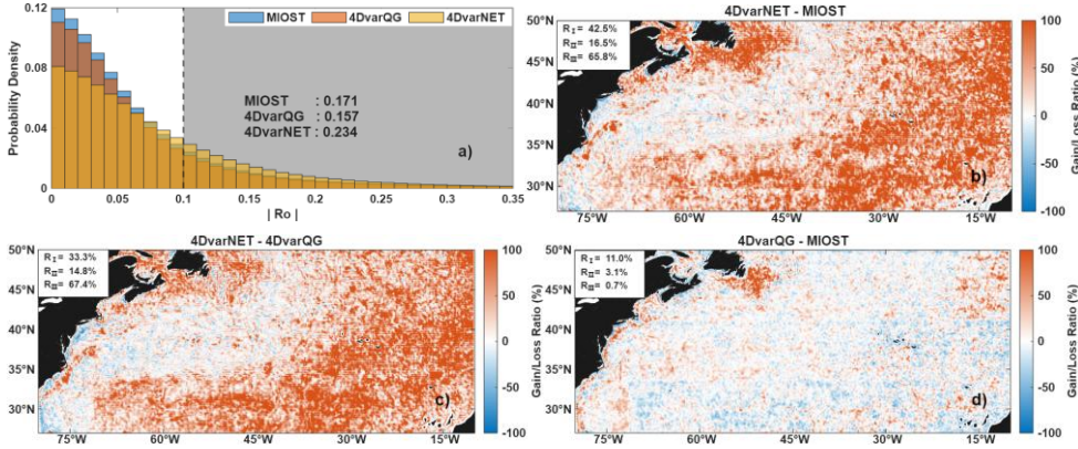
Figure 7: (a) PDFs of the absolute Rossby number |R_o| for the three L4 products. Mean |R_o| values are annotated. (b–d) Spatial distributions of the |R_o| gain/loss ratio between pairs of products. Warm colors indicate regions where the first-listed product exhibits larger |R_o| relative to the reference product, while cold colors indicate regions where it exhibits smaller |R_o| . Insets report region-averaged gain/loss ratios ( R ) over the three predefined dynamical regimes.
