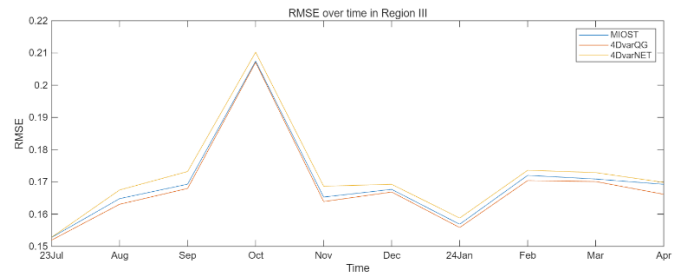
R 2. Temporal variation curves of RMSE for three products across different regions
