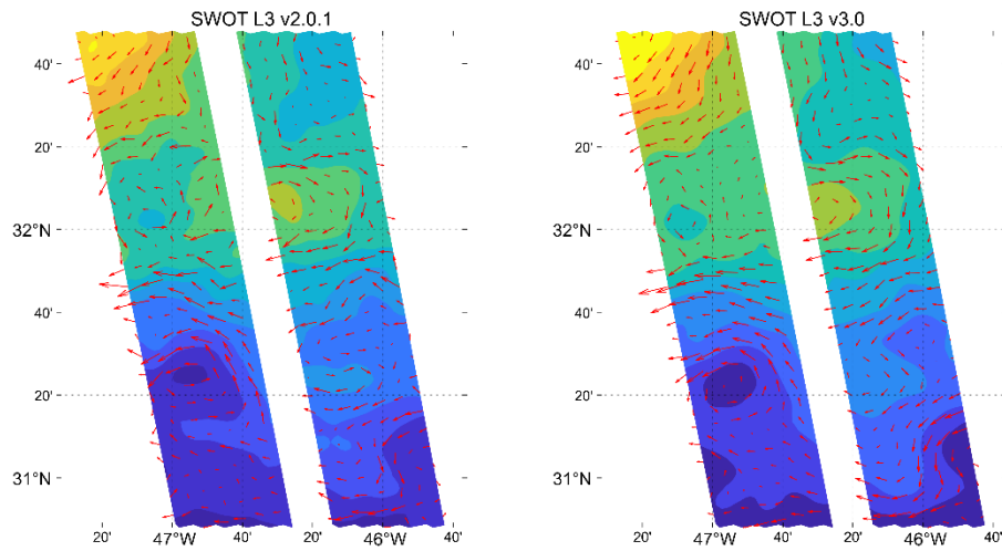
R 1. Comparison of SSHA and geostrophic current fields between different SWOT L3 versions in case 3 (left: v2.0.1; right: v3.0)
