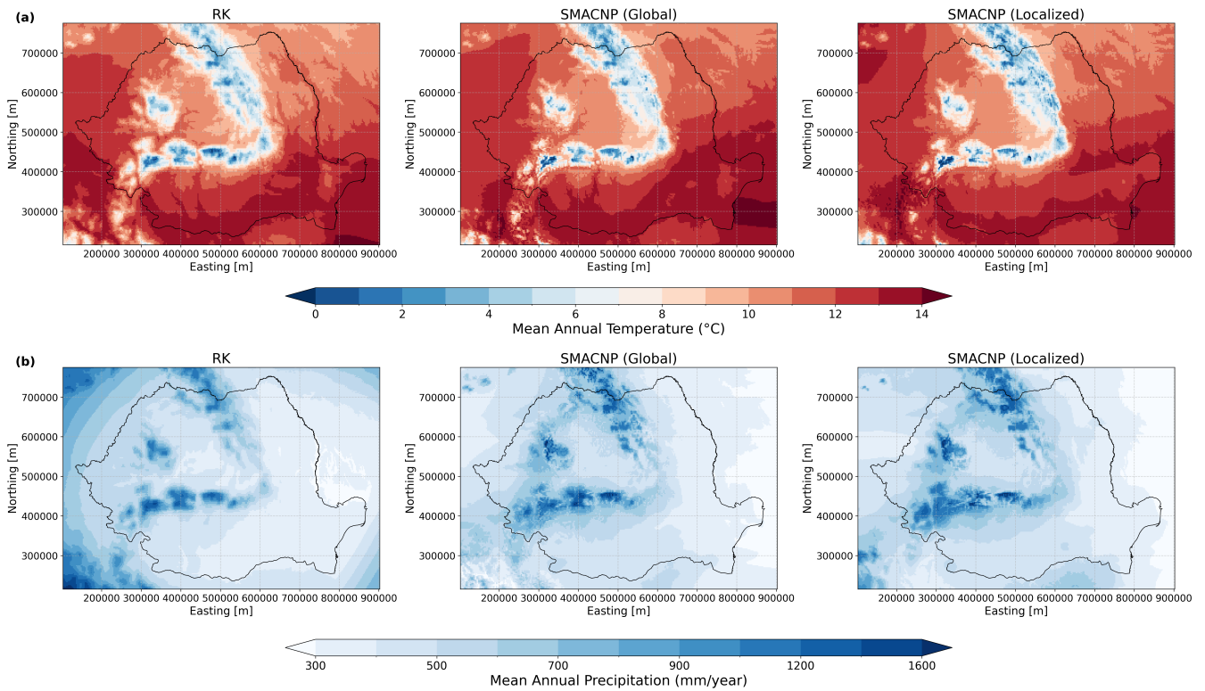
270 Figure 5 Comparison of predicted mean annual temperature (a) and precipitation (b) from three models: RK, SMACNP (Global), and SMACNP (Localized).
