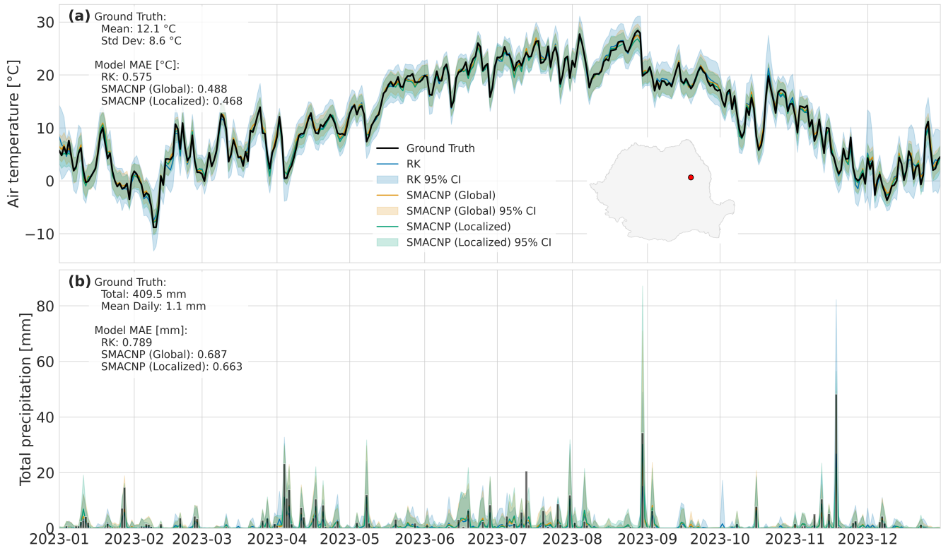
Figure 8 Model performance and uncertainty at Bacău station (428 m a.m.s.l.). Time series comparison of (a) daily average temperature and (b) daily total precipitation for the year 2023. Shaded areas represent the 95% confidence interval for each model's prediction. The inset map shows the location of the station within the study area, marked by a red dot.
